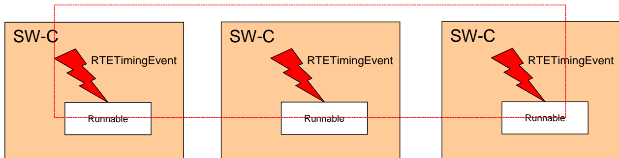
synchronization of runnable triggering
