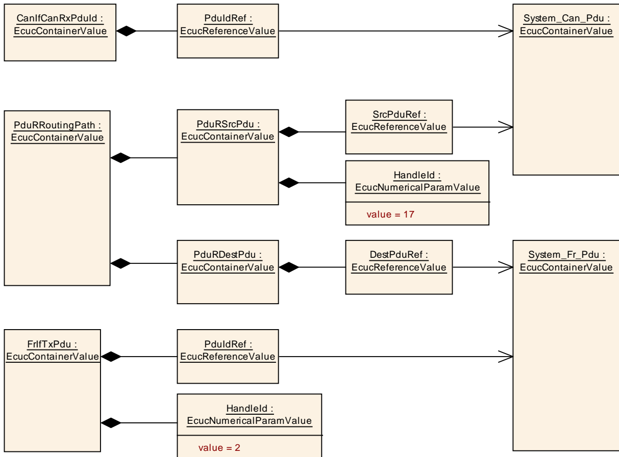
Figure 3.15: Gateway from CanIf to FrIf example
