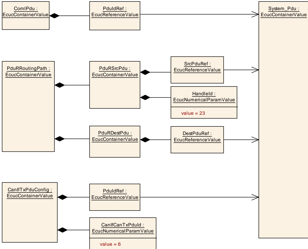
Figure 3.13: Tx from Com to CanIf example
