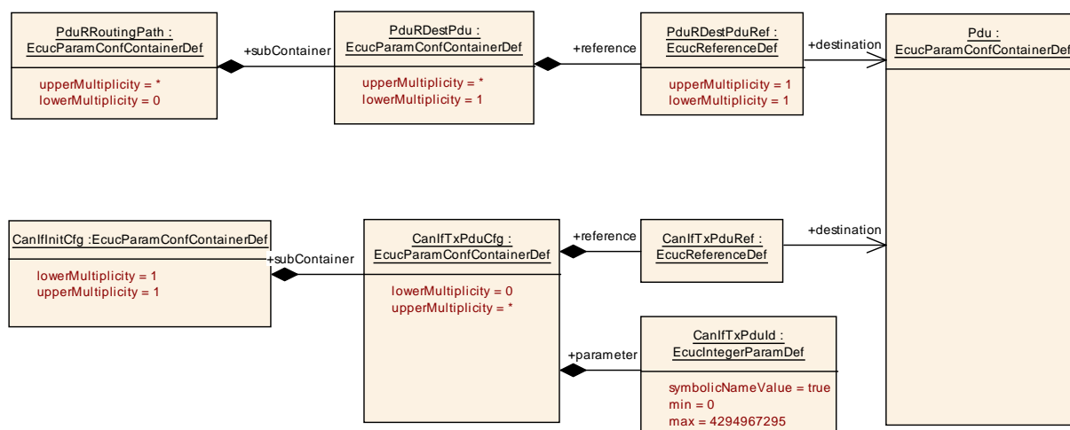
Figure 3.12: Transmission from PduR to CanIf
