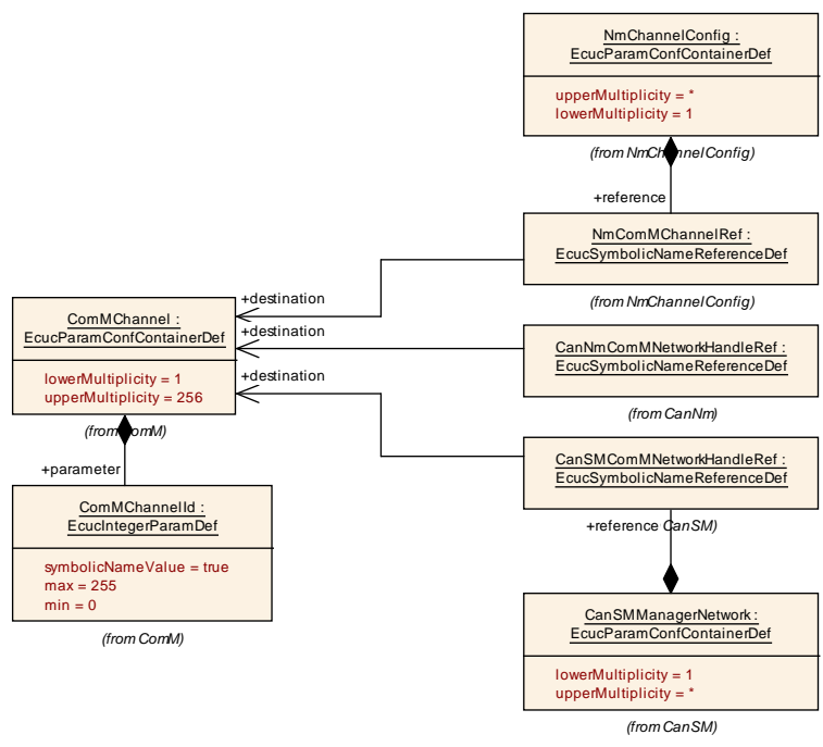
Figure 3.16: Example of Channel interaction between ComM, Can and Nm
