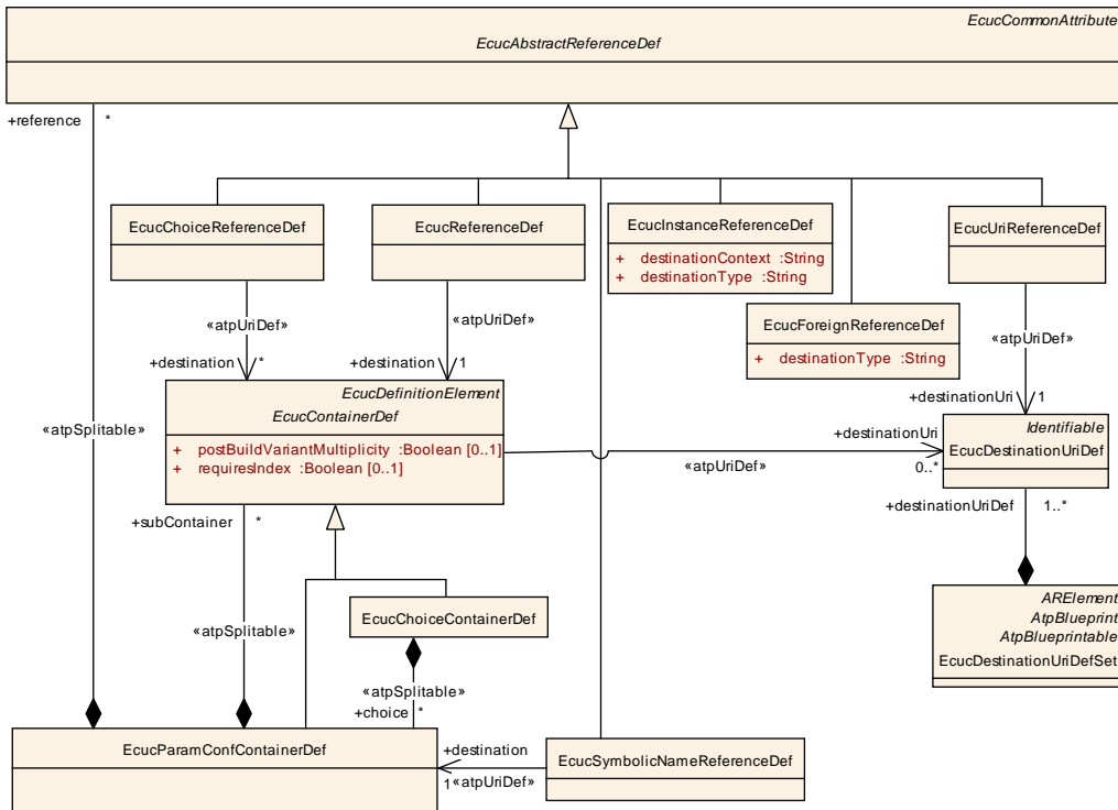
Figure 2.11: Class diagram for parameter references
