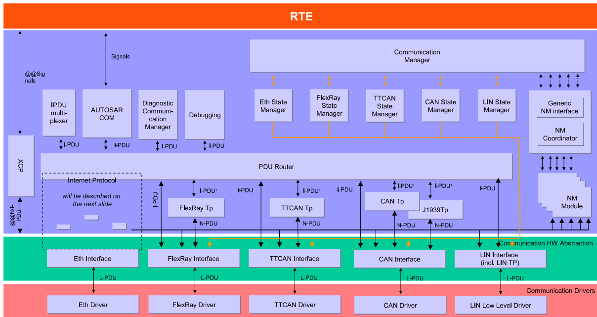
Figure 3.10: Interfaces in the COM-Stack [15]
