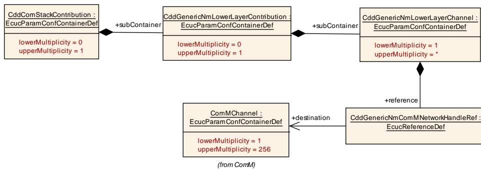
Figure 3.22: GenericNm lower layer contribution
