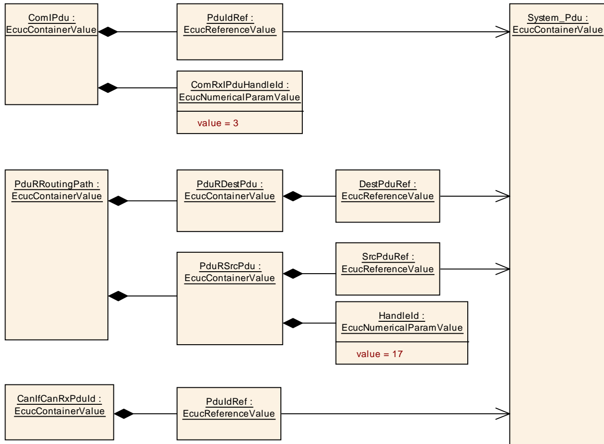
Figure 3.14: Rx from CanIf to Com example
