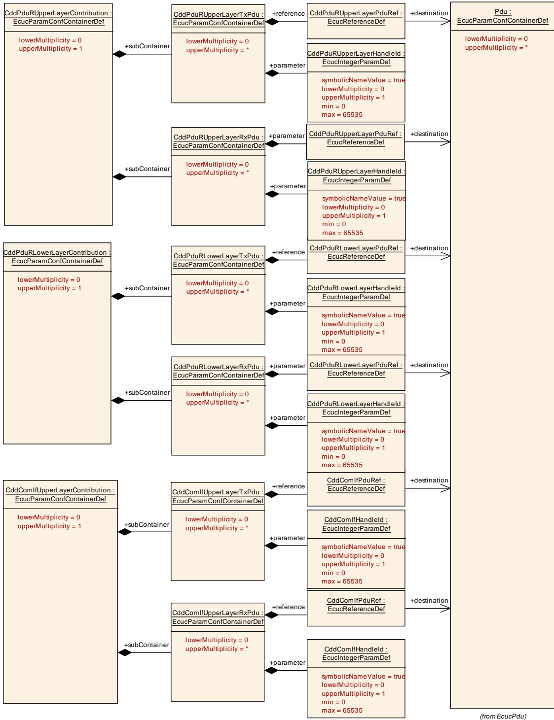
Figure 3.19: PduR and Com Interface contribution
