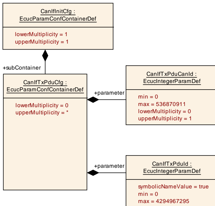
Figure 3.11: Example of Can Interface Tx configuration
