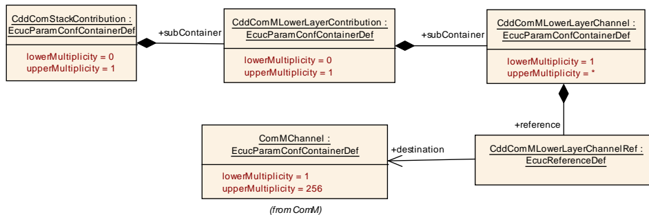
Figure 3.21: ComM lower layer contribution
