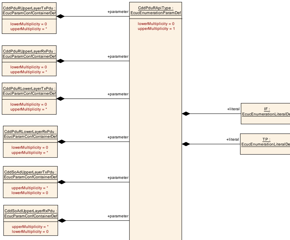
Figure 3.20: Configuration of the CDD interface API type
