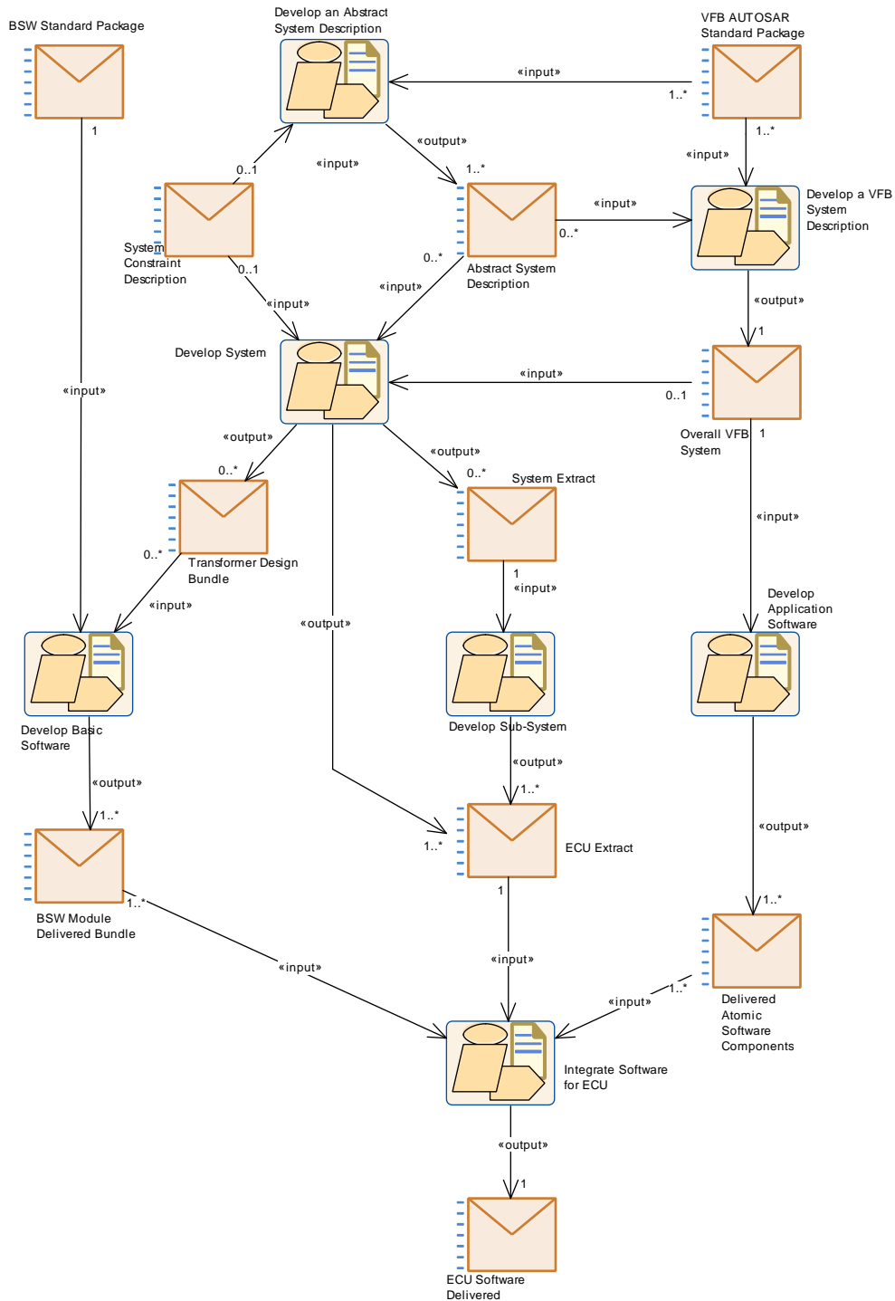
Figure 1.1: AUTOSAR Methodology Overview (from [1])
