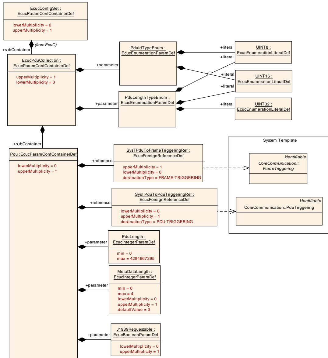
Figure 3.9: Generic Pdu Container
