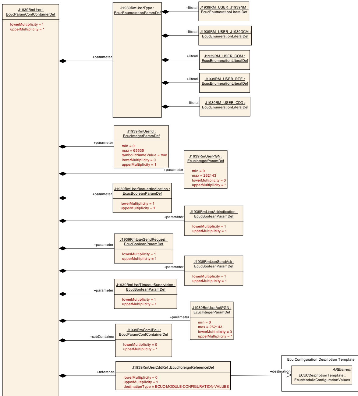
Figure 13: Configuration container J1939RmUser
