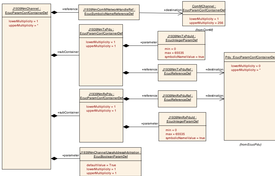
Figure 7: Configuration container J1939NmChannel
