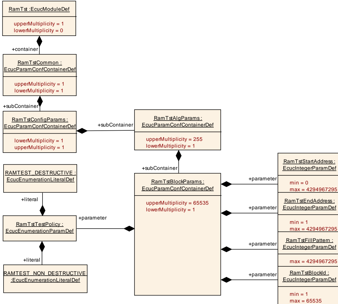
Figure 20: RamTstBlockParams
