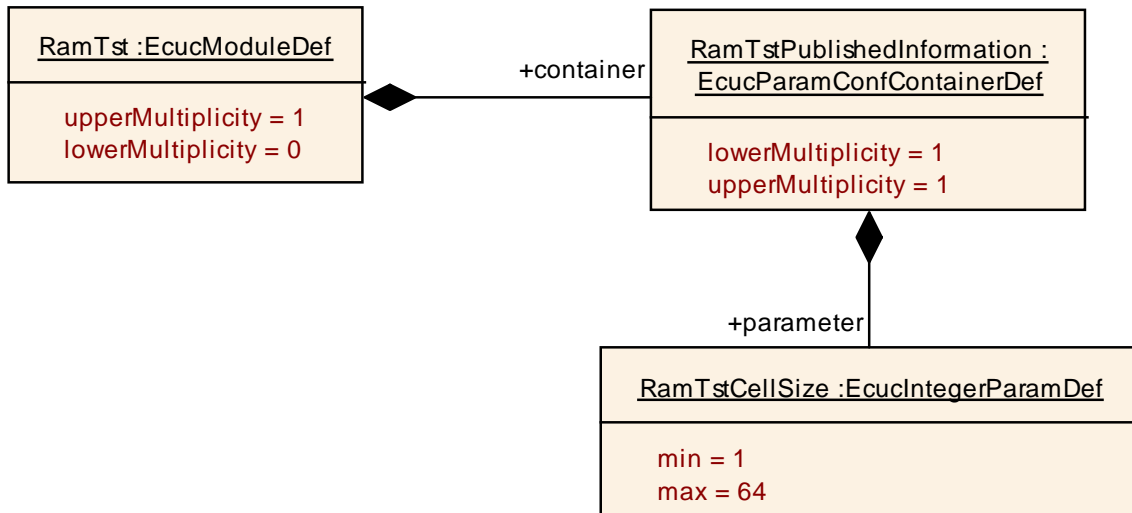
Figure 21: RamTstPublishedInformation
