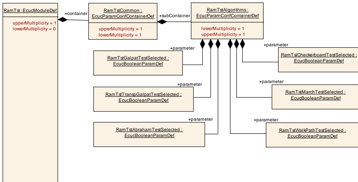
Figure 17: RamTstAlgorithms
