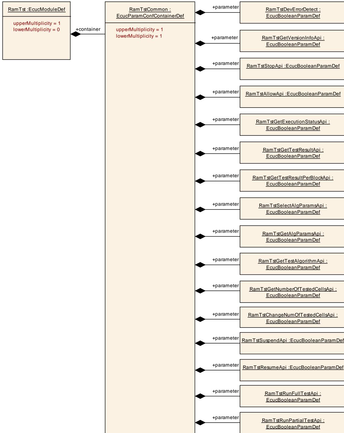
Figure 16: RamTstCommon
