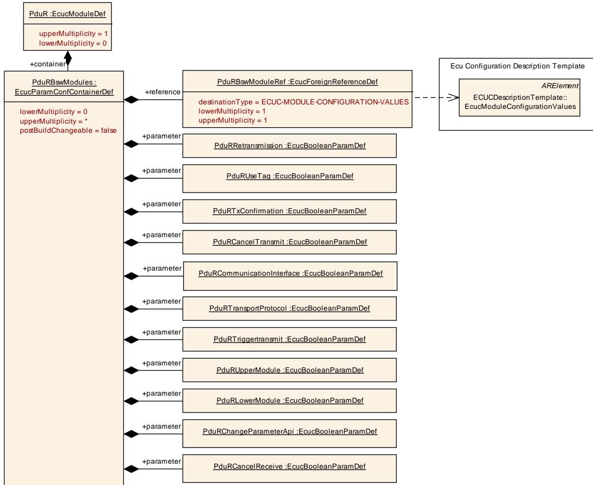
Figure 24 - PduRBSwModules
