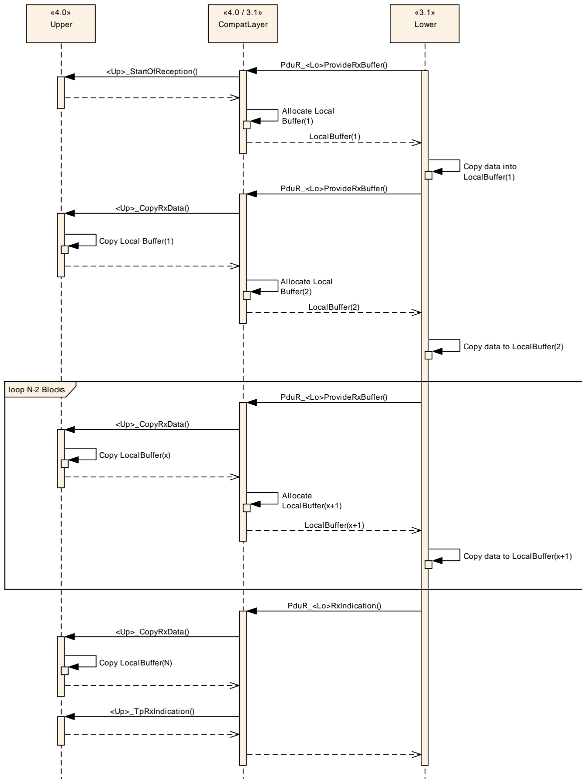
Figure 28 - Reception-Lower3.1-Upper4.0
