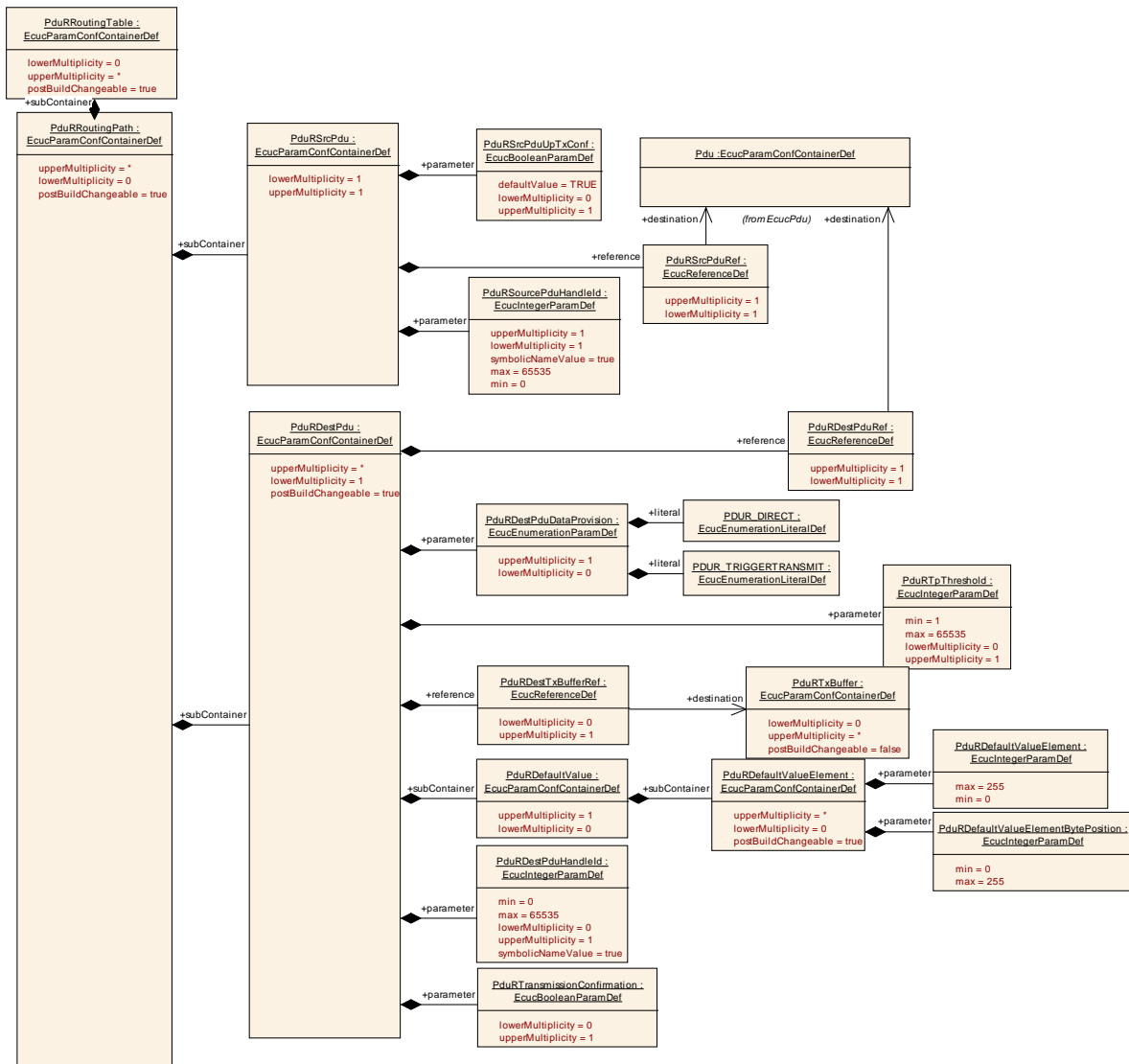
Figure 27 - PduRRoutingPath
