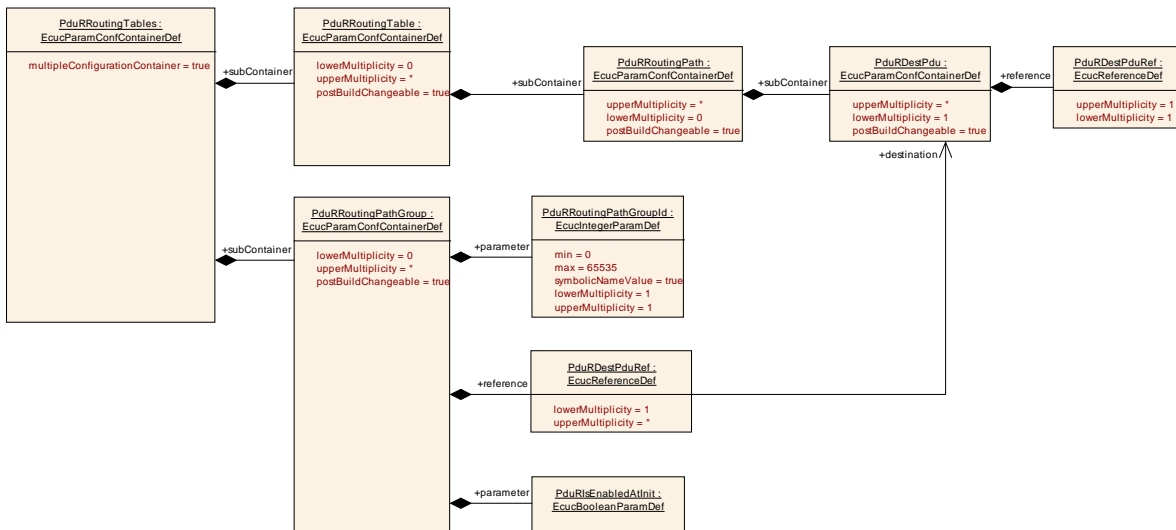
Figure 26 - PduRRoutingPathGroup
