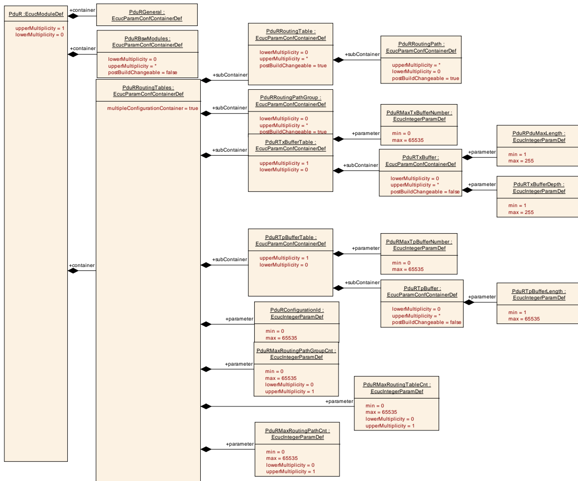
Figure 23: PDU Router Configuration Overview - PduR
