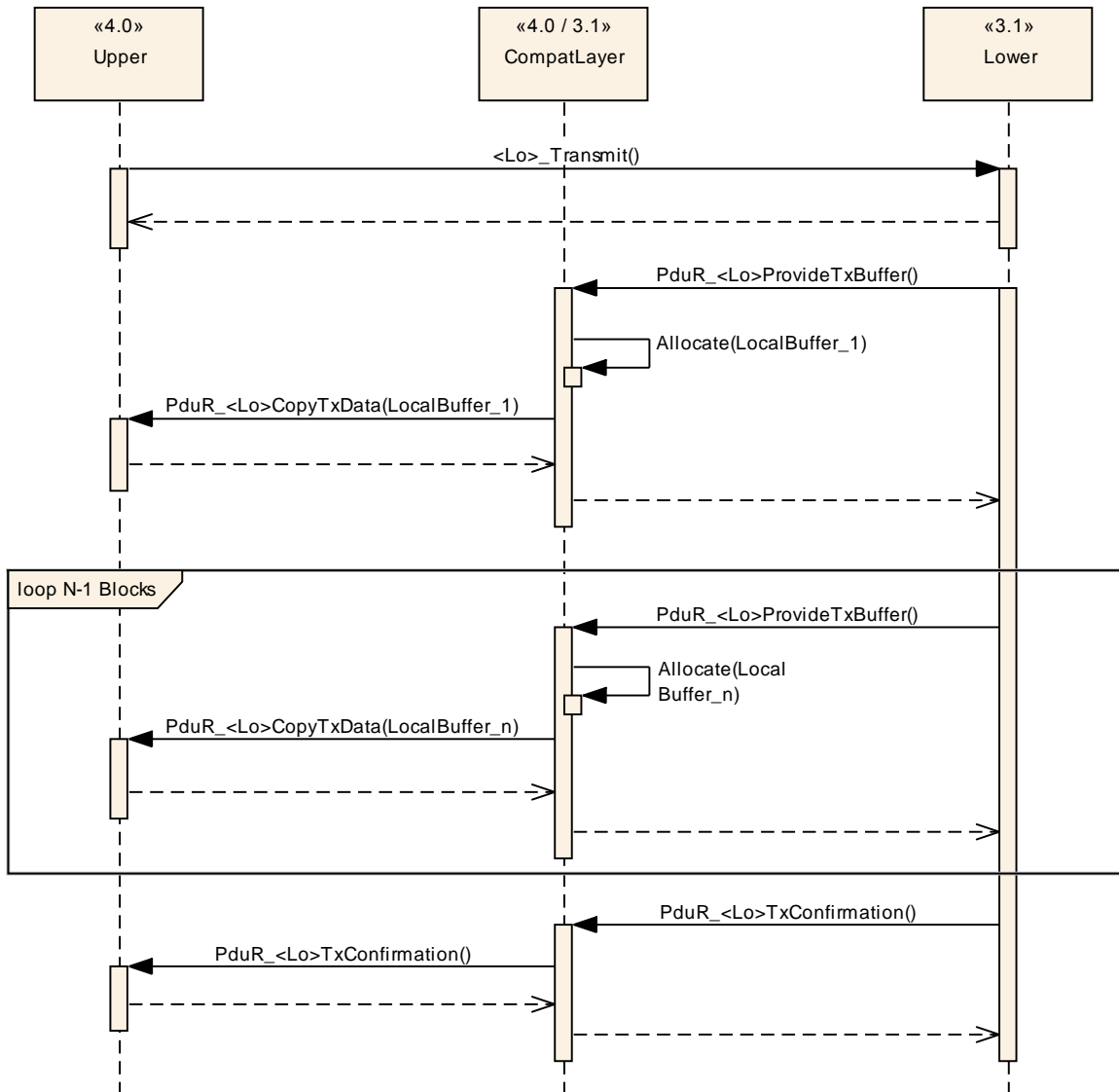
Figure 29 - Transmission-Upper4.0-Lower3.1
