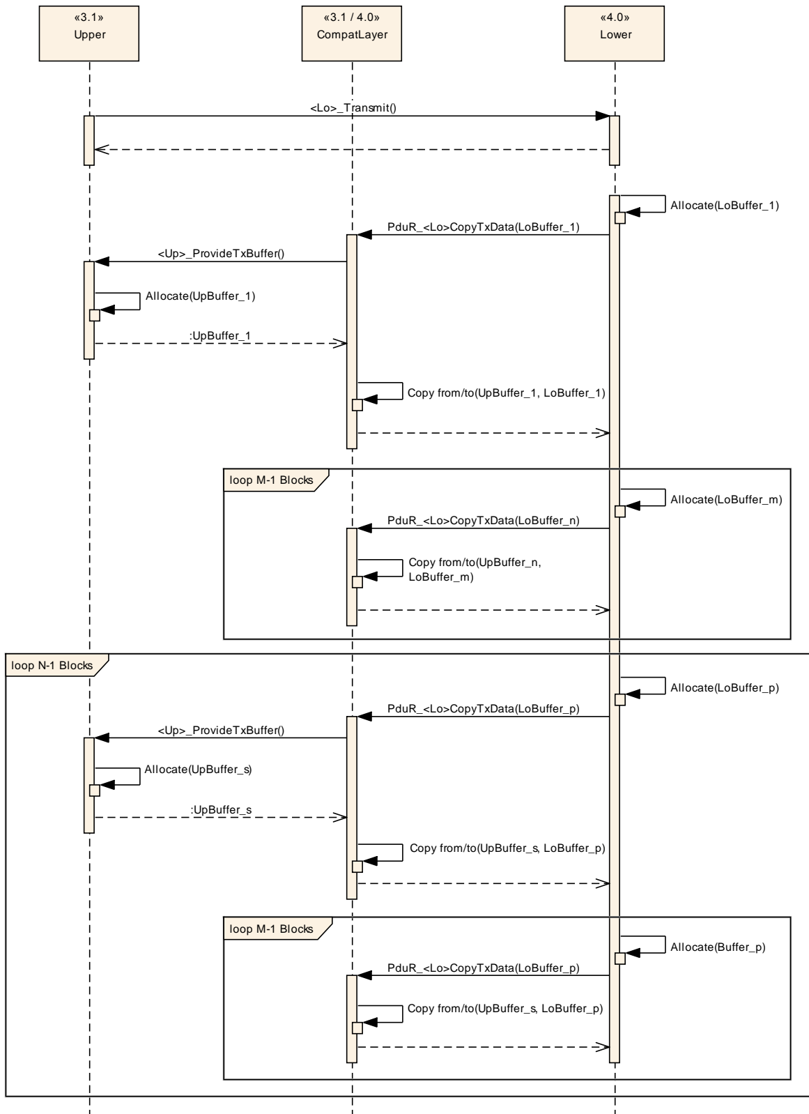
Figure 31 - Transmission-Upper3.1-Lower4.0
