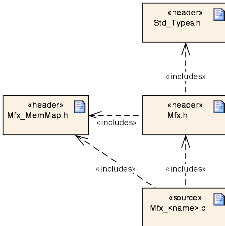
Figure 1: File structure
