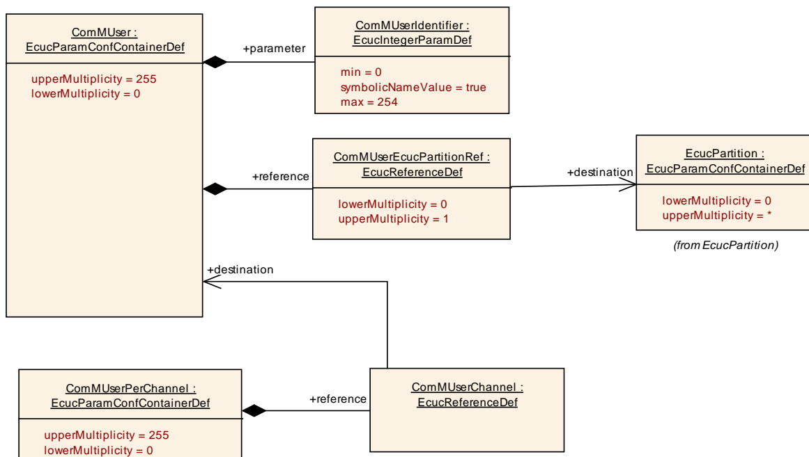
Figure 15: Configuration ComMUser
