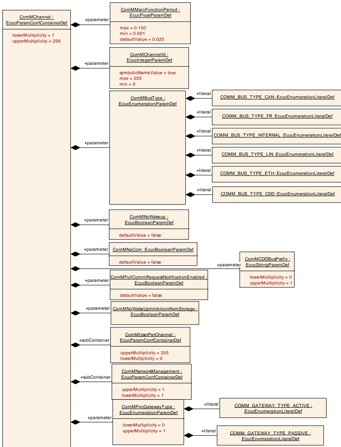
Figure 16: Configuration ComMChannel
