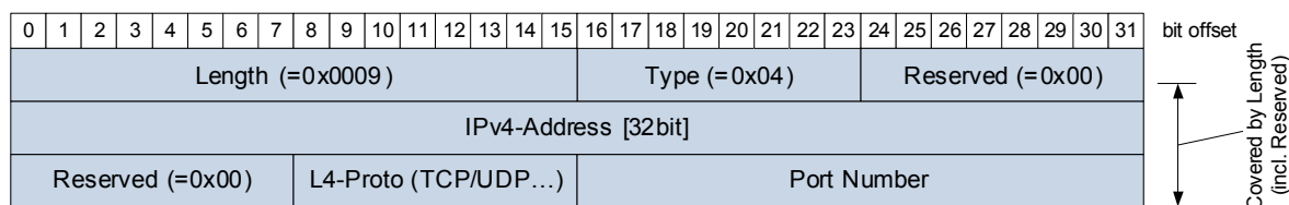
Figure 6.16: SOME/IP-SD IPv4 Endpoint Option
