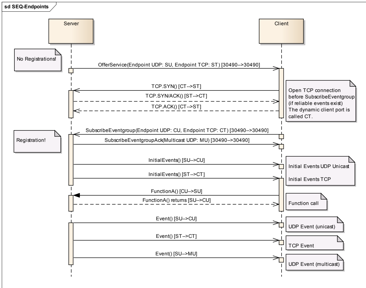
Figure 6.34: Publish/Subscribe Example for Endpoint Options and the usage of ports
