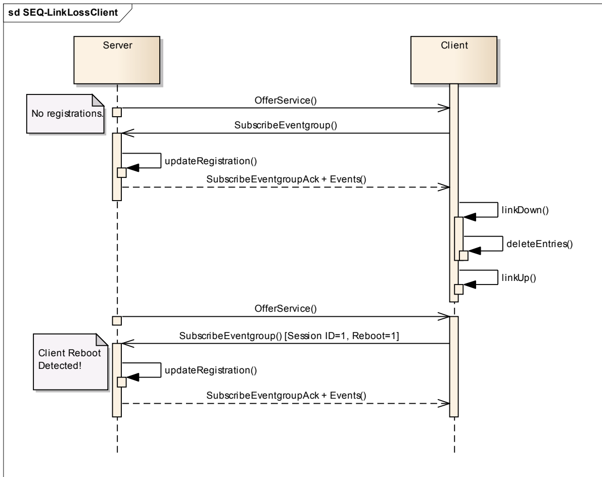
Figure 6.27: Publish/Subscribe with link loss at client (figure ignoring timings)
