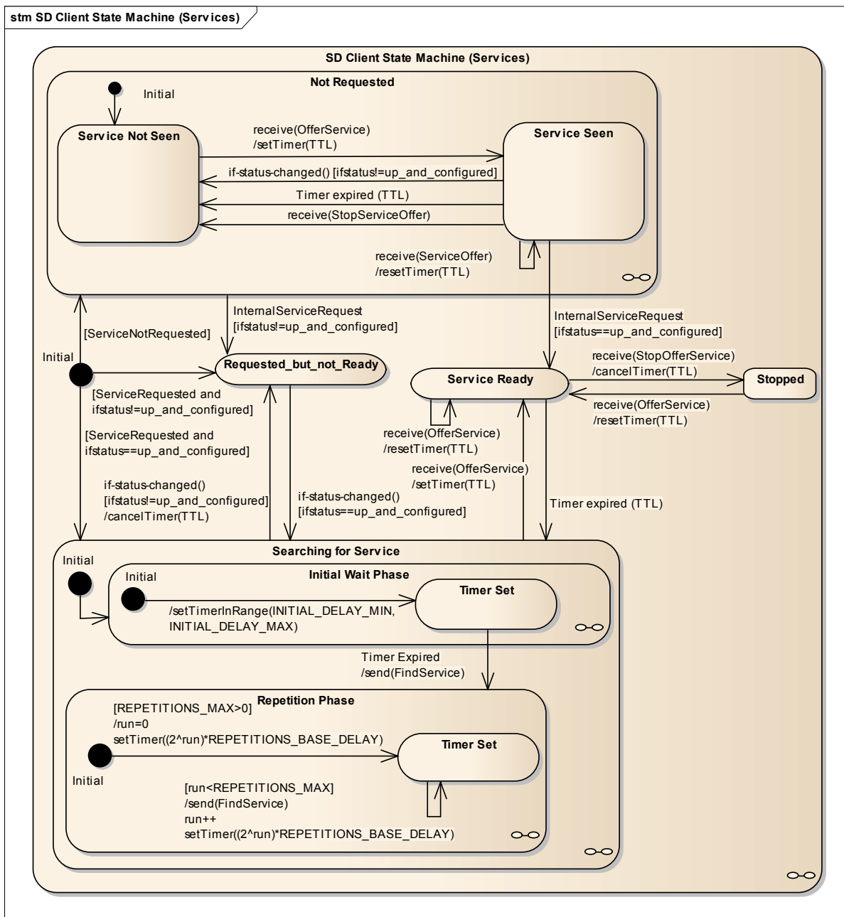
Figure 6.24: SOME/IP Service State Machine Client
