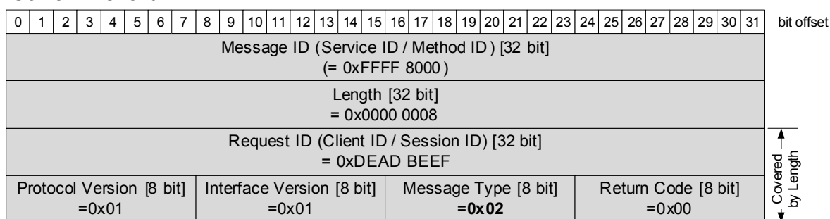
Figure 6.7: SOME/IP Magic Cookie Message for SOME/IP
