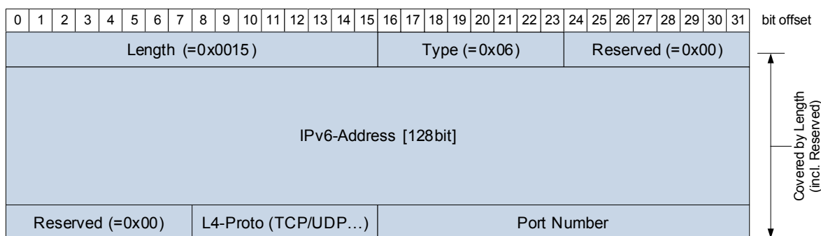
Figure 6.17: SOME/IP-SD IPv6 Endpoint Option
