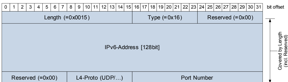
Figure 6.19: SOME/IP-SD IPv6 Multicast Option
