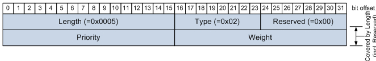
Figure 6.15: SOME/IP-SD Load Balancing Option
