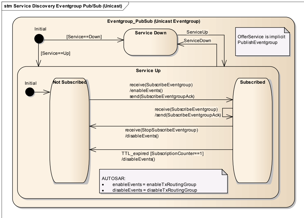
Figure 6.30: Publish/Subscribe State Diagram (server behavior for unicast eventgroups)
