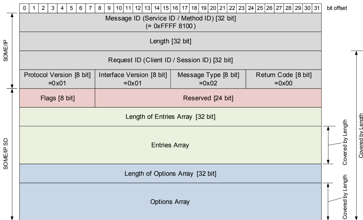
Figure 6.10: SOME/IP-SD Header Format
