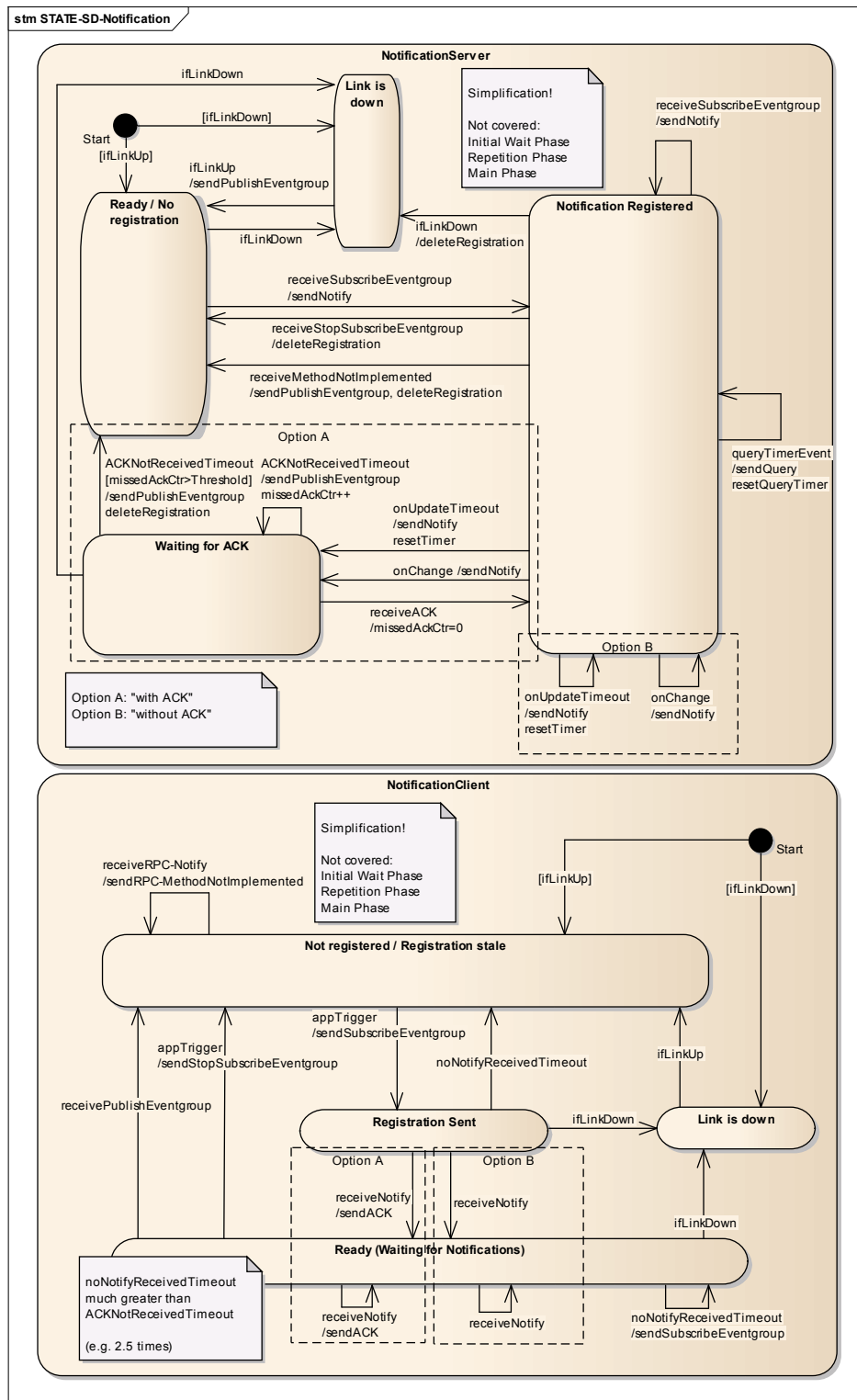
Figure 6.33: Publish/Subscribe State Diagram (overall behavior)
