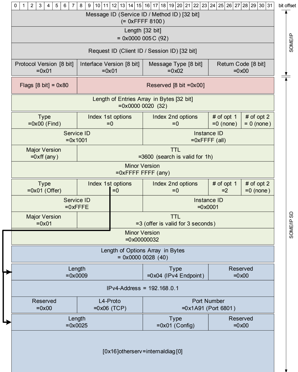
Figure 6.25: SOME/IP-SD Example PDU for Non-SOME/IP-SD
