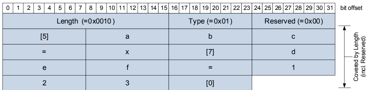
Figure 6.14: SOME/IP-SD Configuration Option Example
