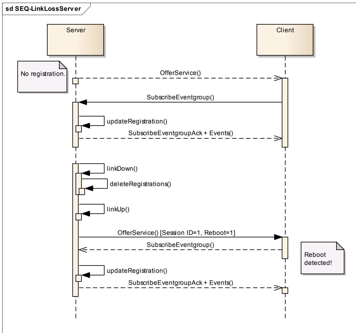
Figure 6.29: Publish/Subscribe with link loss at server (figure ignoring timings)
