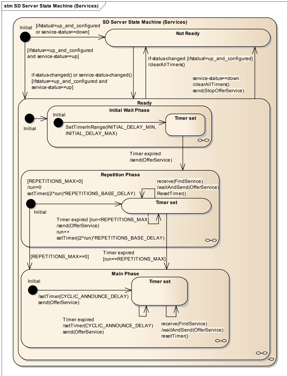
Figure 6.23: SOME/IP Service State Machine Server
