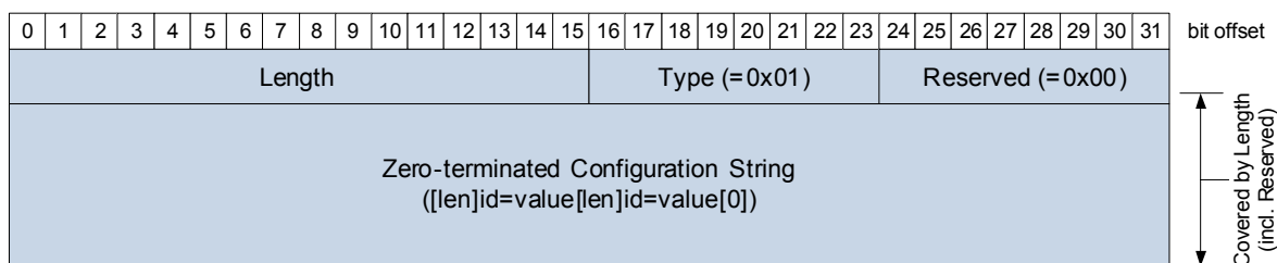
Figure 6.13: SOME/IP-SD Configuration Option
