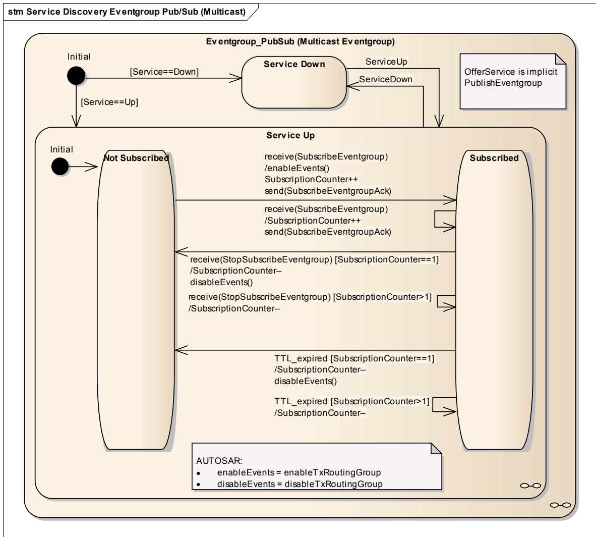
Figure 6.31: Publish/Subscribe State Diagram (server behavior for multicast event-groups)
