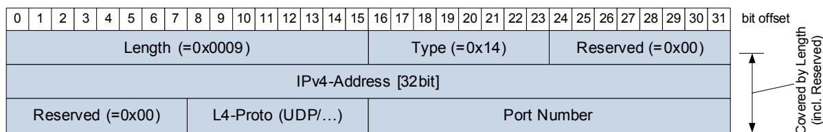
Figure 6.18: SOME/IP-SD IPv4 Multicast Option
