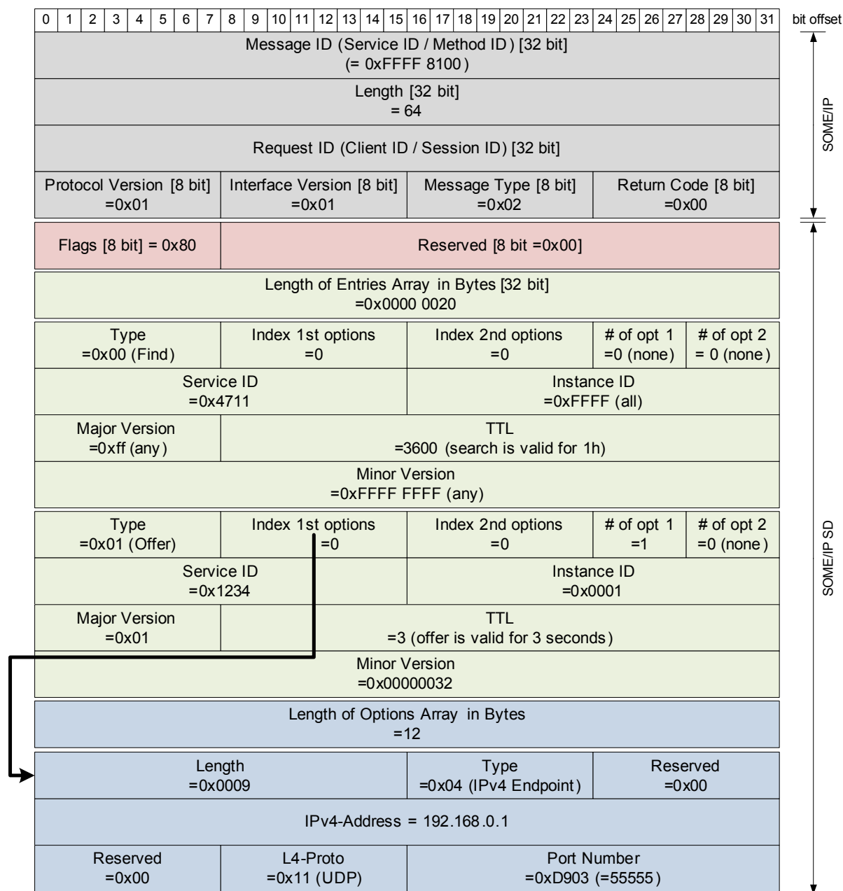
Figure 6.22: SOME/IP-SD Example PDU
