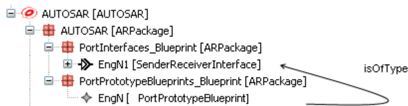
Figure 3 Example AUTOSAR Blueprints EngN
