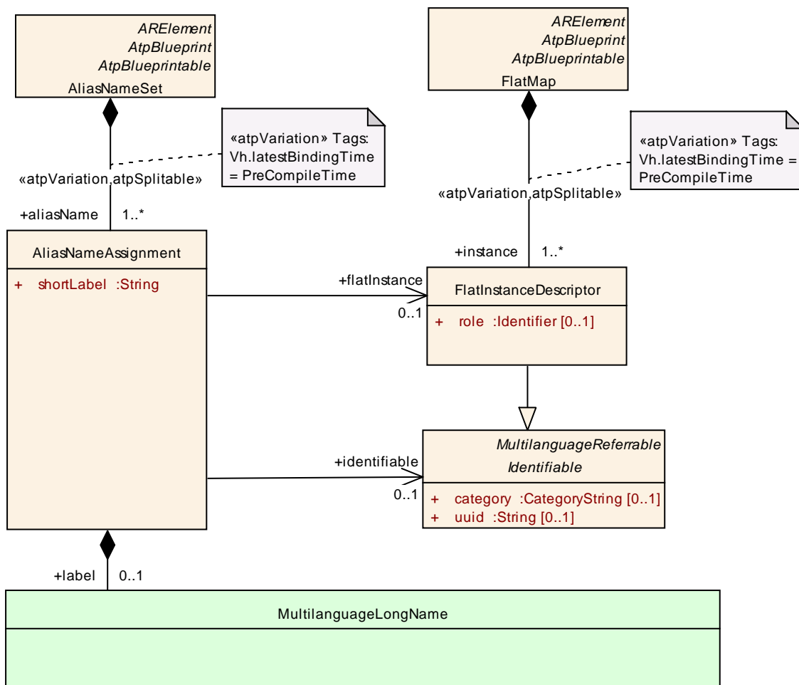
Figure 4 AliasNameAssignment [4]
