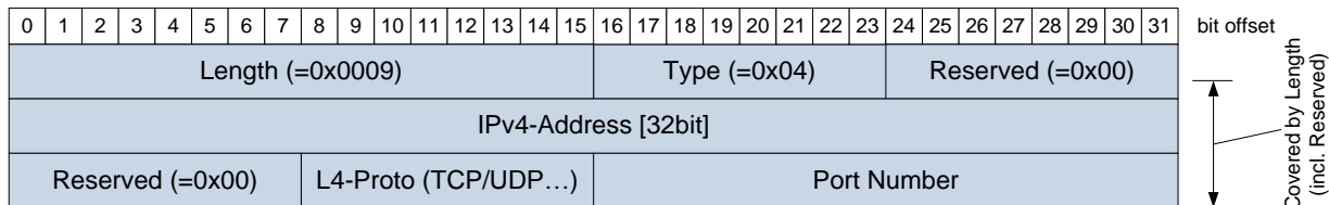
Figure 8 – IPv4 Endpoint Option format
