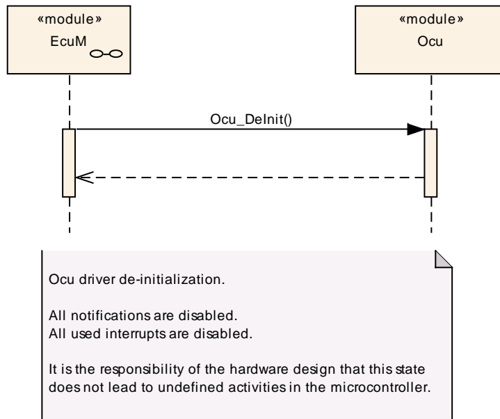
Figure 12: Ocu de-initialization
