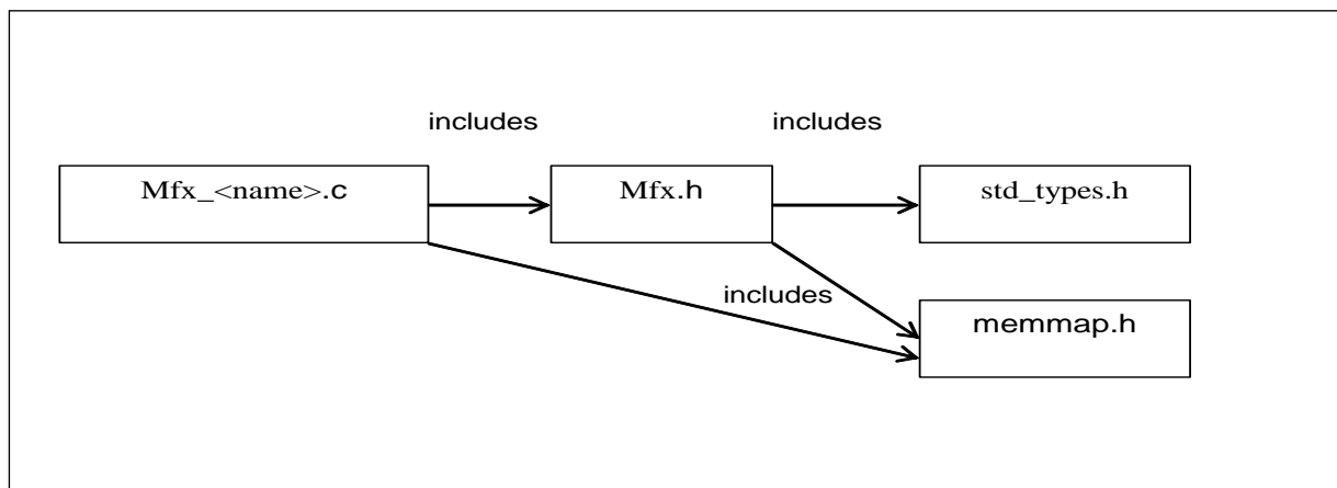
Figure 1: File structure
