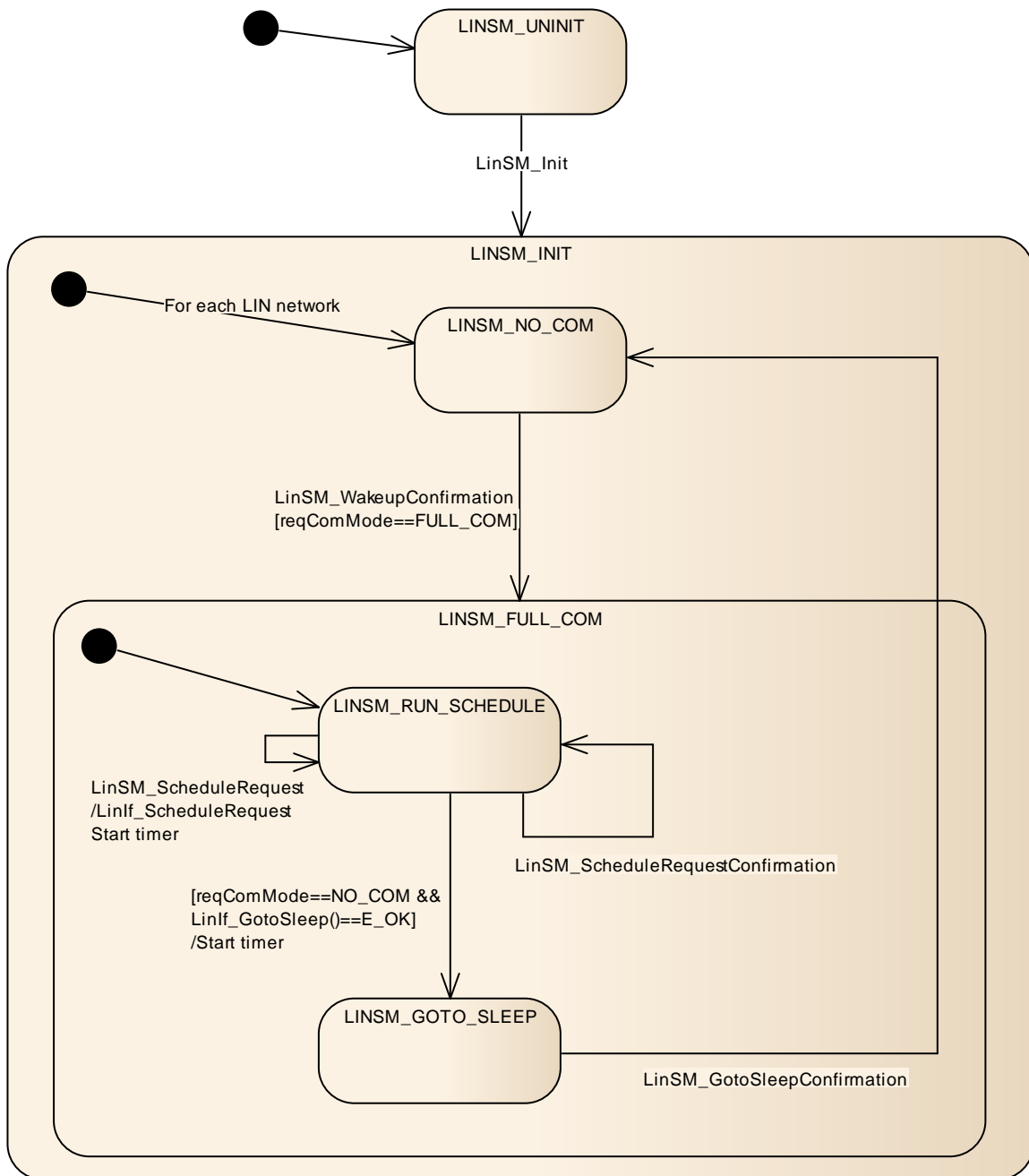
Figure 4: LinSM State Machine
