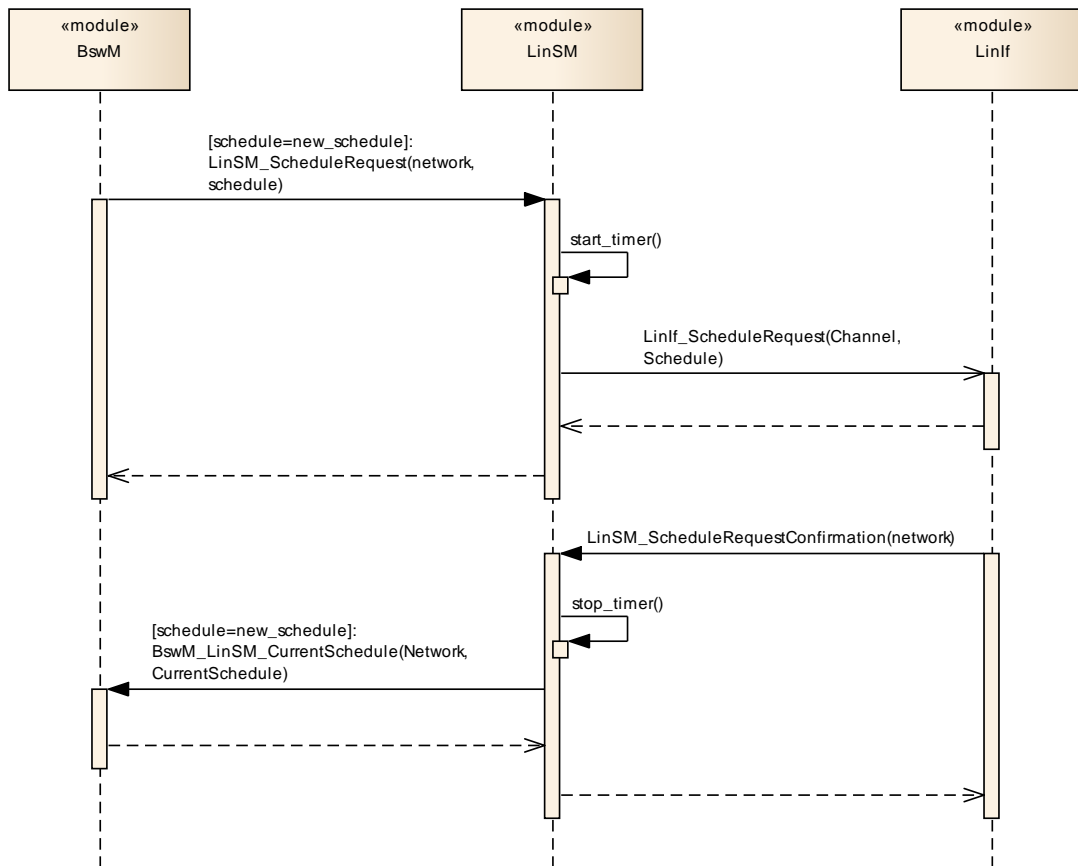
Figure 7: Schedule Table switch
