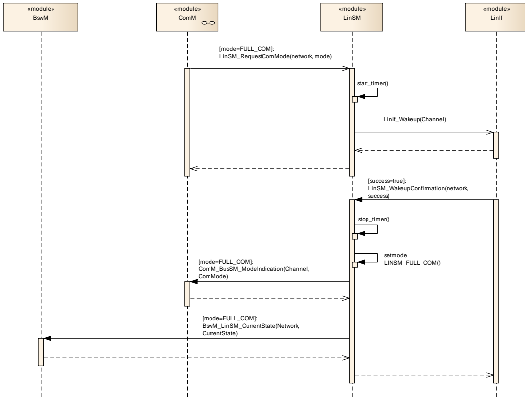
Figure 6 - Internal wake up
