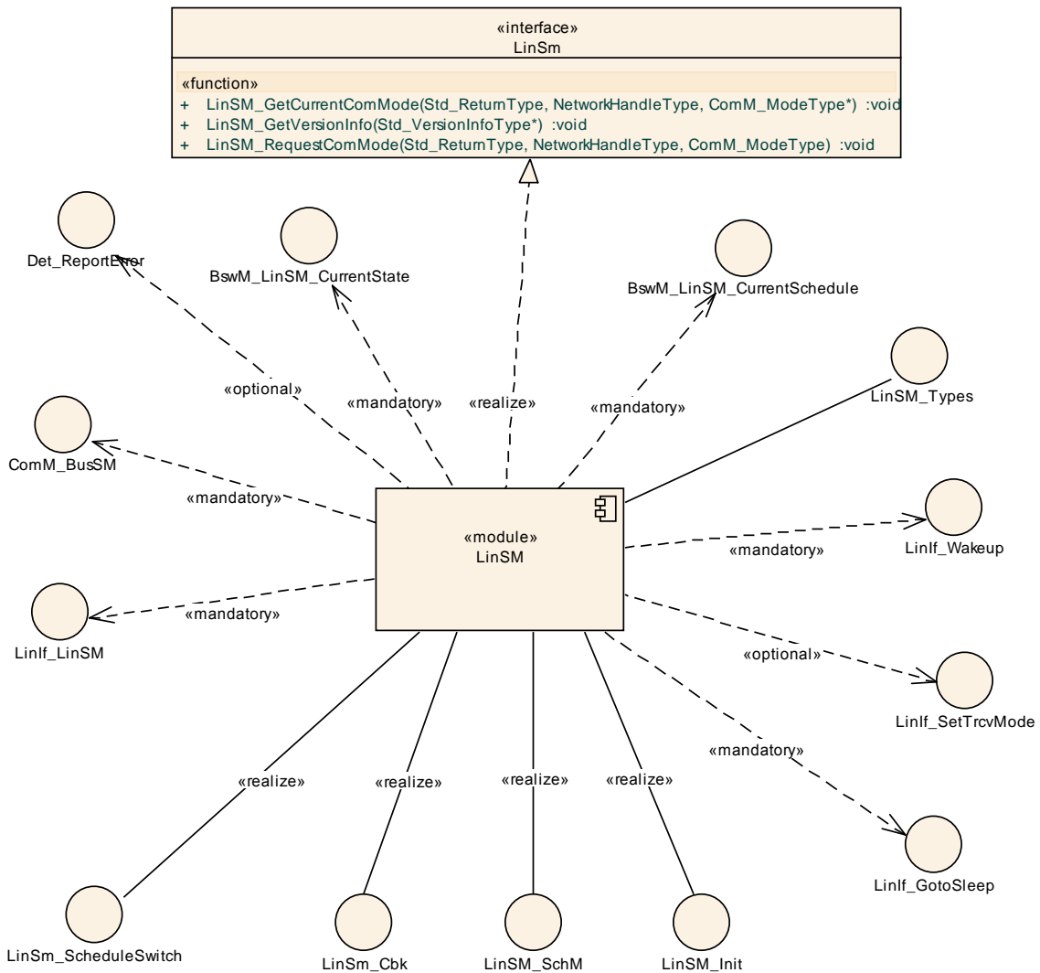
Figure 2 Dependencies to other modules
