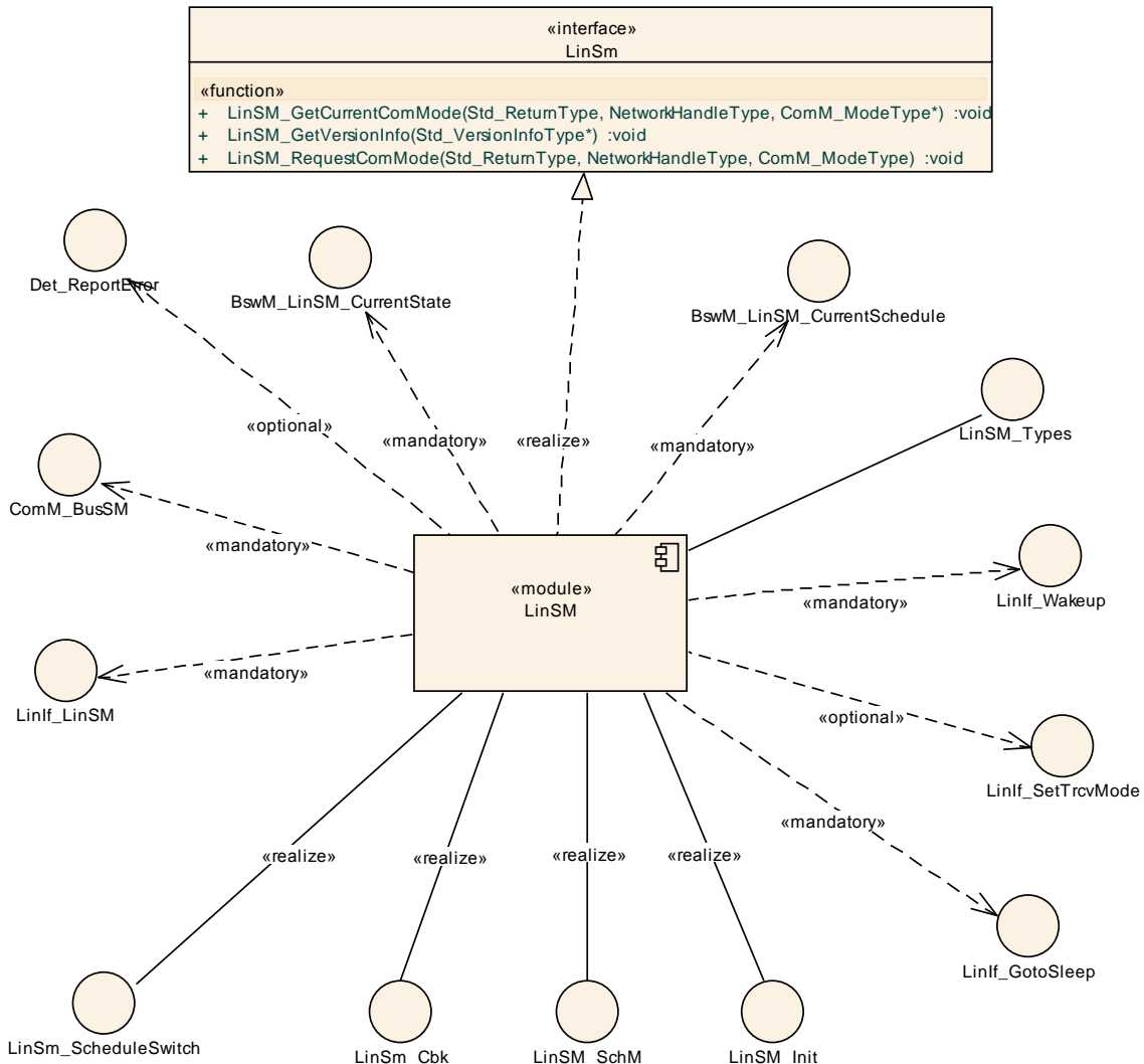
Figure 2 shows the modules that are required or optional for the realization of the LinSM module. The figure is complete but is not regarded as requirement.
