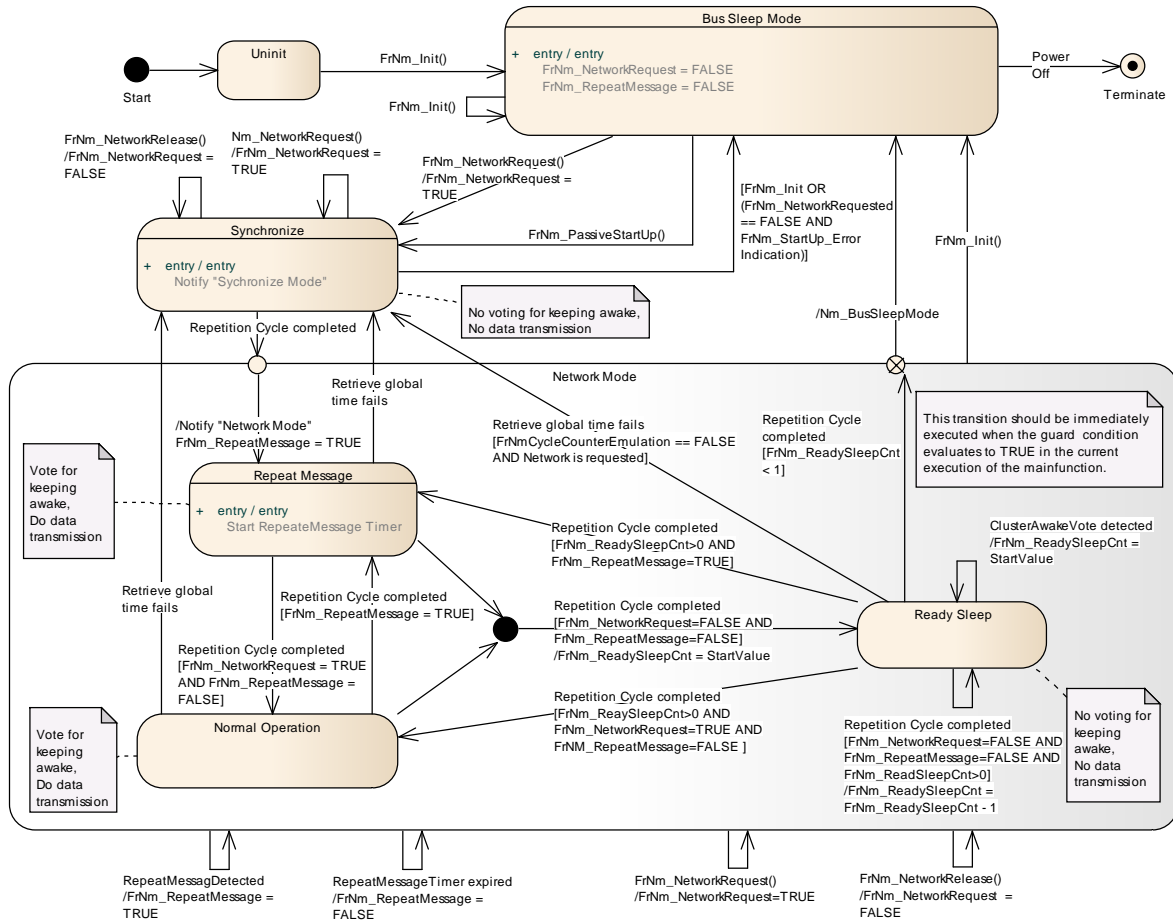
Figure The figure shows an UML state diagram with respect to the API specification.
