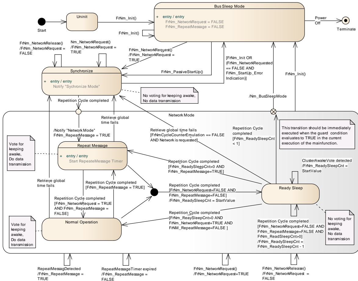
Figure (in chapter 7.4 on page 36) shows the detailed UML state chart of the FlexRay NM.
