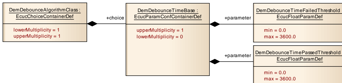
Figure 29 Time based debounce algorithm
