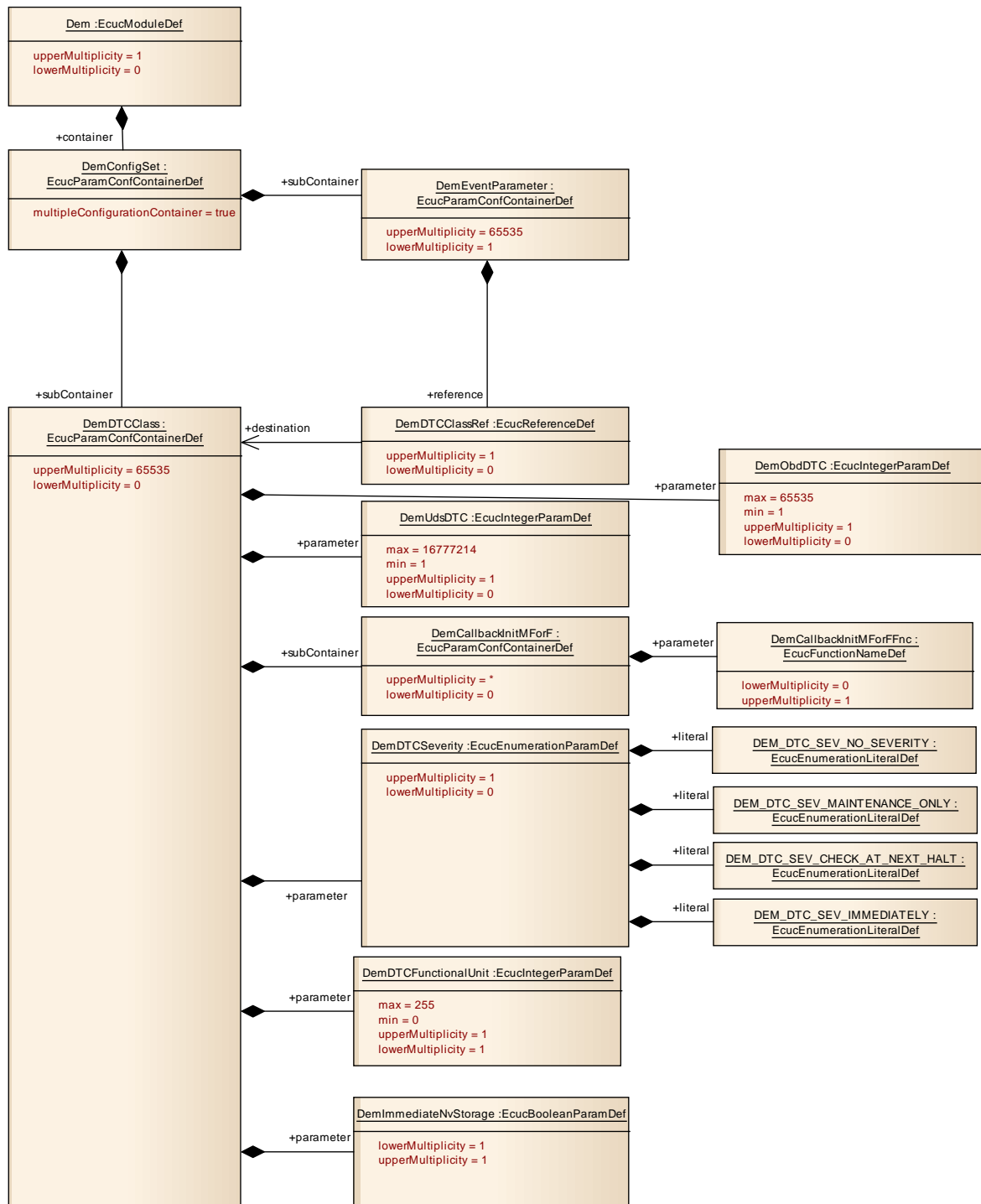
Figure 8 DTC configuration
