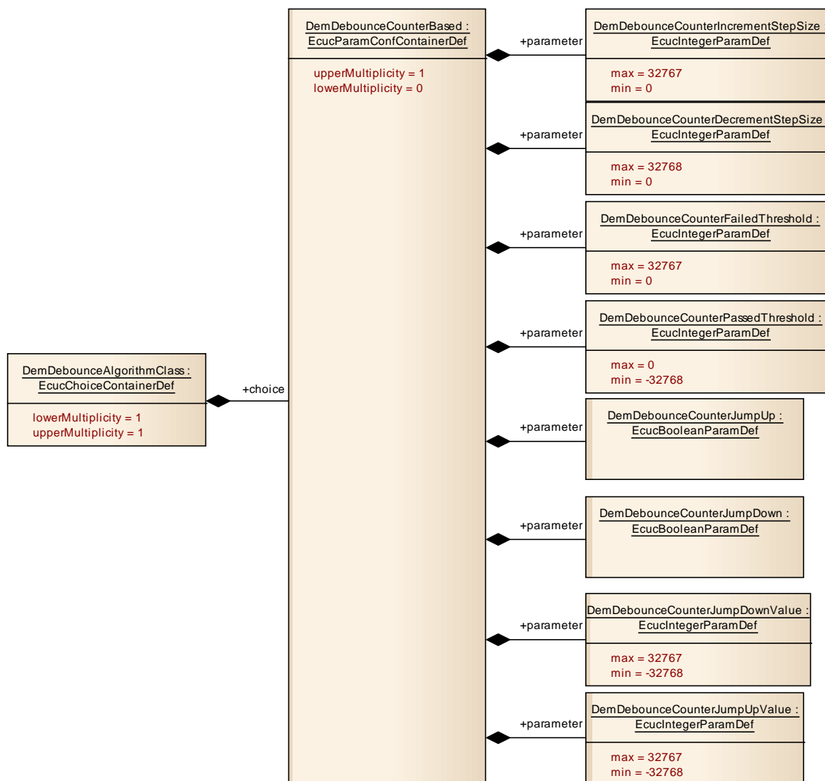
Figure 27 Counter based debounce algorithm
