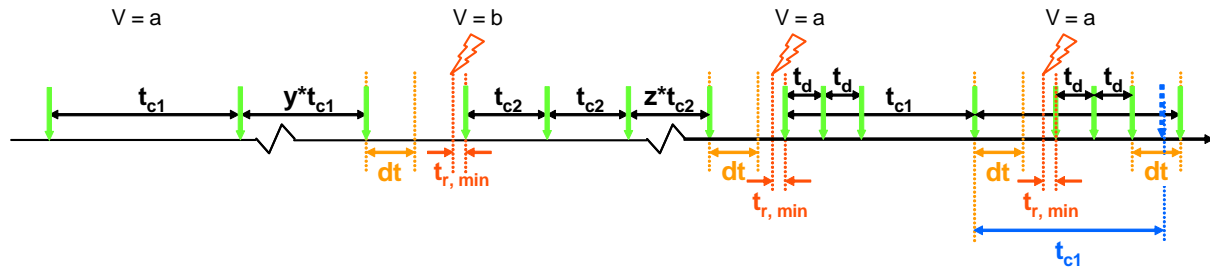
Figure 26: Use Case 6, TM MIXED , here n=3 + periodic (with TMS switch)
