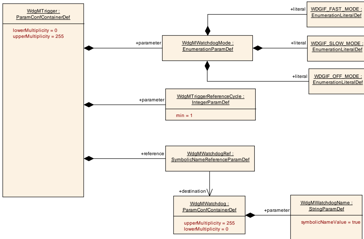
Figure 26: Configuration Container WdgMTrigger
