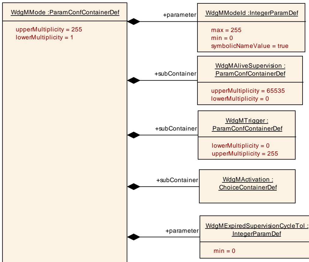
Figure 24: Configuration Container WdgMMode
