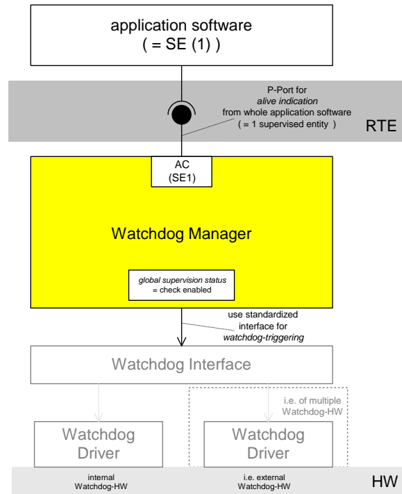
Figure 2: Alive-supervision of a single entity
