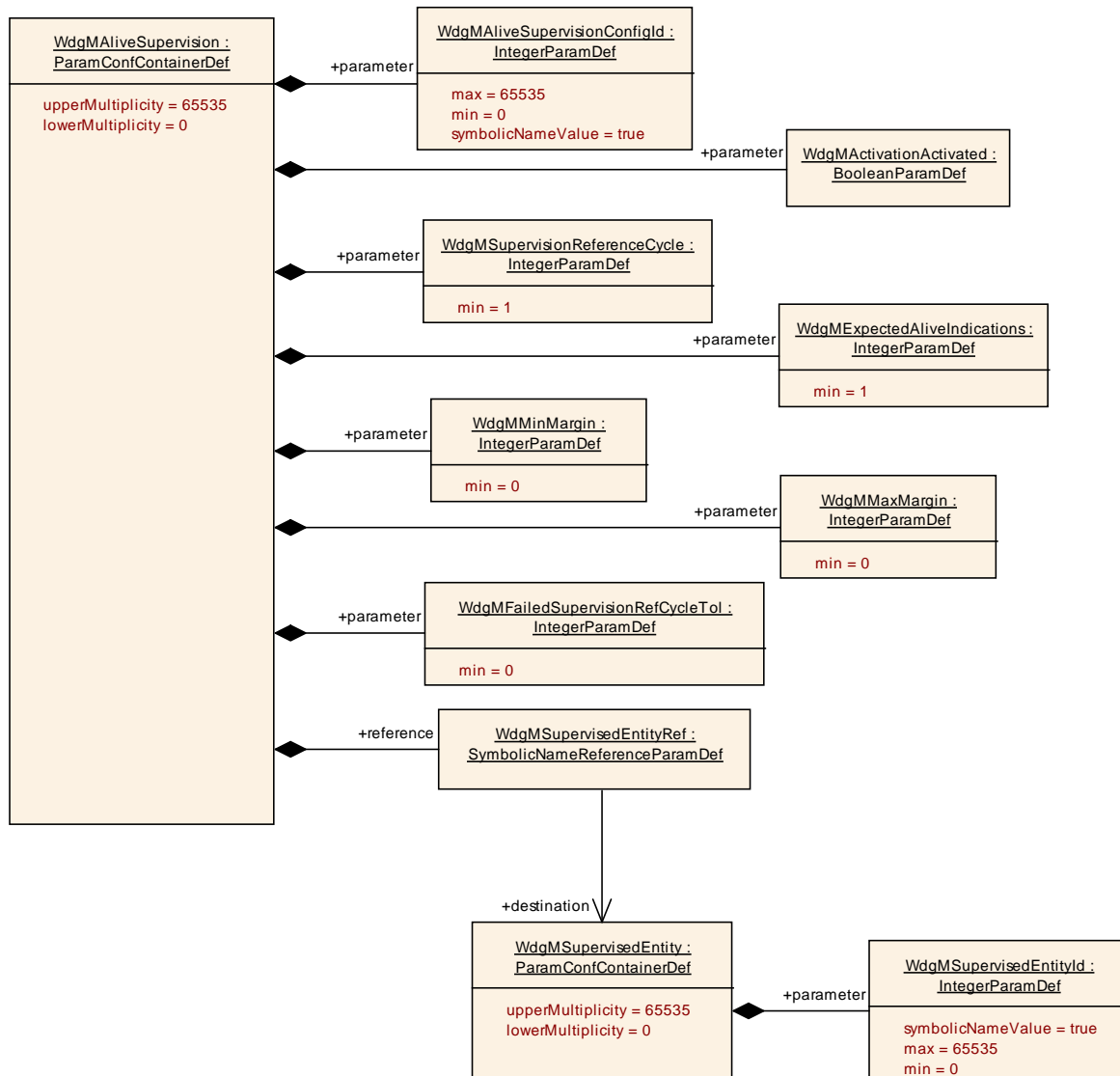
Figure 25: Configuration Container WdgMAliveSupervision
