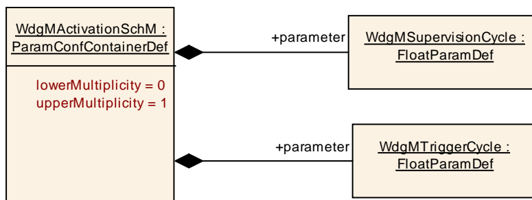
Figure 28: Configuration Container WdgMActivationSchM
