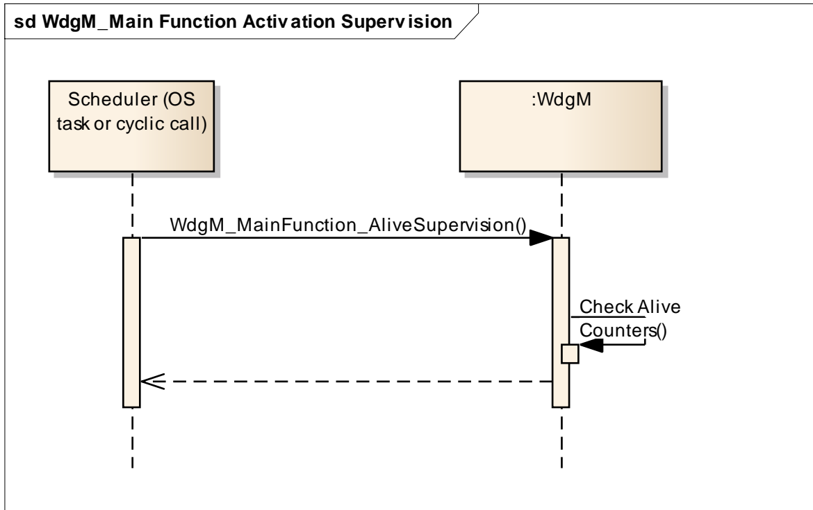
Figure 16: Main Function Activation for Alive-supervision
