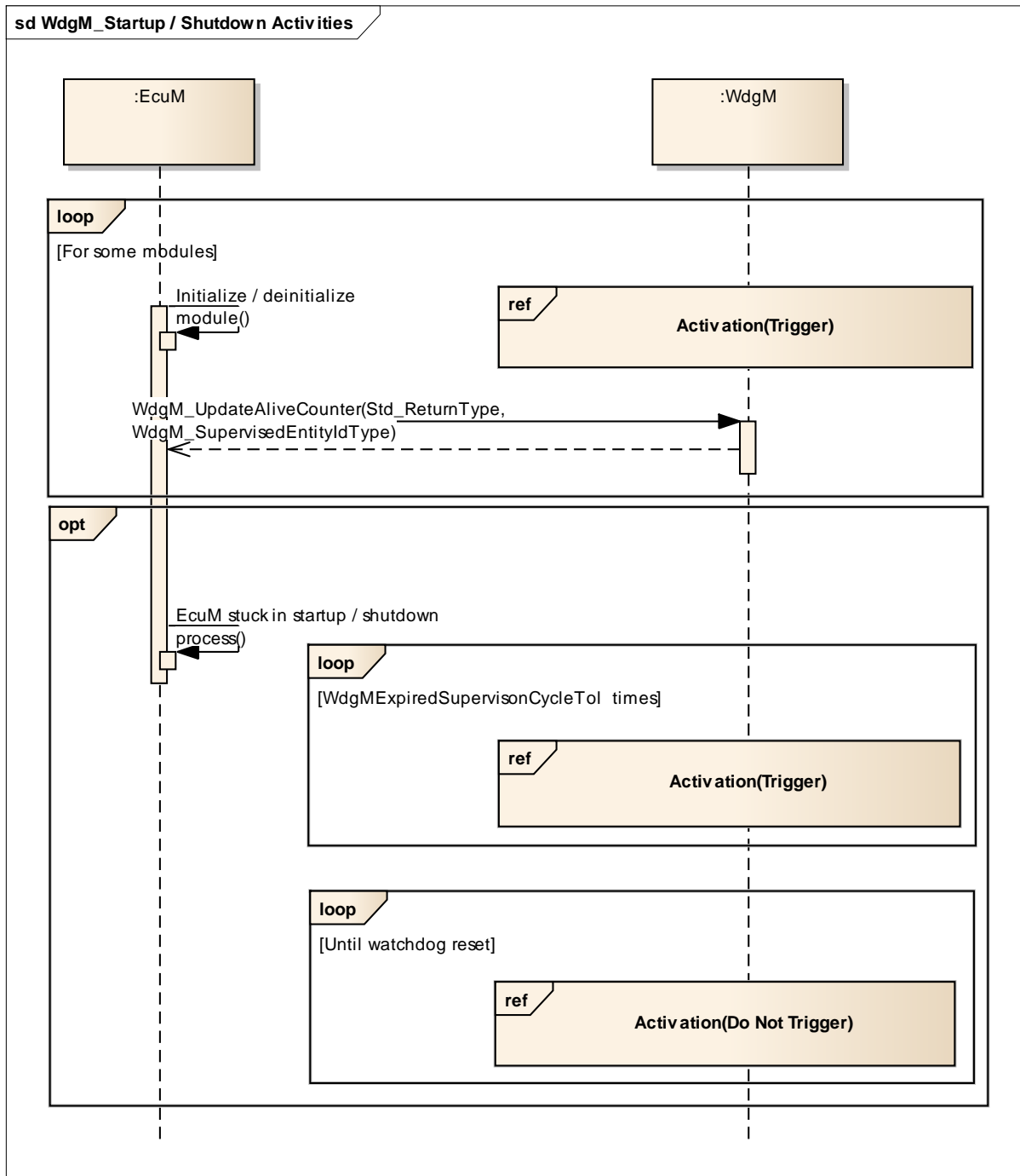
Figure 14: Startup and Shutdown Activities
