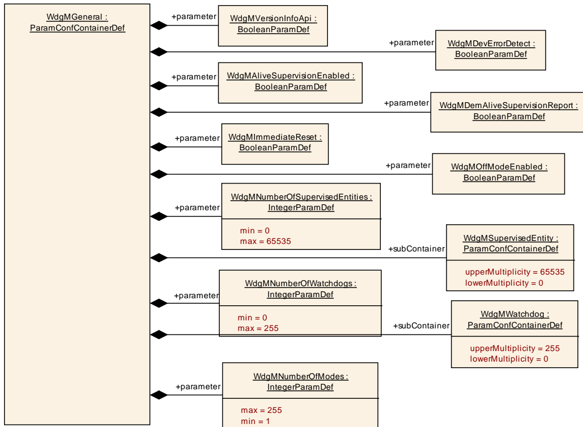
Figure 20: Configuration Container WdgMGeneral
