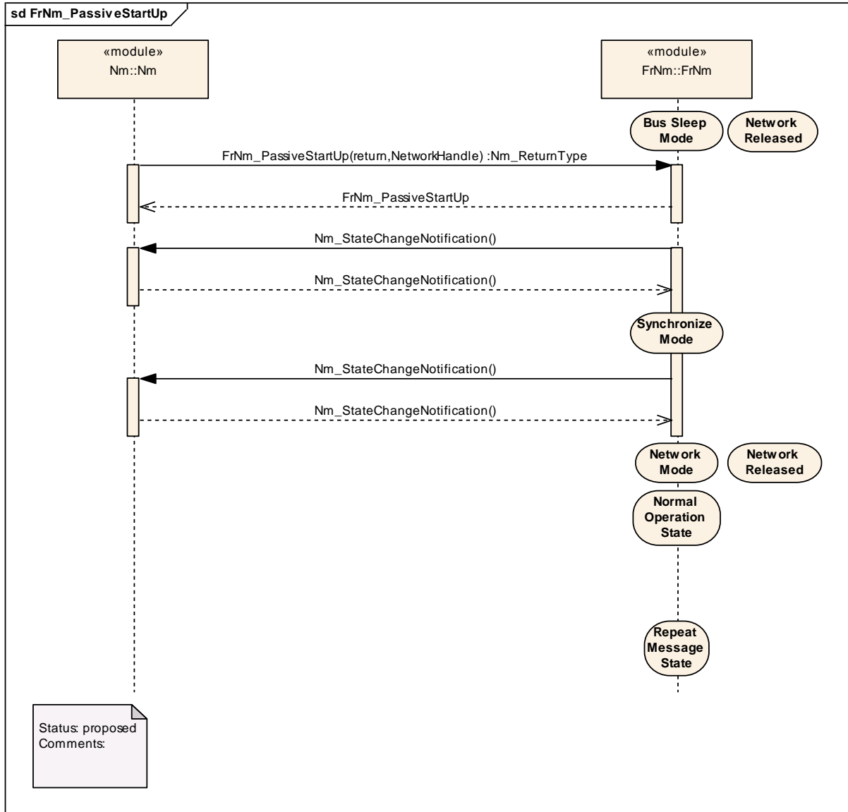
Figure 9-1 FrNm passive startup sequence
