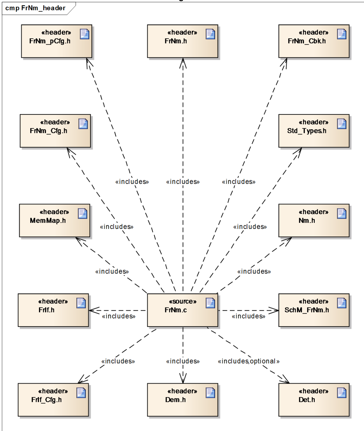
5-2 Header File Structure
