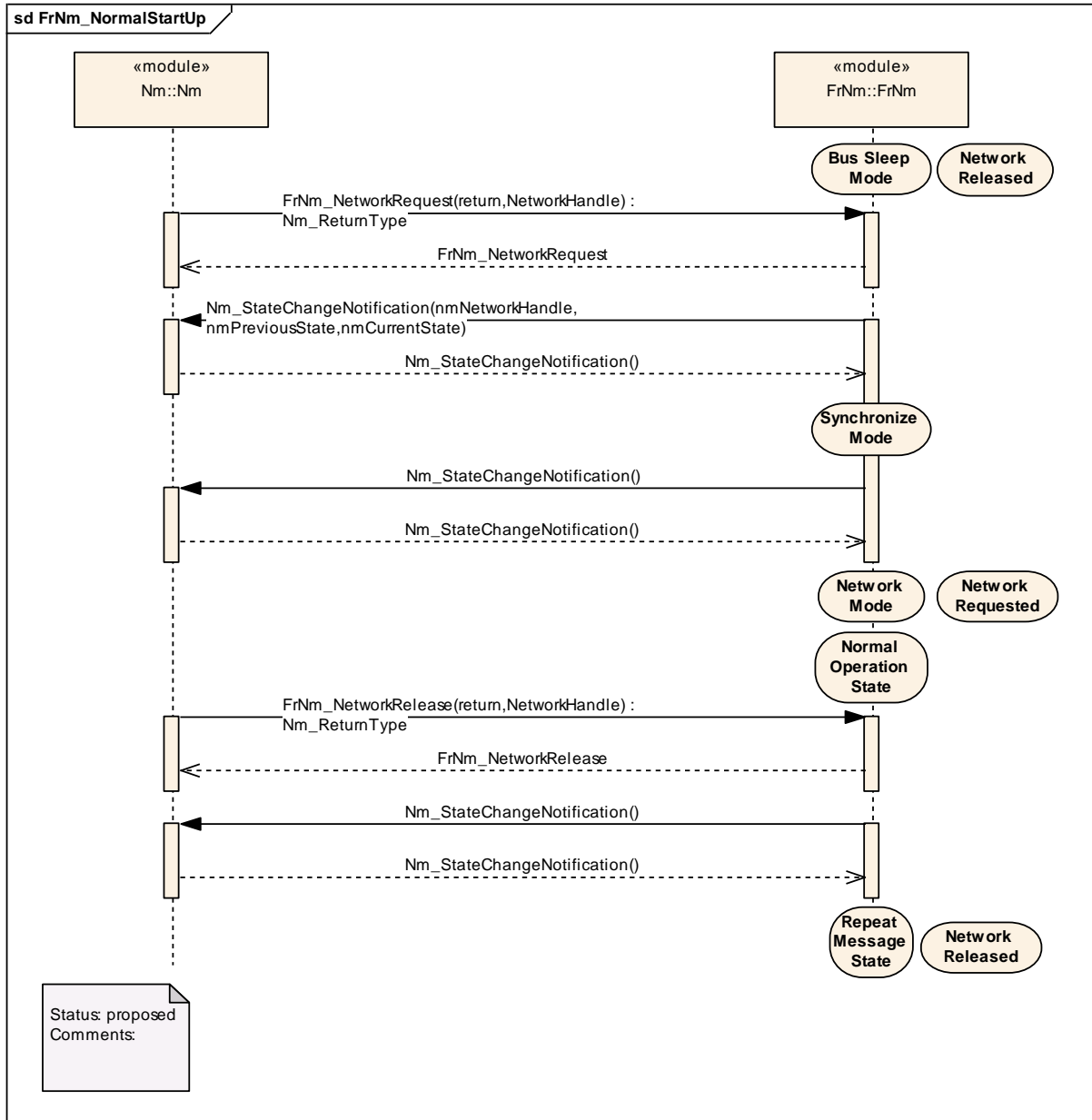
Figure 9-3 FrNm normal operation sequence
