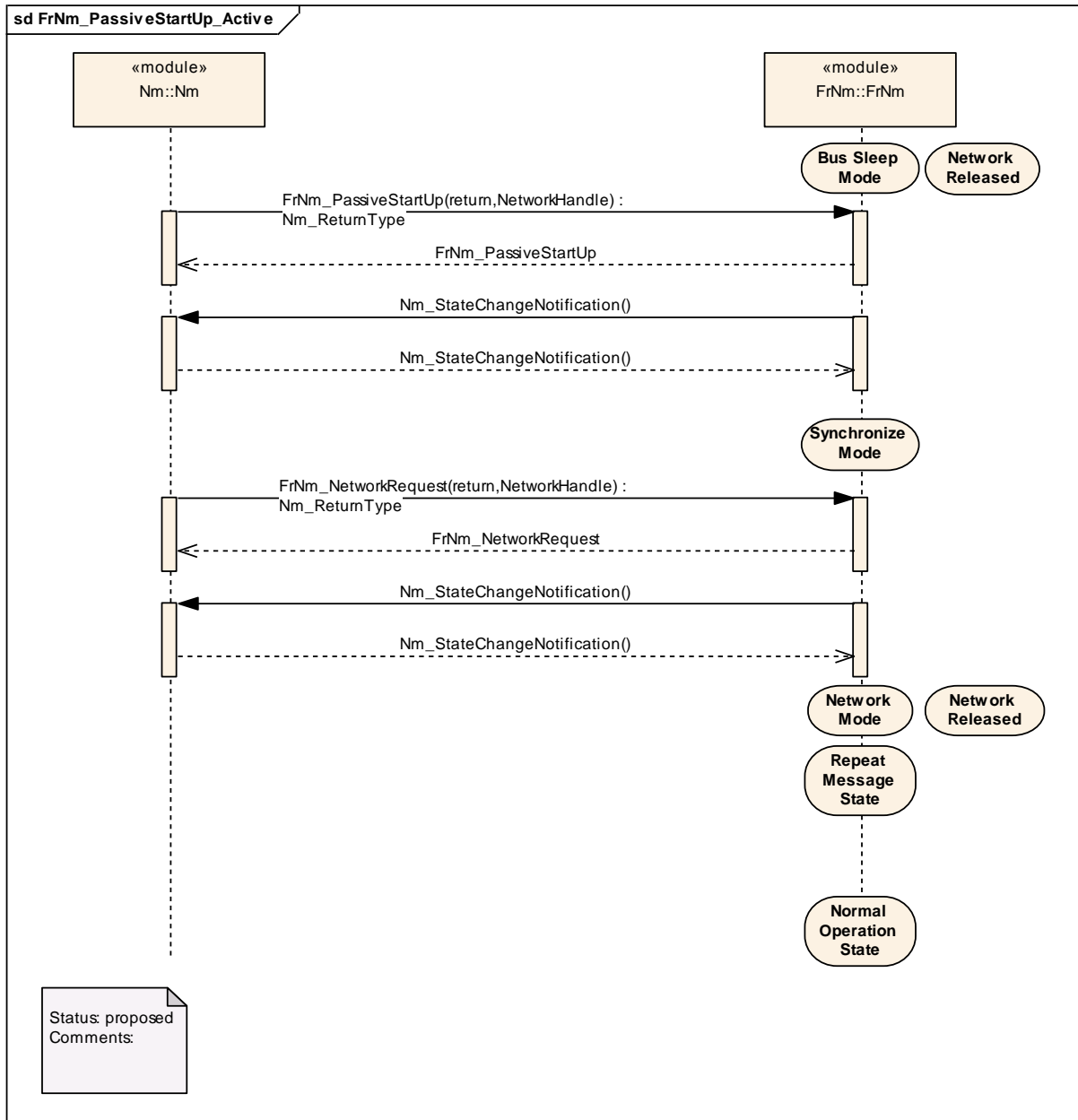
Figure 9-2 FrNm passive startup with a “active” network request sequence
