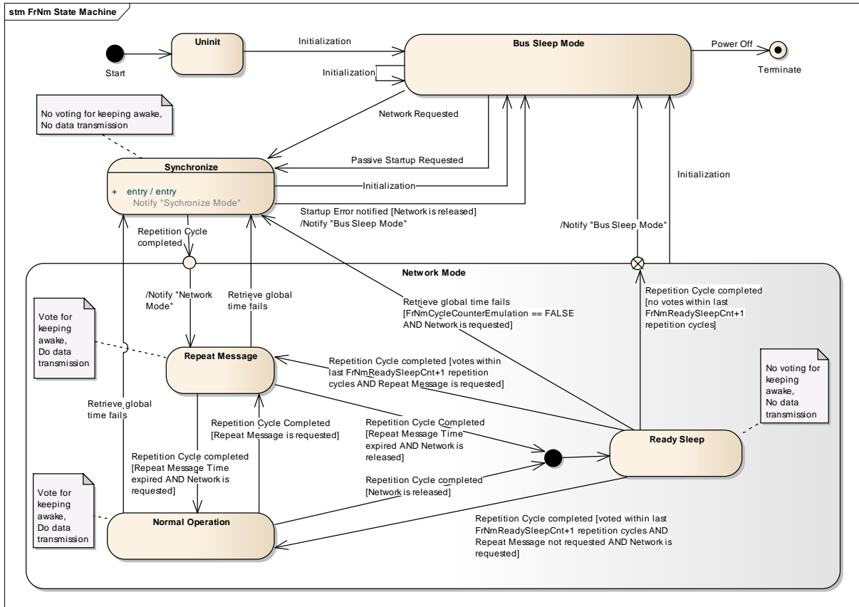
Figure 7-1 UML State Chart
