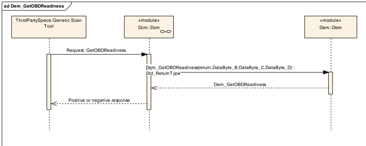
Figure 27 Sequence diagram of Dem_GetOBDRoadiness
