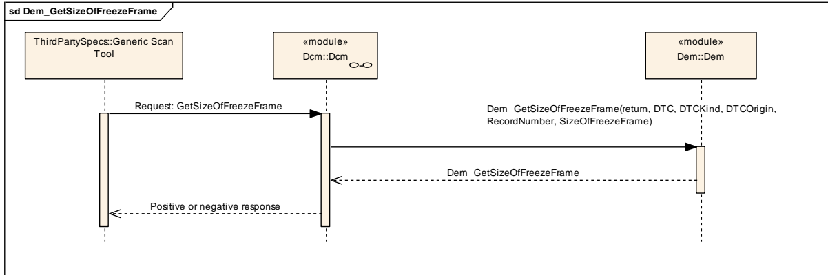
Figure 29 Sequence diagram of Dem_GetSizeOfFreezeFrame
