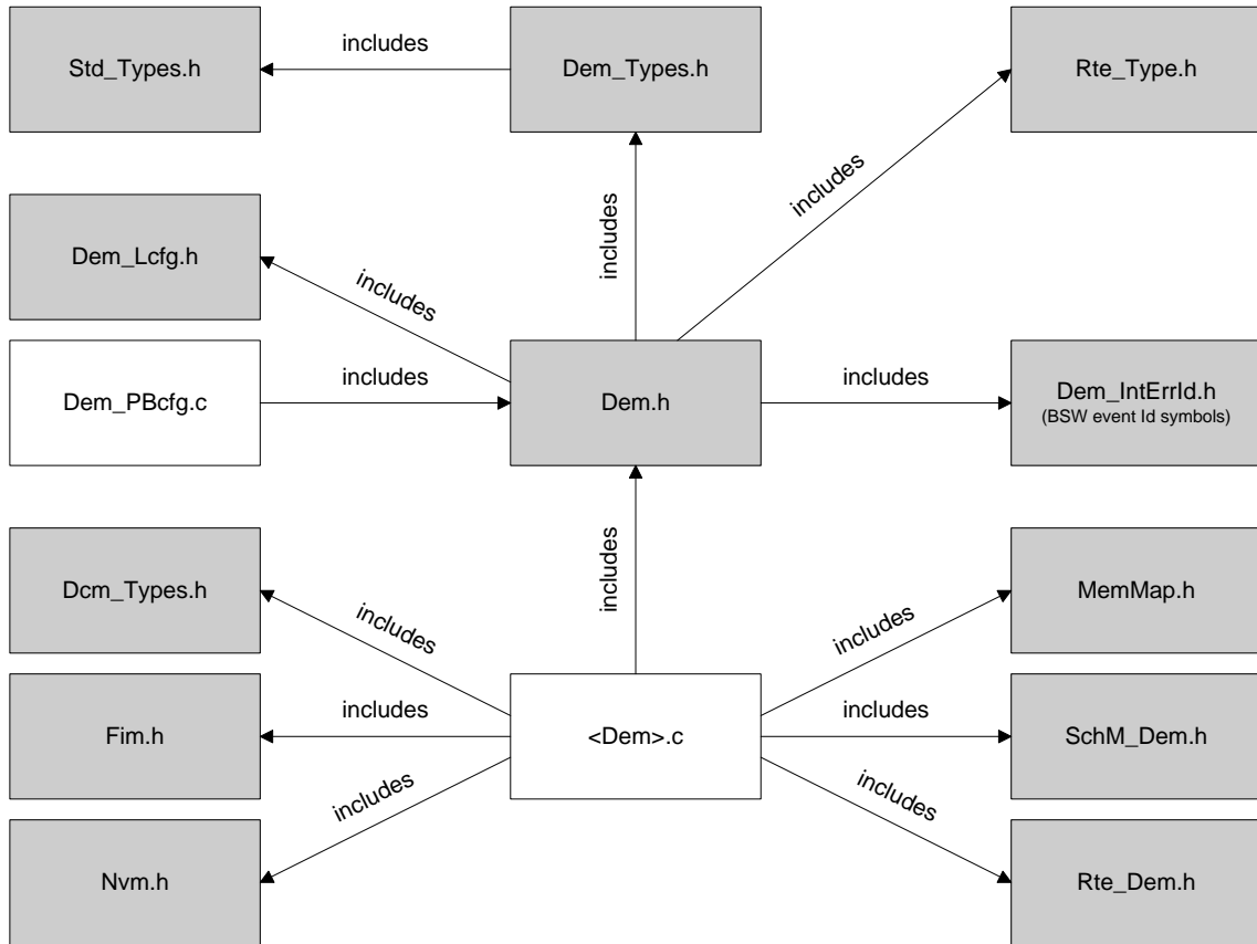
Figure 2 Header file structure
