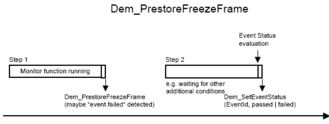
Figure 8 Example to use Dem_PrestoreFreezeFrame to prestore FreezeFrame data
