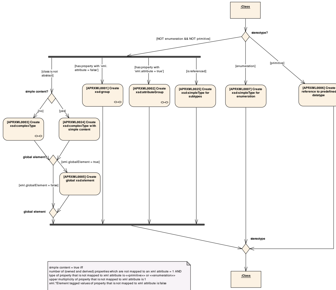
Figure 5-2: Class representation
