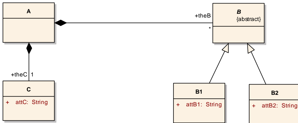
Figure 4-1: Example metamodel
