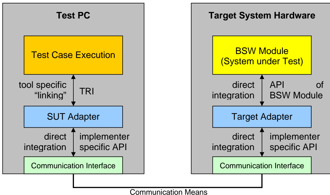
Figure 3 - Integration interfaces for SUT adapter and target adapter
