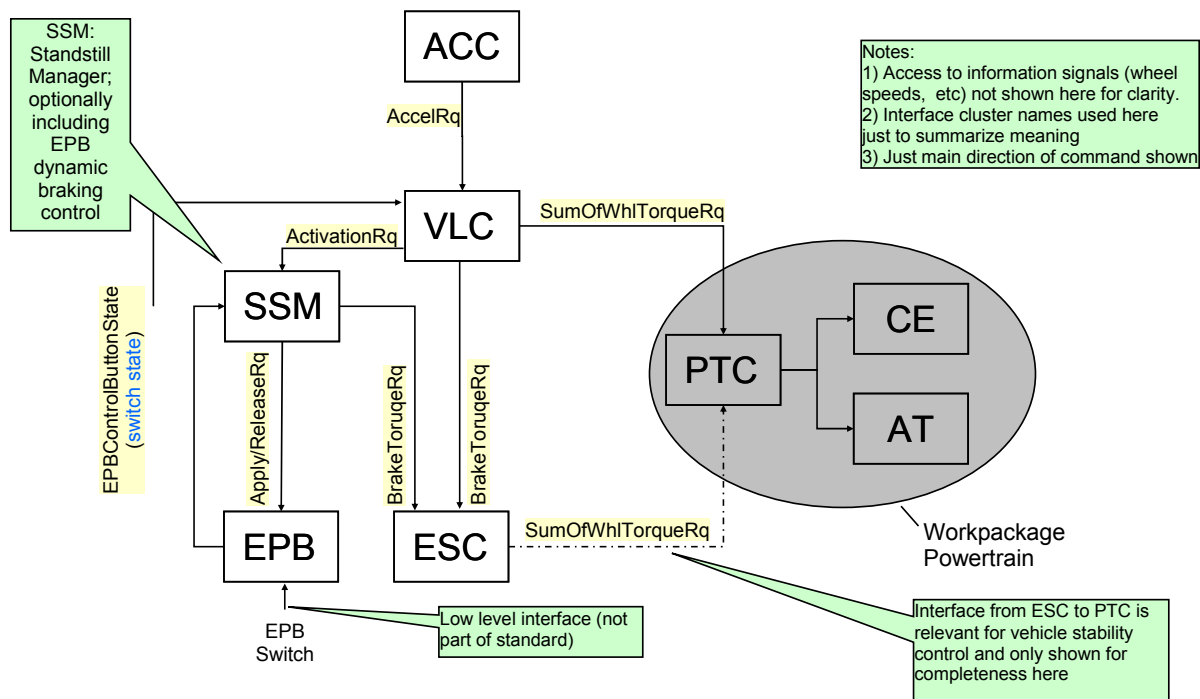
Figure 3: Overview of the Software Composition VLC
