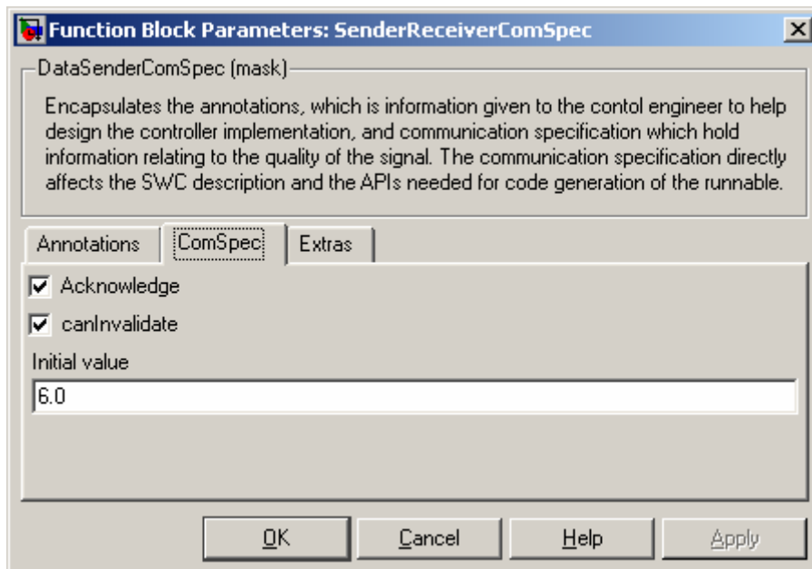
Figure 17: DataSenderComSpec parameters.
