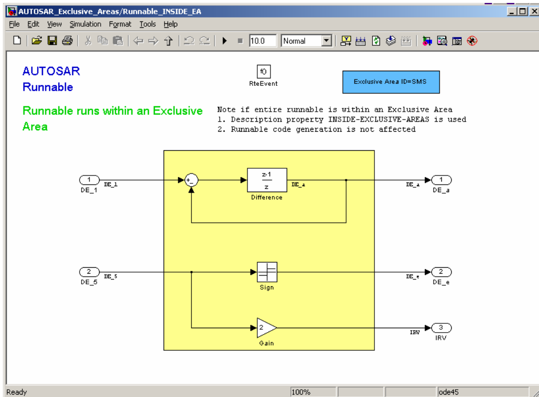
Figure 10: Entire runnable is within an Exclusive Area
