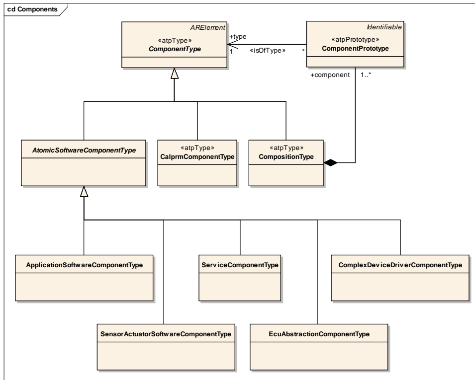
Figure 4.1: AUTOSAR SW-Component classification
