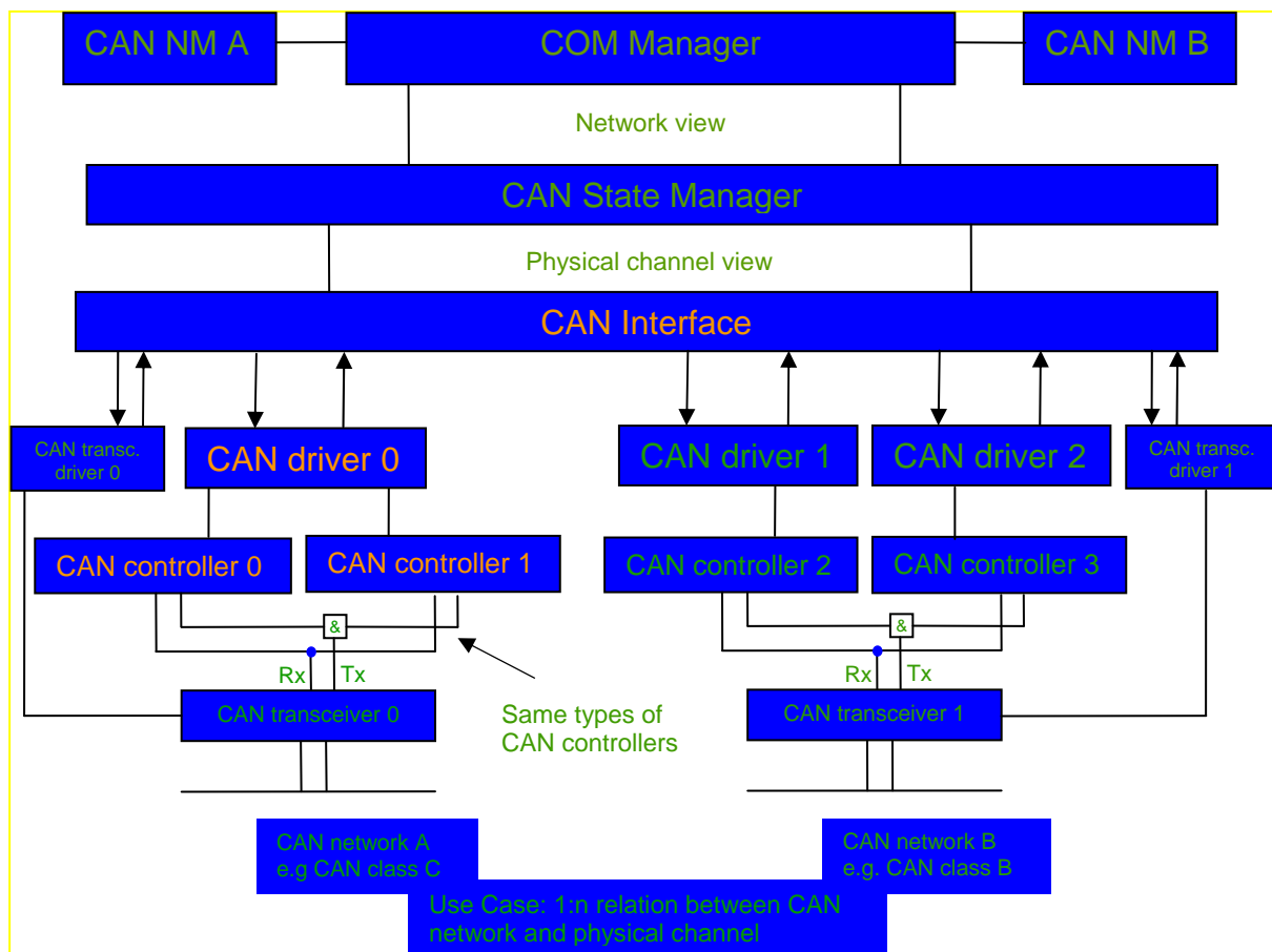
Figure 5: Physical channel view definition example B
