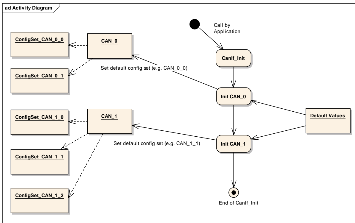
Figure 7 Controller specific initialization of CAN Interface and CAN Driver
