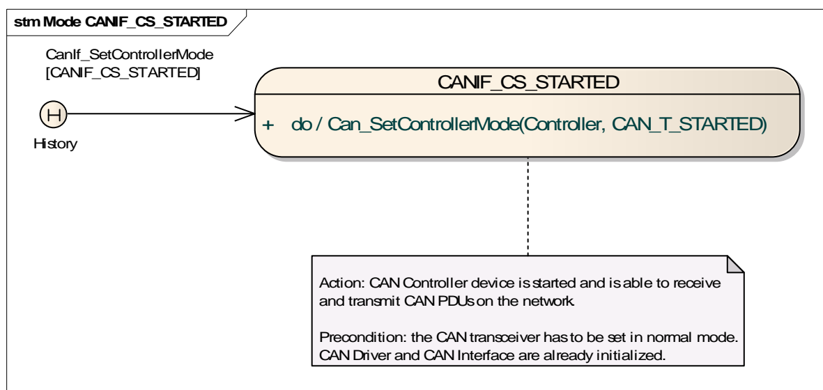
Figure 14 Activities of STARTED mode transition
