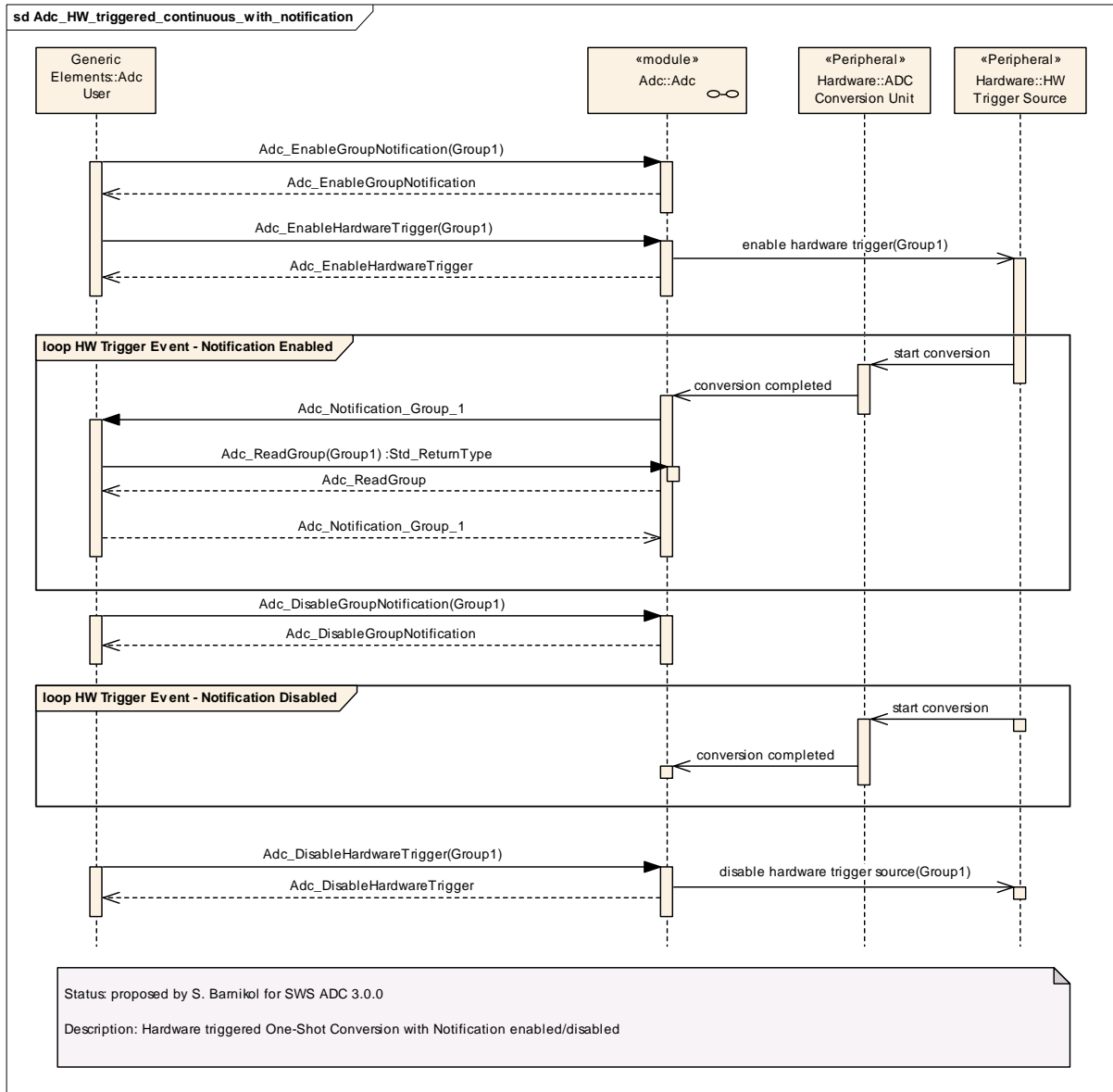
Figure 17: Hardware triggered one-shot conversion with notification
