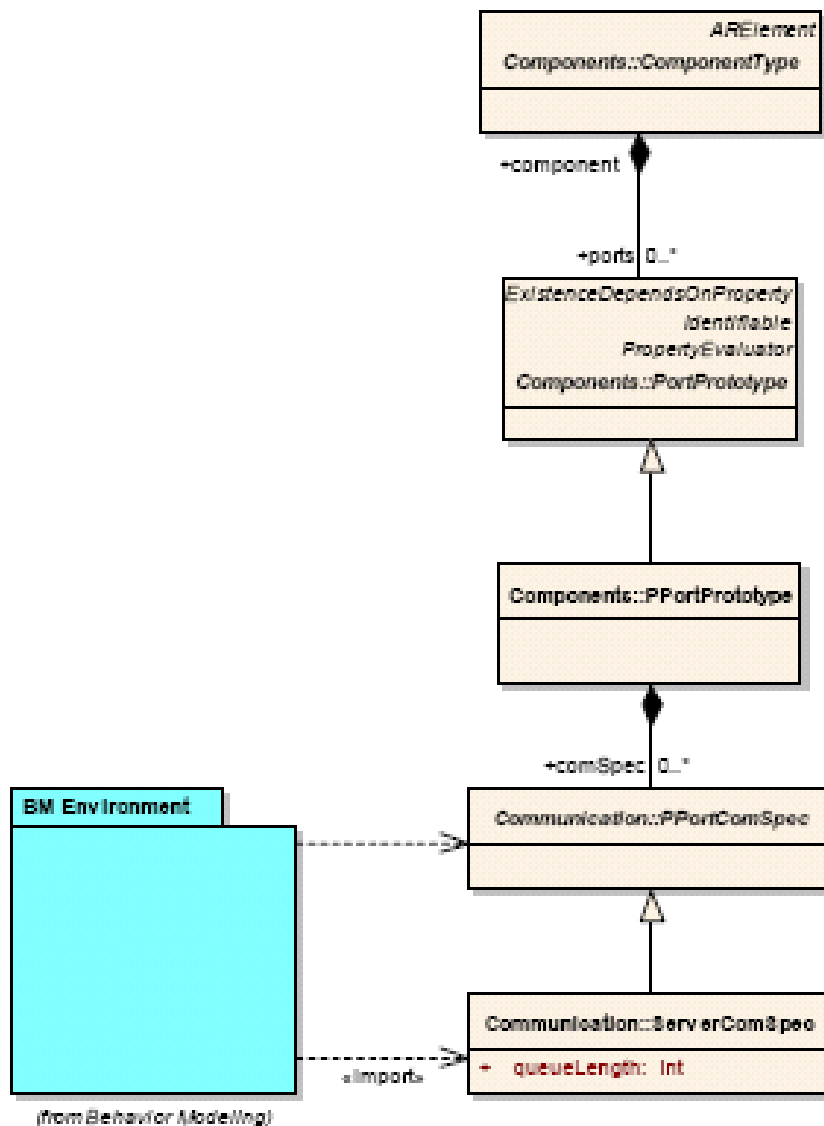
Figure 17: ServerComSpec
