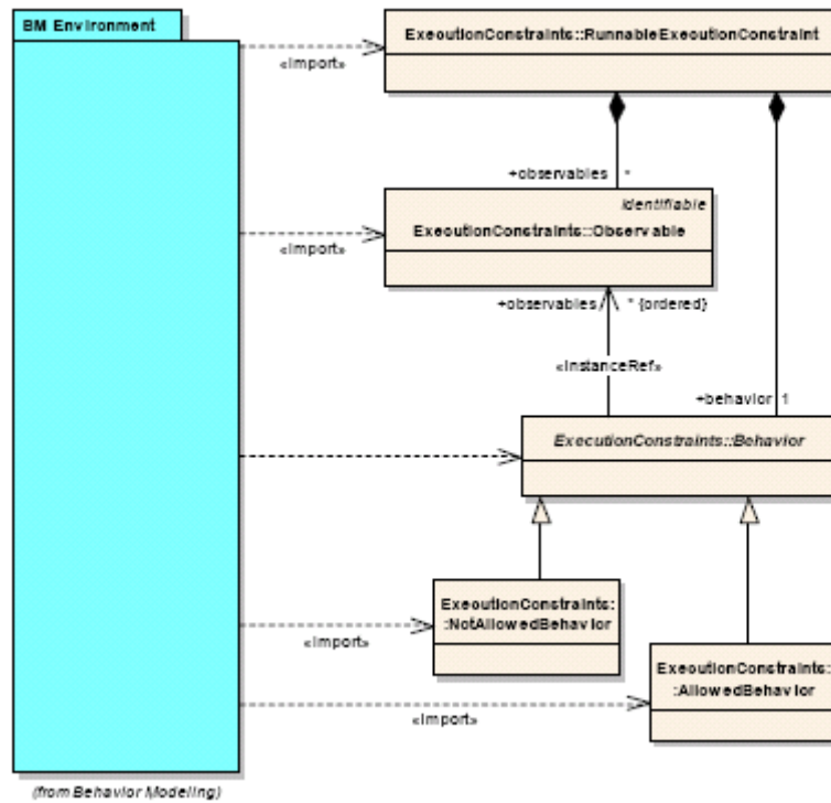
Figure 19: Execution Constraints
