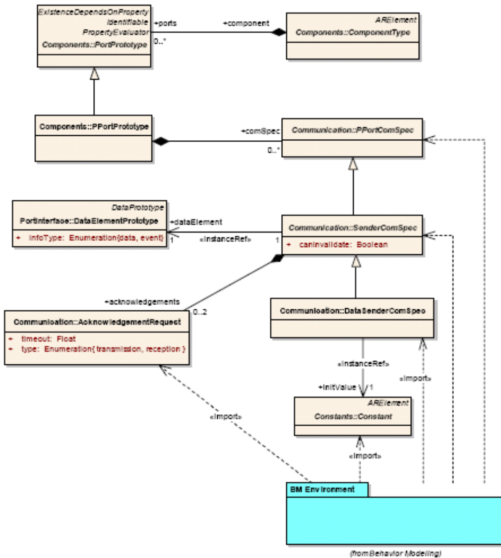
Figure 15: SenderComSpec
