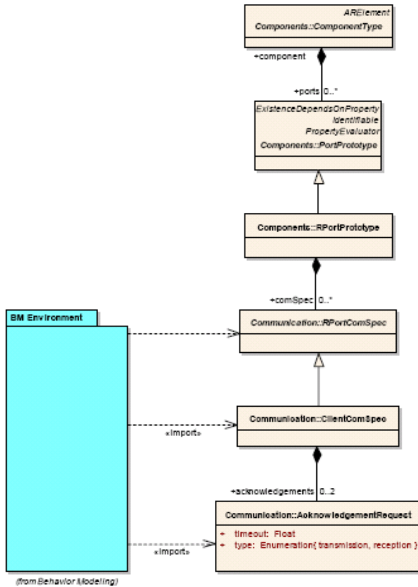
Figure 16: ClientComSpec
