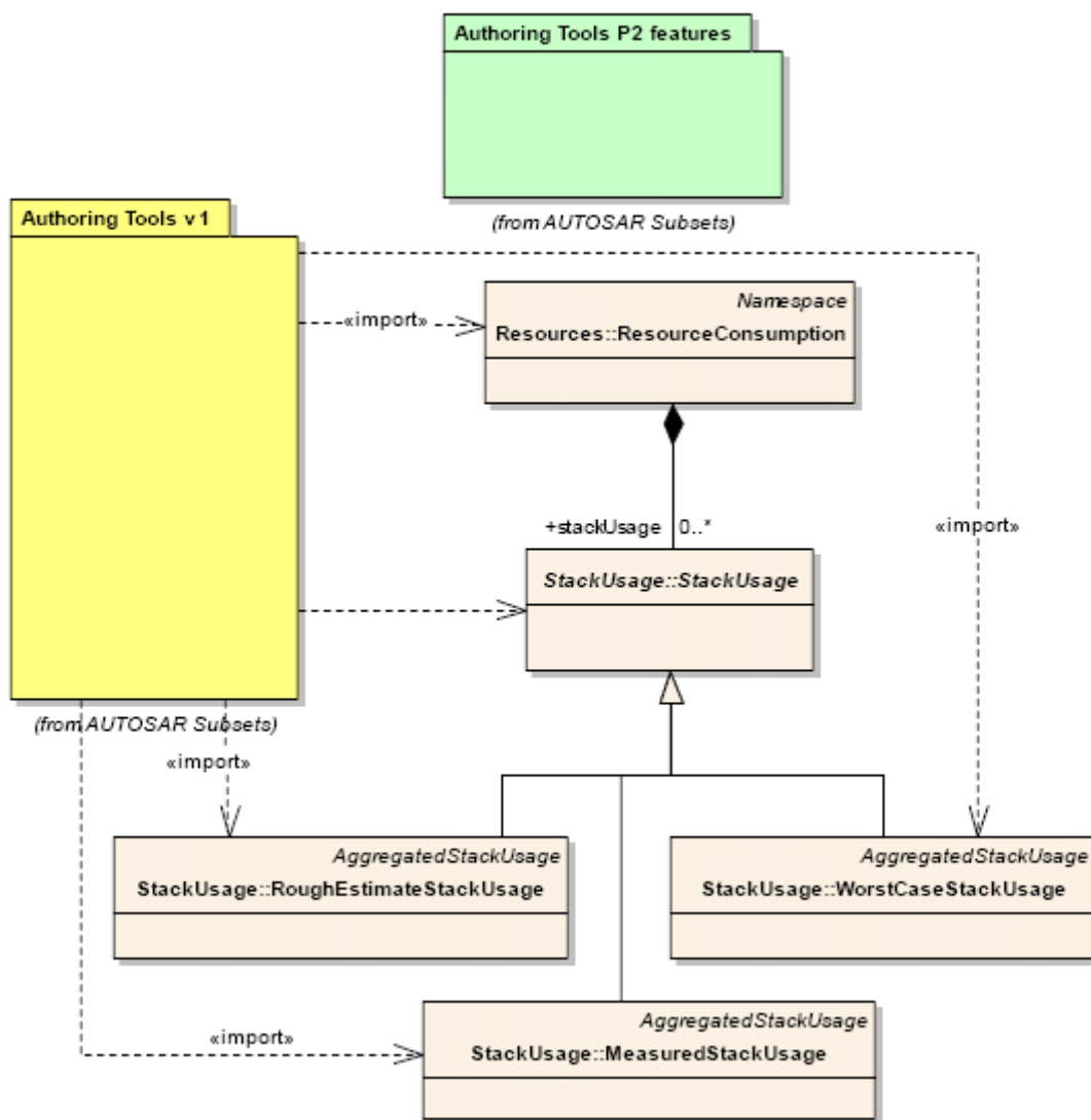
Figure 6-10: Annotation of the meta-model for the support of memory resource requirement (II)
