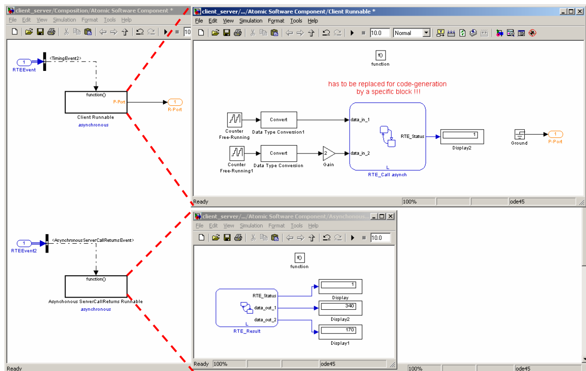
Figure 26: Model of Client Runnable (Asynchronous)
