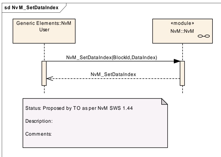
Figure 11: UML sequence diagram NvM_SetDataIndex
