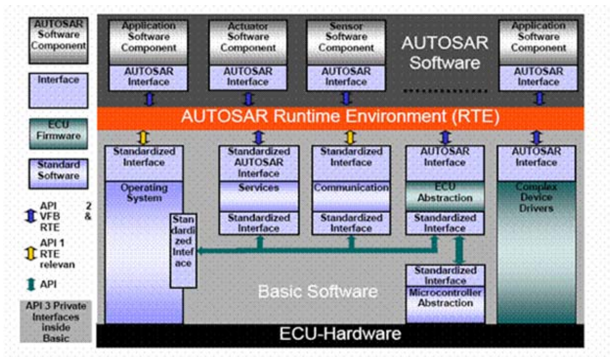
Figure 7.1: Autosar architecture
