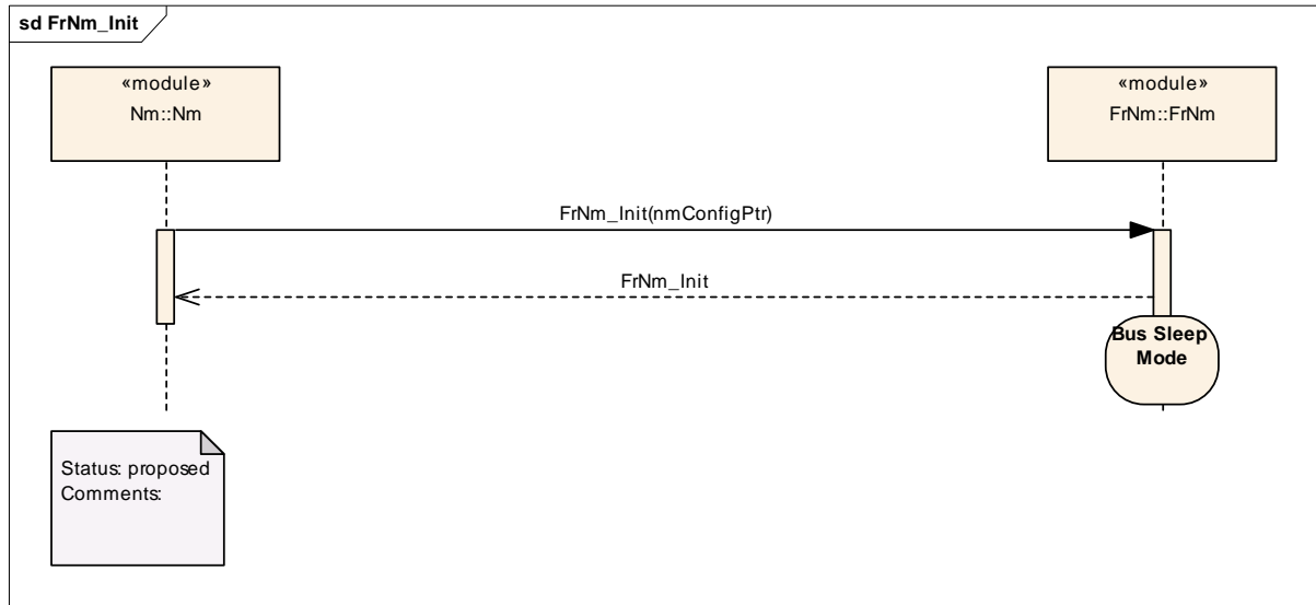
Figure 9-1 FrNm Init Sequence
