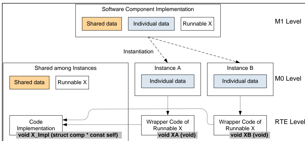
Figure 35: Wrapper Runnables
