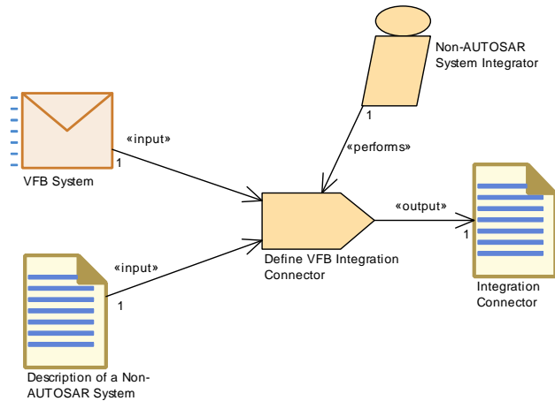
Figure 3.39: Task Define VFB Integration Connector
