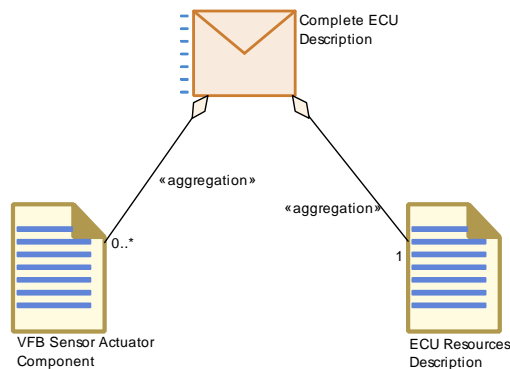
Figure 3.63: Complete ECU Description
