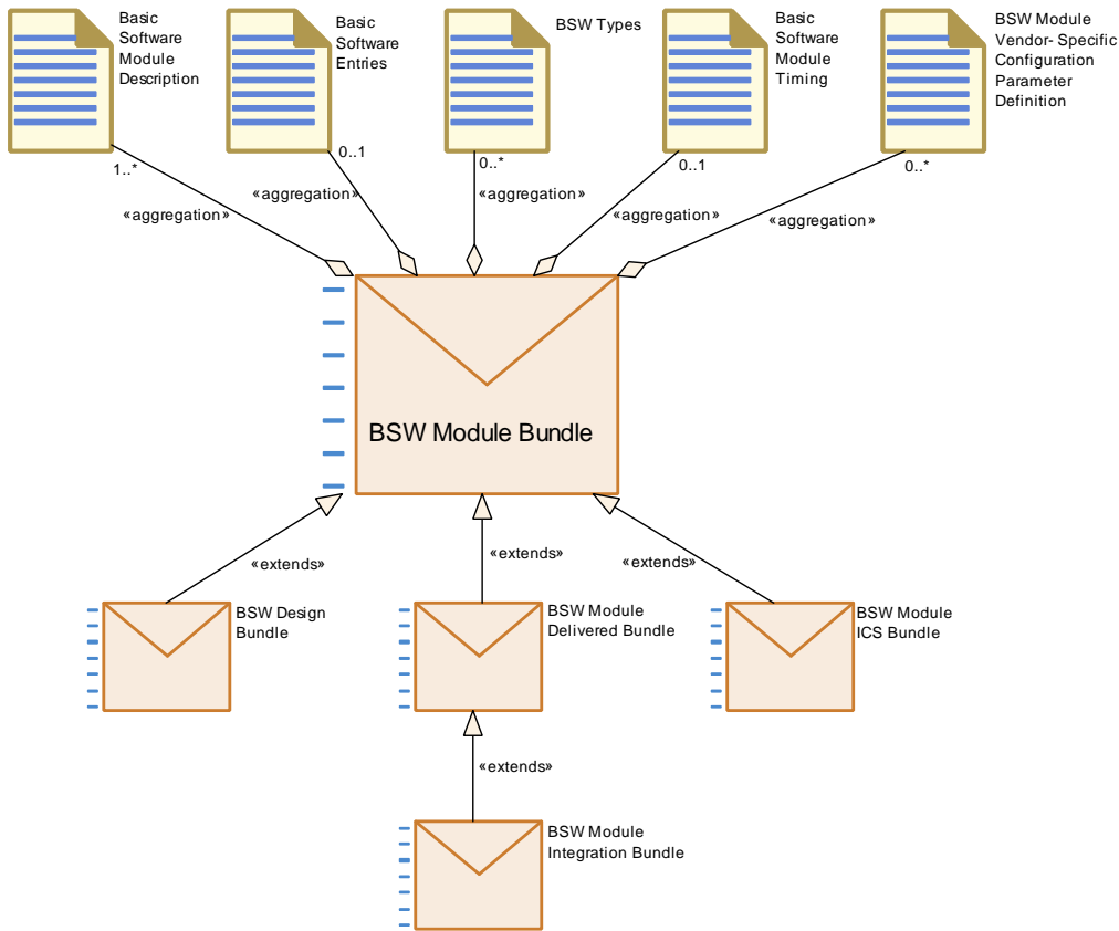
Figure 3.116: BSW Module Bundle
