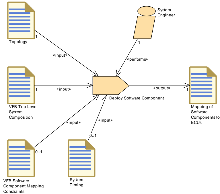
Figure 3.50: Deploy Software Component
