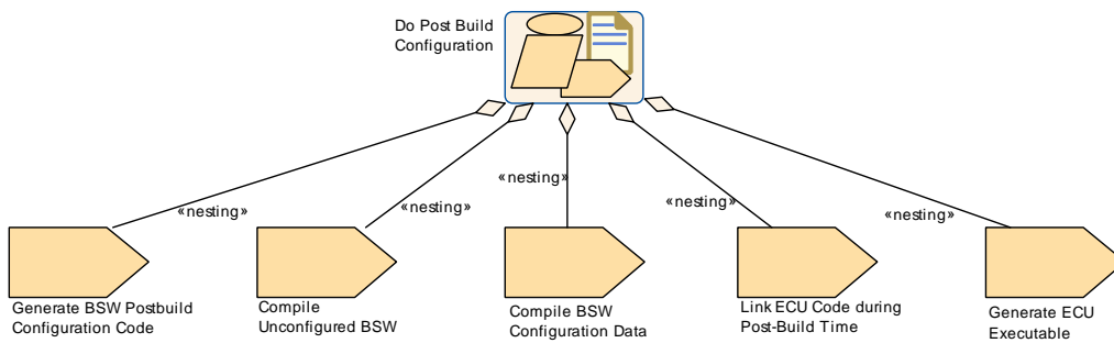
Figure 2.57: Work Flow for Post-Build Configuration
