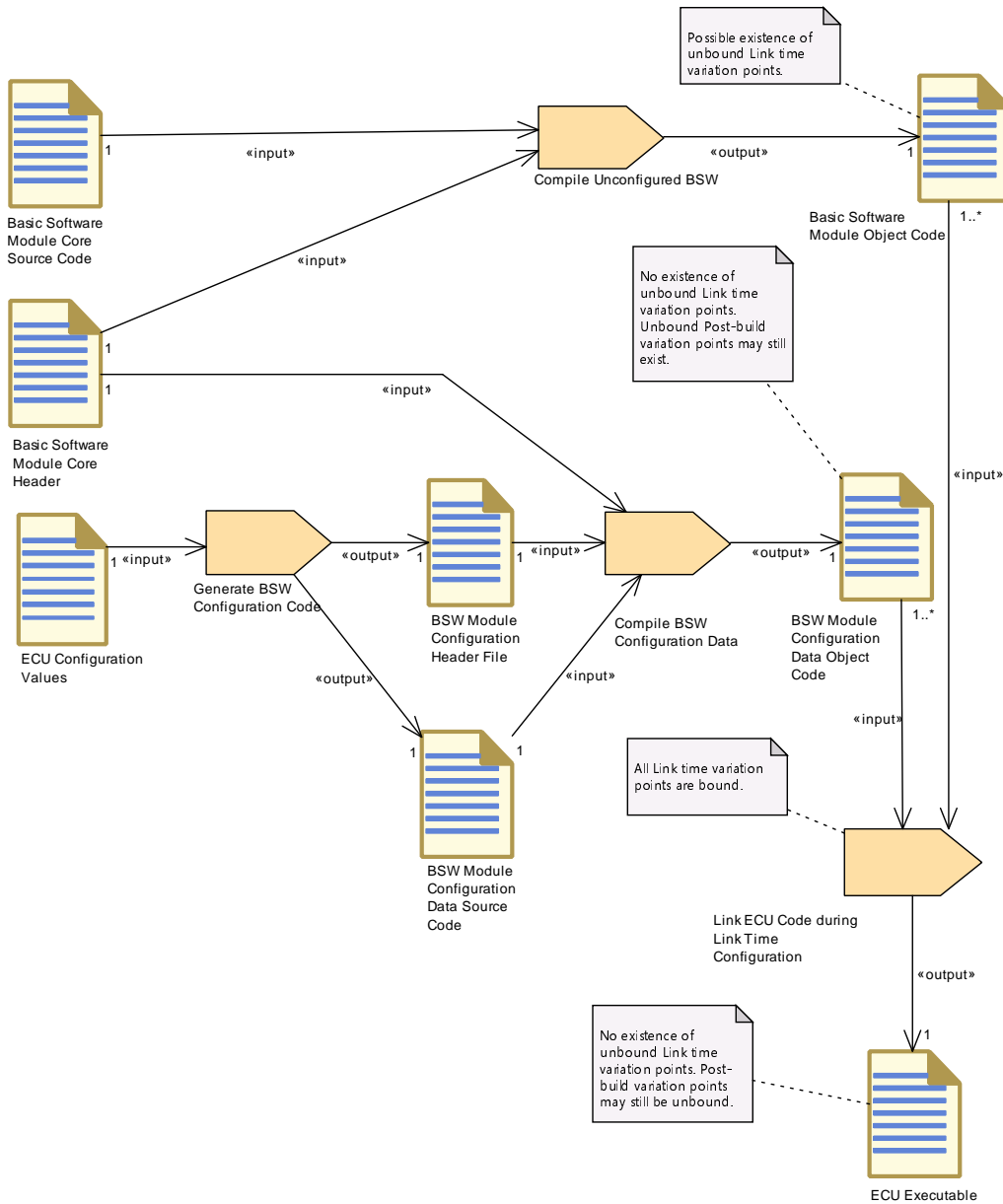
Figure 2.53: Overview Link Time Configuration
