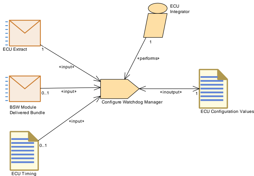
Figure 3.127: Configure Watchdog Manager
