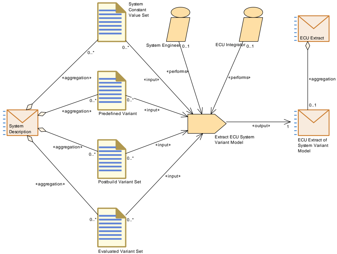
Figure 3.84: Extract the ECU System Variant Model
