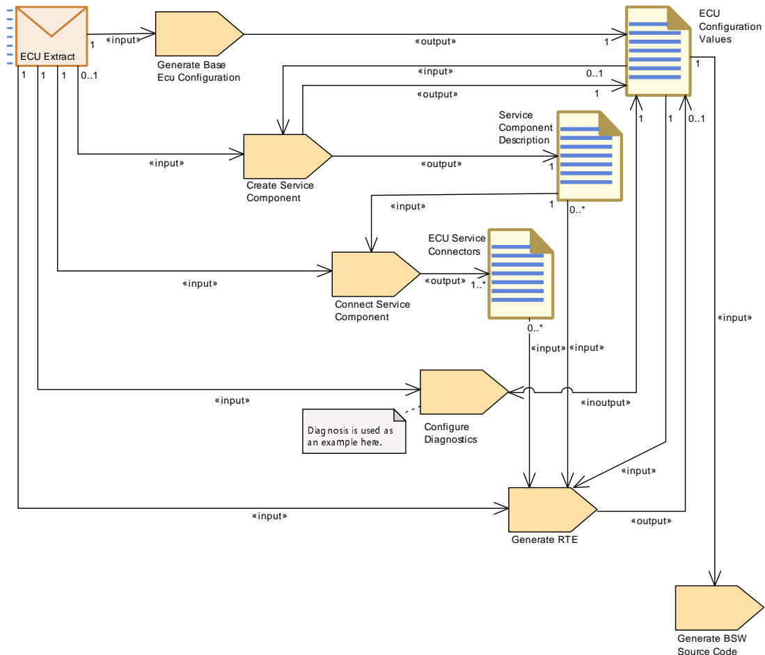
Figure 2.60: Connect and Configure Service Module on ECU - Detailed view with work products
