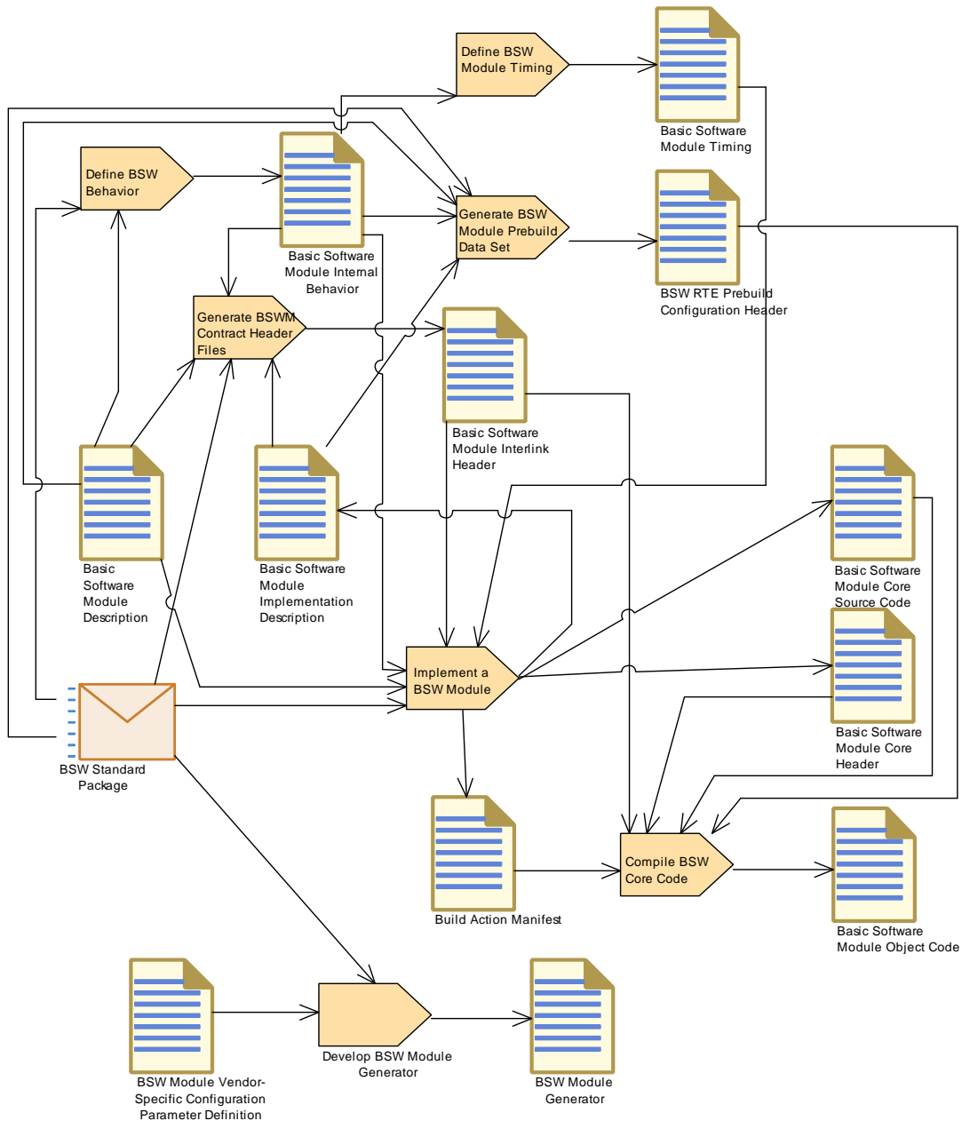
Figure 2.40: Develop Basic Software Module
