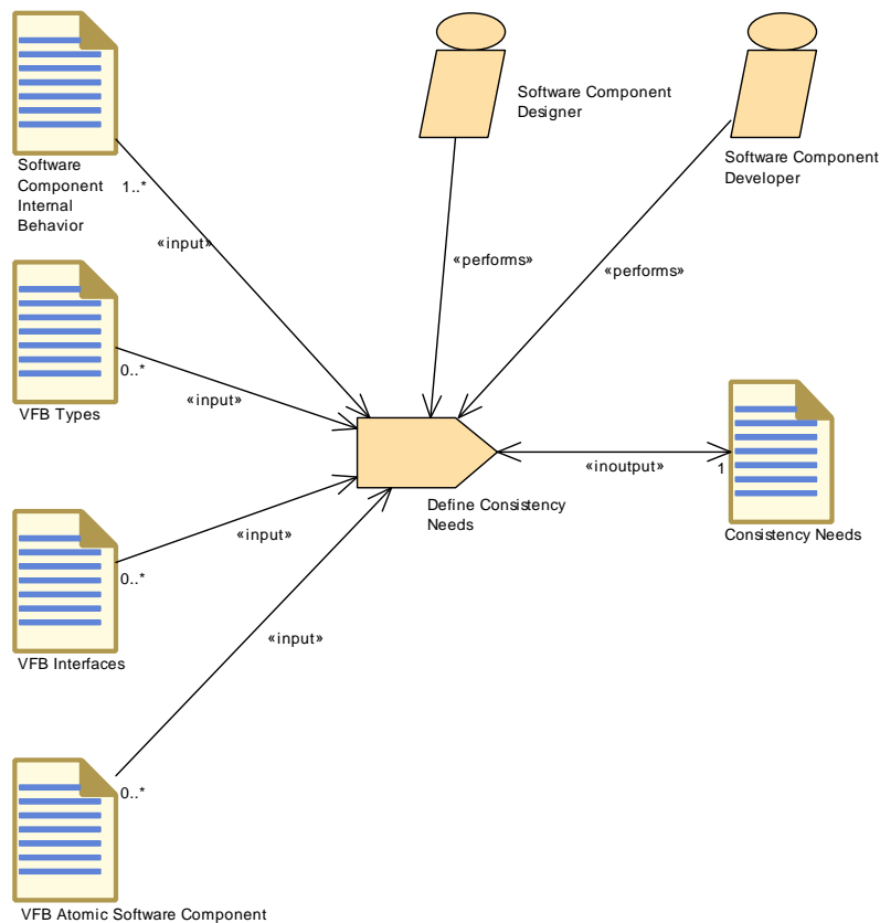
Figure 3.100: Define Consistency Needs
