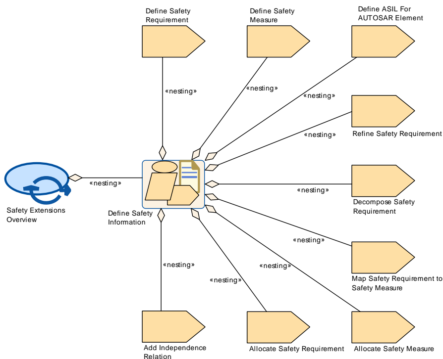
Figure 2.68: Safety Extensions Overview
