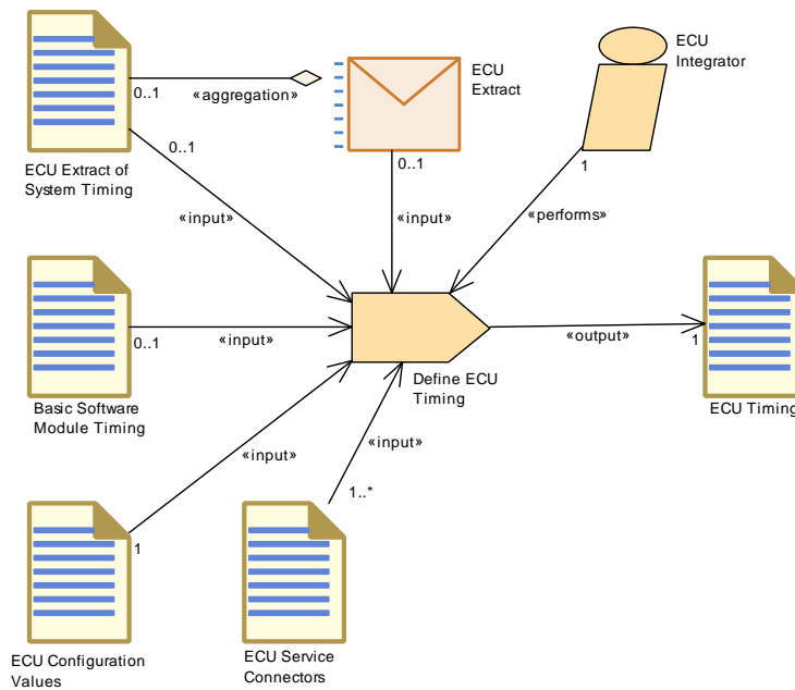
Figure 3.123: Define ECU Timing
