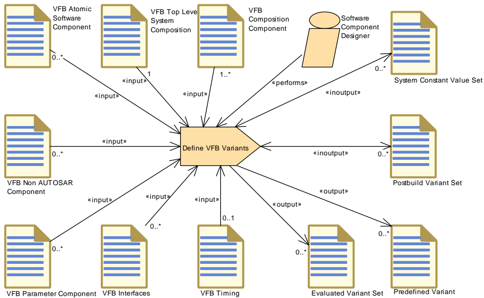
Figure 3.38: Task Define VFB Variants
