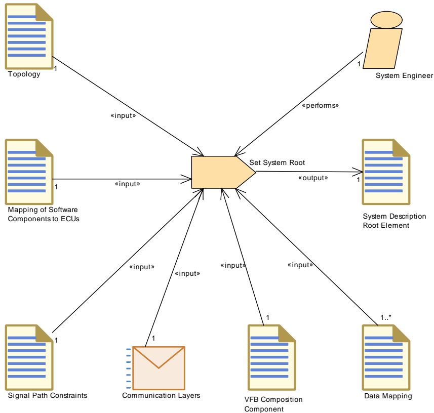
Figure 3.46: Set System Root
