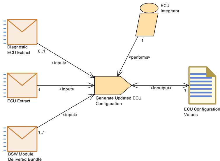
Figure 3.122: Generate Updated ECU Configuration
