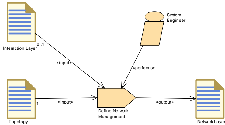
Figure 3.71: Define Network Management
