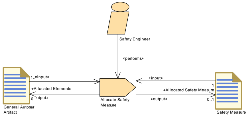
Figure 3.16: Allocate Safety Measure
