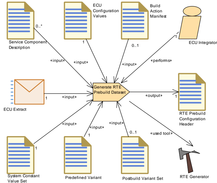
Figure 3.143: Generate RTE Prebuild Dataset
