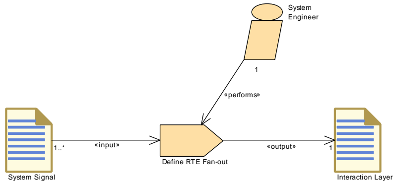
Figure 3.74: Define RTE Fan-out
