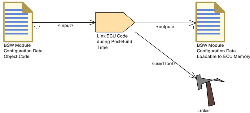
Figure 3.162: Link ECU Code During Post-build Time
