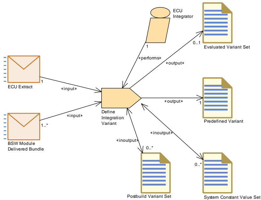
Figure 3.120: Define Integration Variant
