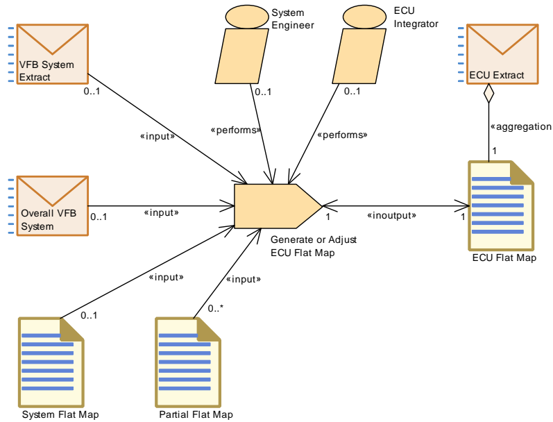
Figure 3.80: Generate or Adjust ECU Flat Map
