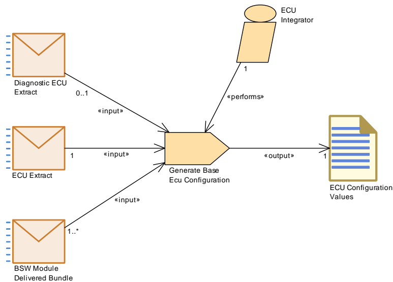
Figure 3.121: Generate Base ECU Configuration
