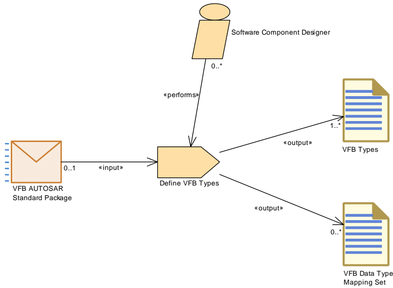
Figure 3.34: Task Define VFB Types
