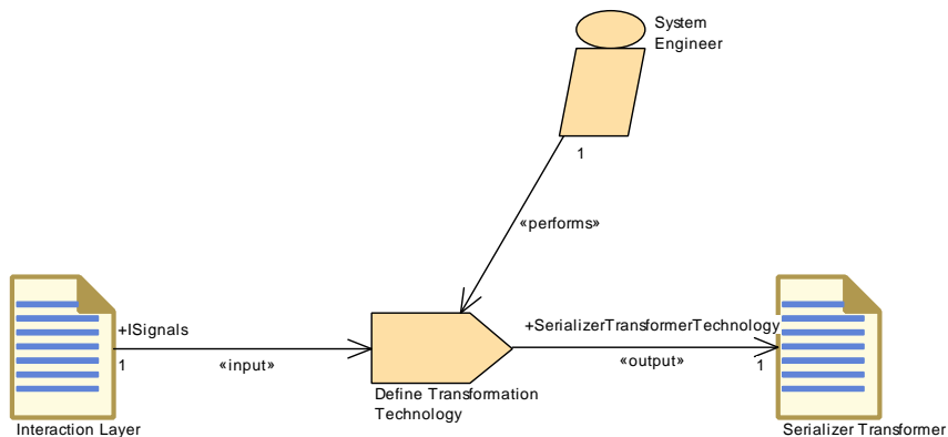
Figure 3.75: Define Transformation Technology
