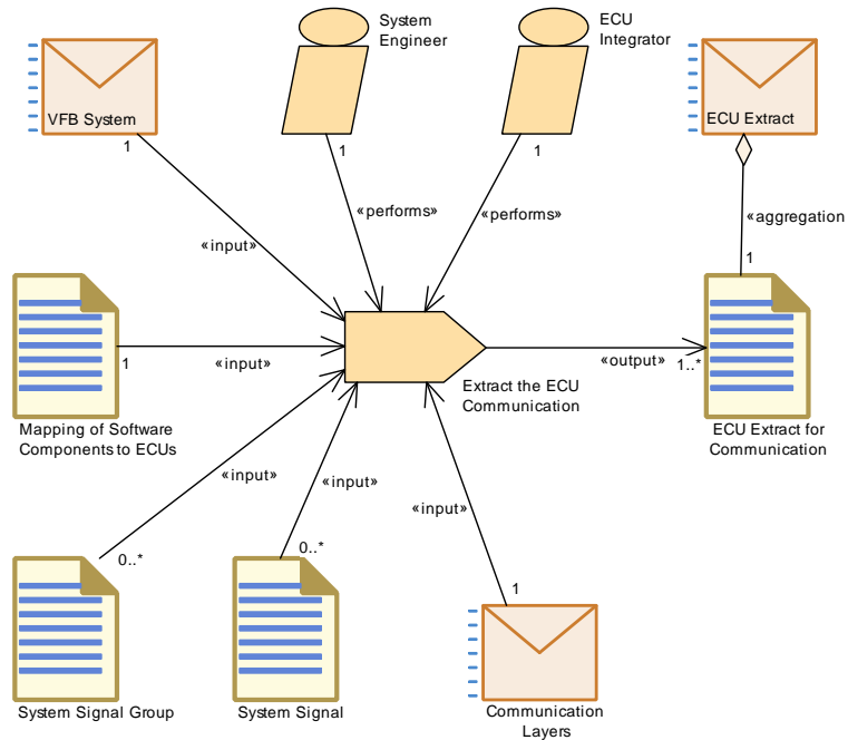
Figure 3.82: Extract the ECU Communication
