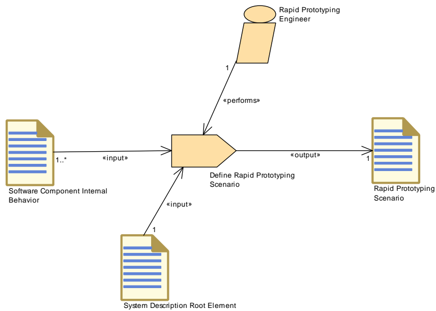
Figure 3.61: Define Rapid Prototyping Scenario
