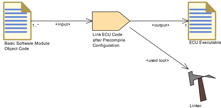
Figure 3.160: Link ECU Code after Precompile Configuration
