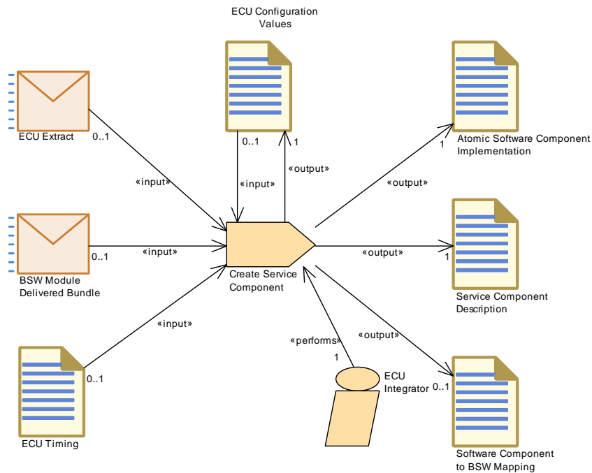
Figure 3.131: Create Service Component
