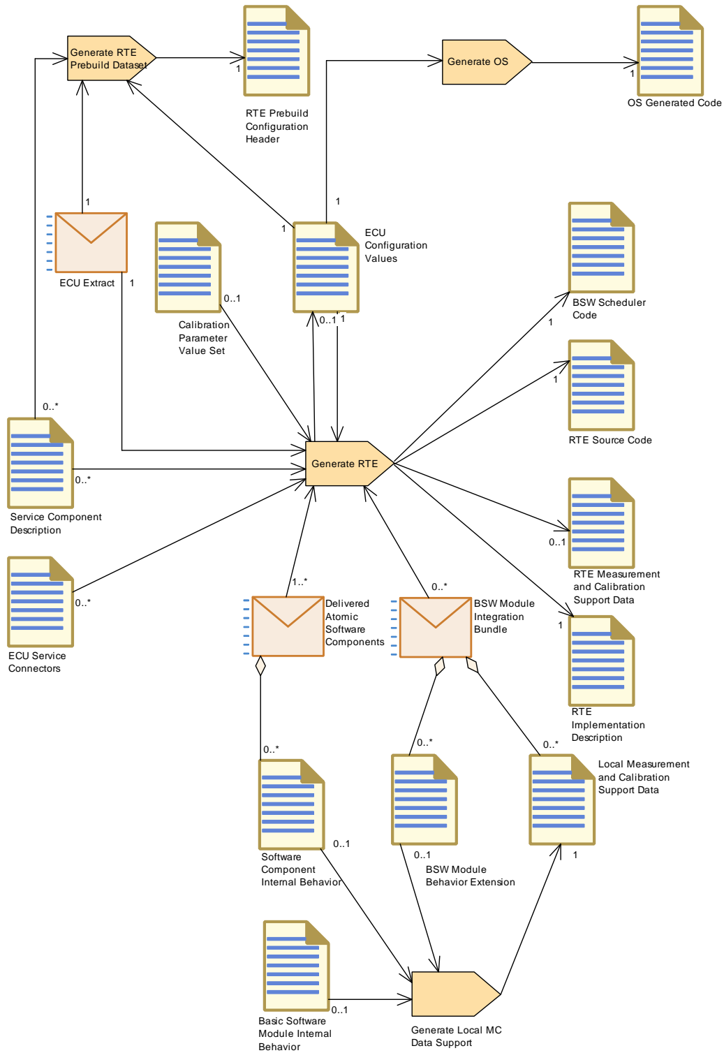
Figure 2.49: Generate BSW and RTE(Part 2)
