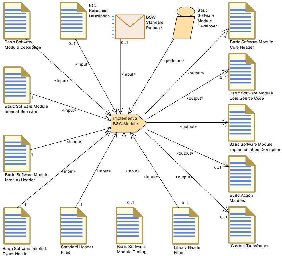
Figure 3.110: Implement a BSW Module
