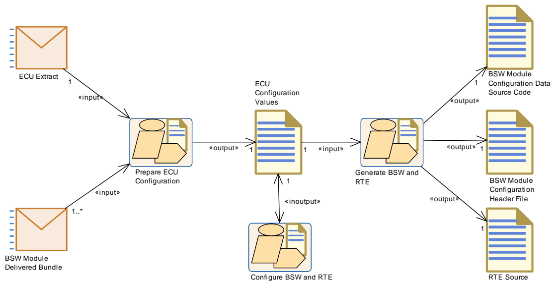
Figure 2.42: ECU Configuration Overview
