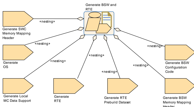
Figure 2.47: Generate BSW and RTE
