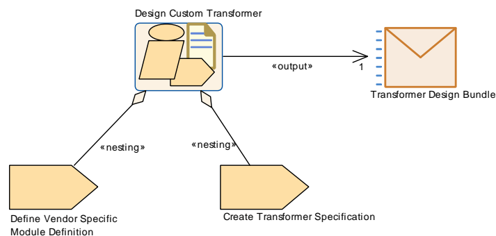
Figure 2.34: Design Custom Transformer activity
