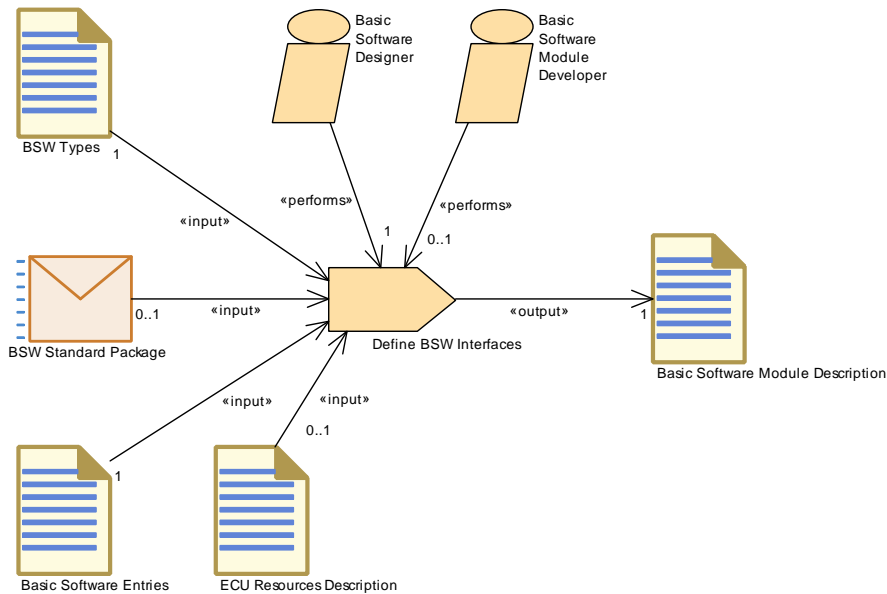
Figure 3.105: Define BSW Interfaces
