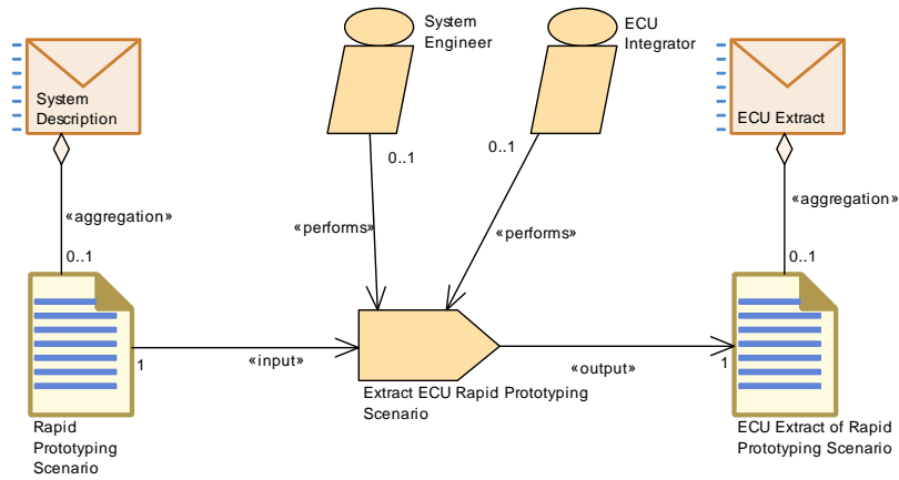
Figure 3.85: Extract ECU Rapid Prototyping Scenario
