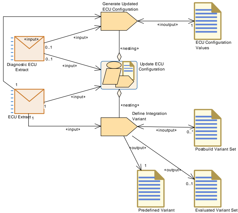
Figure 2.45: Update ECU Configuration
