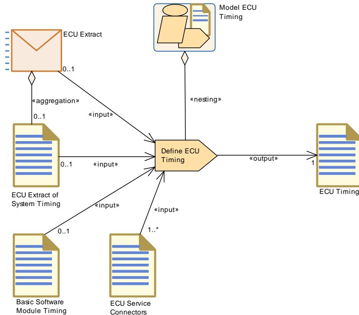
Figure 2.46: Model ECU Timing
