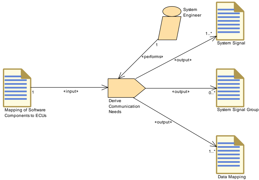
Figure 3.52: Derive Communication Needs
