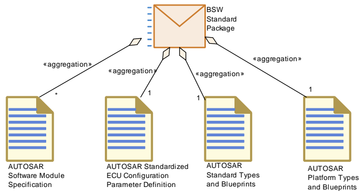
Figure 3.115: BSW Standard Package
