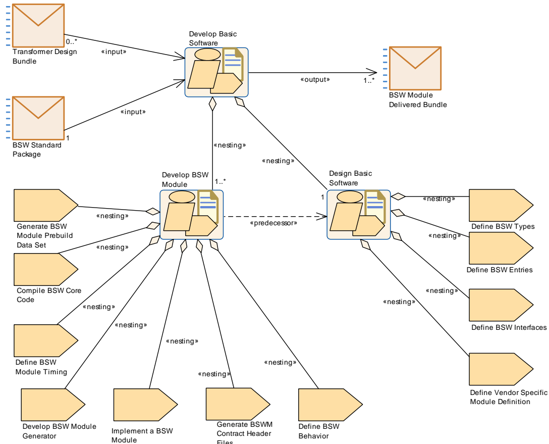
Figure 2.36: Nesting relationship: Develop Basic Software
