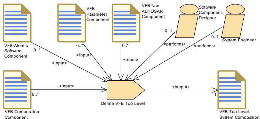
Figure 3.22: Task Define VFB Top Level
