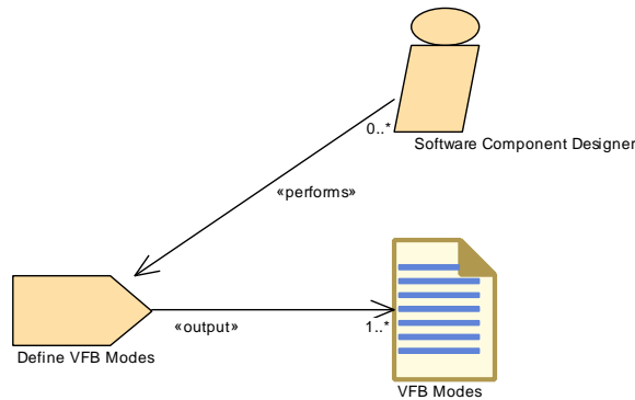
Figure 3.35: Task Define VFB Modes
