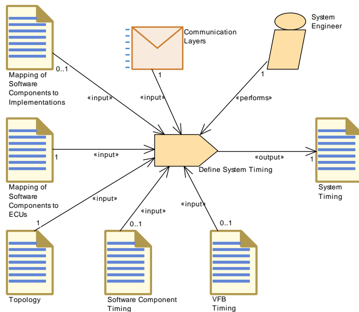
Figure 3.55: Define System Timing
