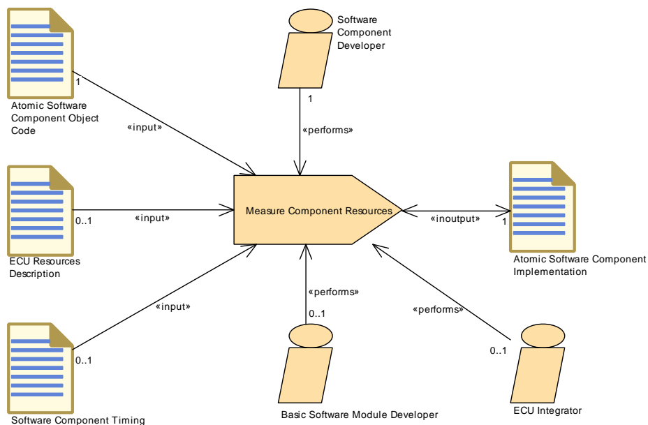
Figure 3.98: Measure Component Resources
