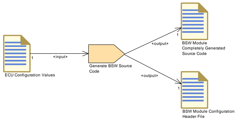
Figure 3.157: Generate BSW Source Code
