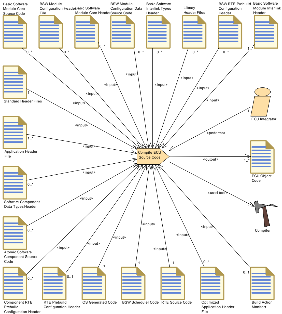
Figure 3.144: Compile ECU Source Code
