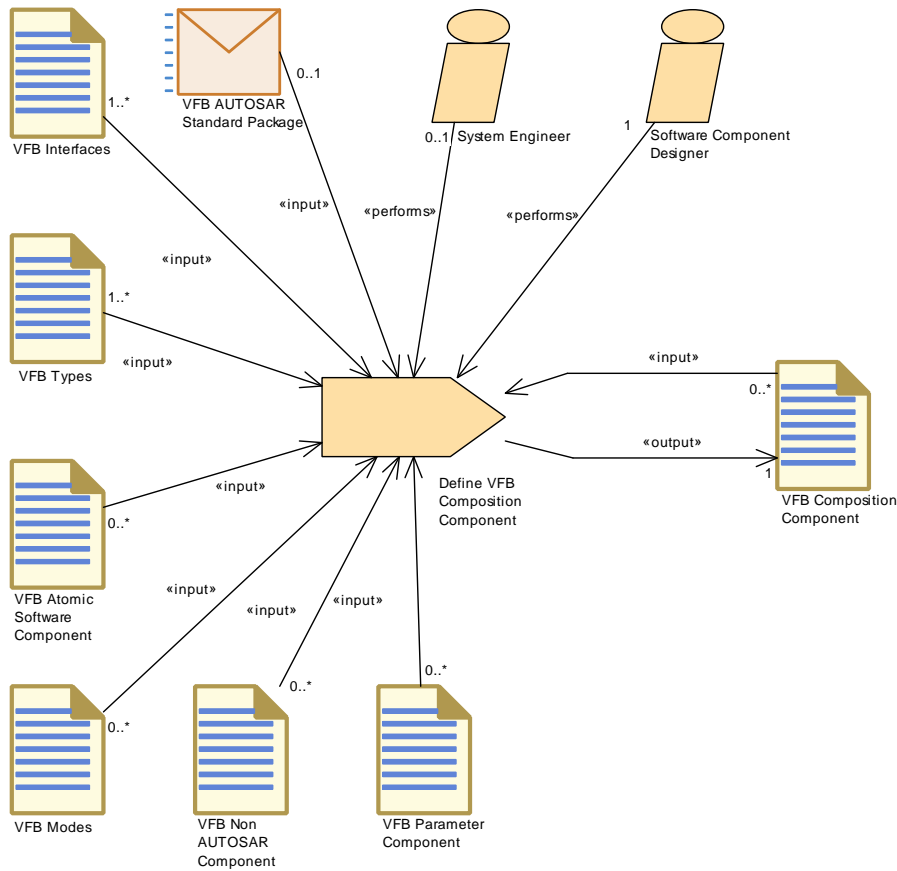
Figure 3.23: Task Define VFB Composition Component
