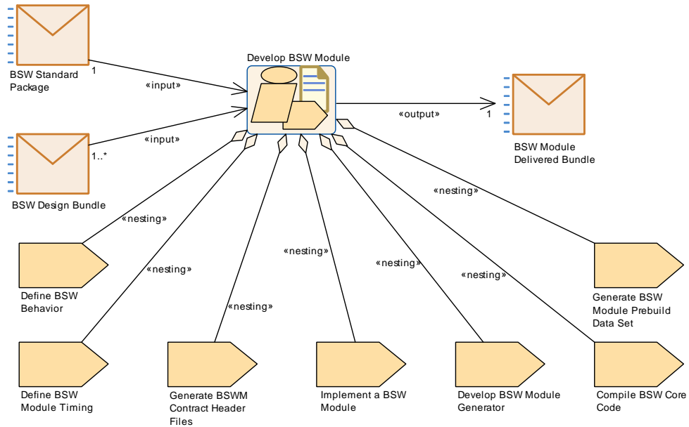
Figure 2.39: Nesting relationship : Develop Basic Software Module
