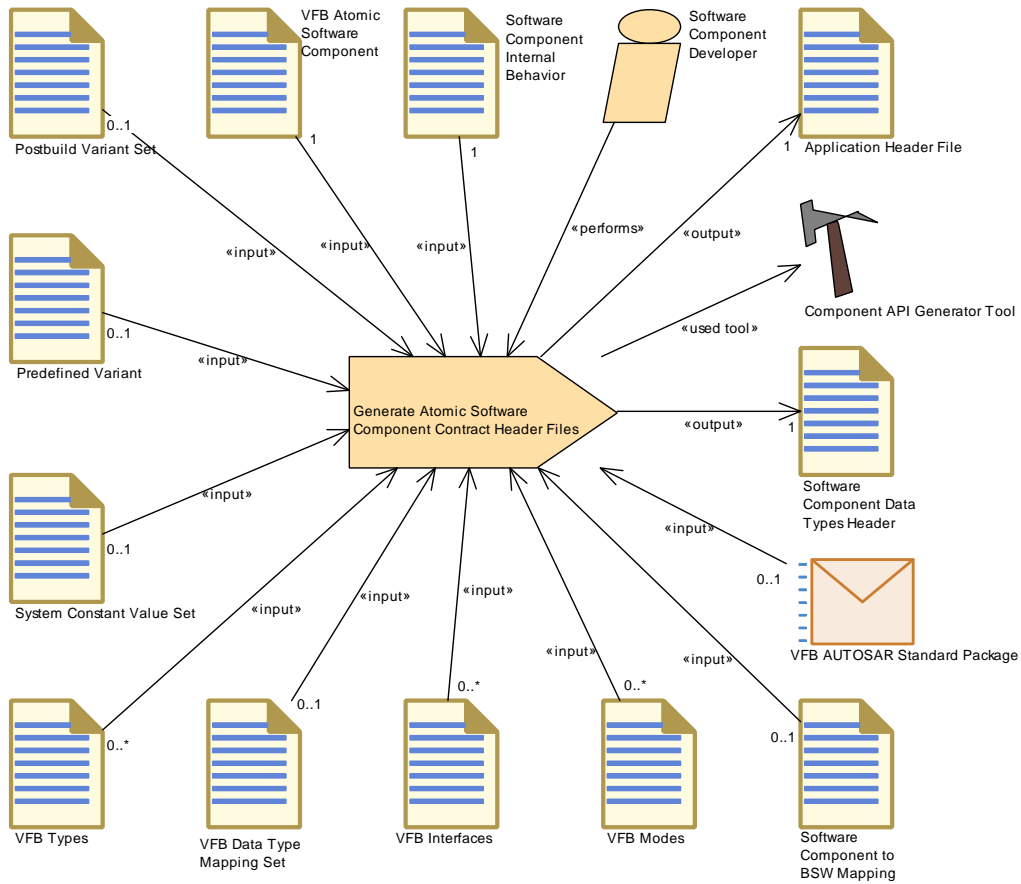
Figure 3.92: Generate Atomic Software Component Contract Header Files
