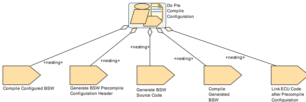
Figure 2.52: Pre compile time configuration activities
