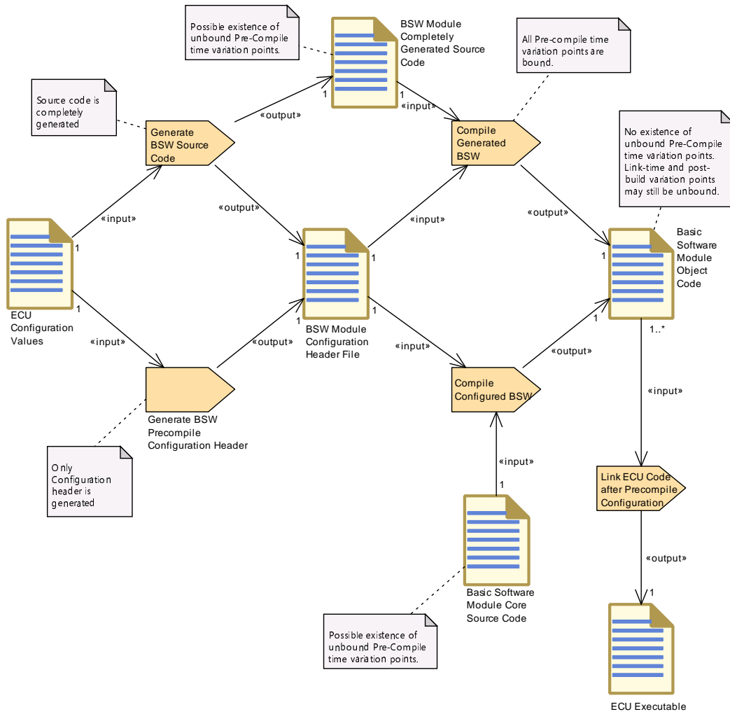
Figure 2.51: Pre-compile time configuration overview
