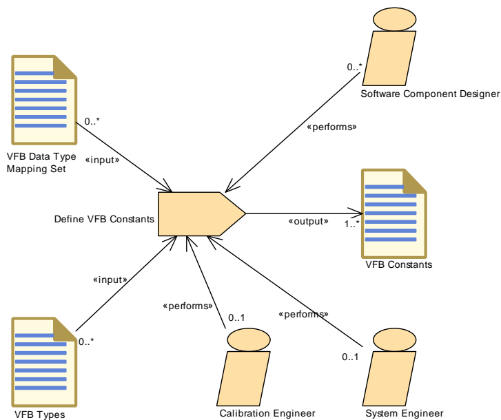
Figure 3.36: Task Define VFB Constants
