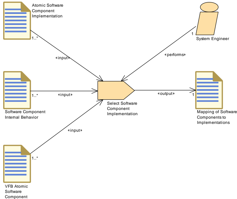
Figure 3.57: Select Software Component Implementation
