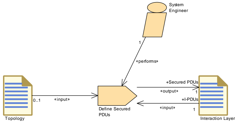
Figure 3.69: Define Secured PDUs
