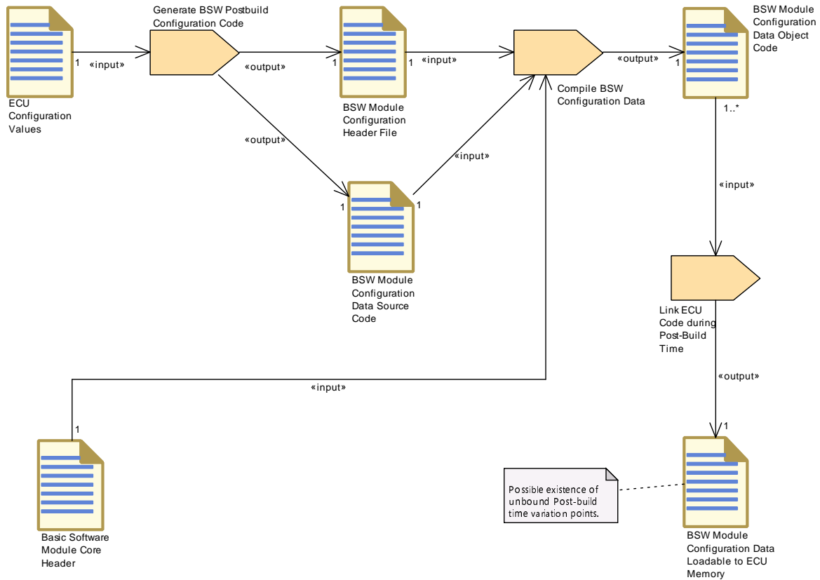
Figure 2.56: Update of the Post-Build Configuration
