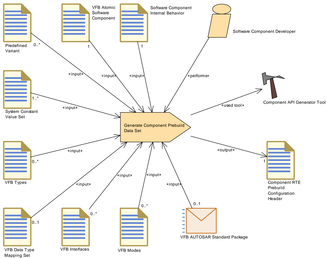
Figure 3.94: Generate Component Prebuild Data Set
