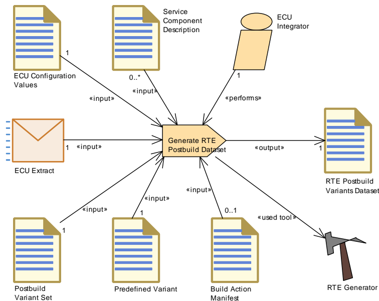
Figure 3.146: Generate RTE Postbuild Dataset
