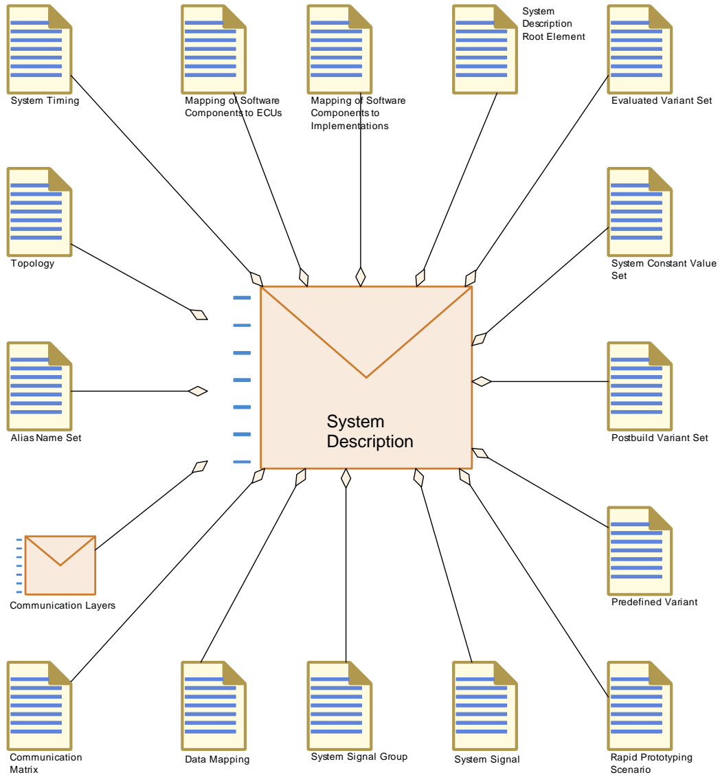
Figure 3.62: Structure of generic deliverable System Description
