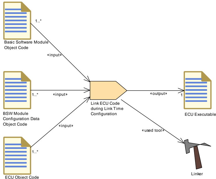
Figure 3.161: Link ECU Code During Link Time Configuration
