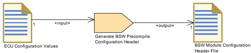
Figure 3.156: Generate BSW Precompile Configuration Header
