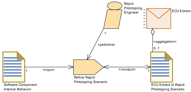
Figure 3.149: Refine Rapid Prototyping Scenario
