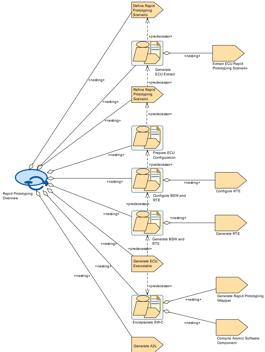
Figure 2.67: Rapid Prototyping Overview
