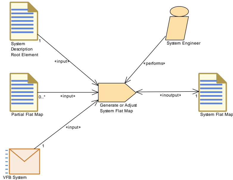
Figure 3.51: Generate or Adjust System Flat Map
