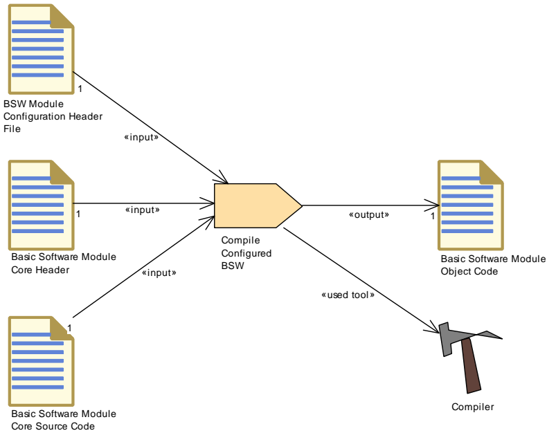
Figure 3.153: Compile Configured Bsw
