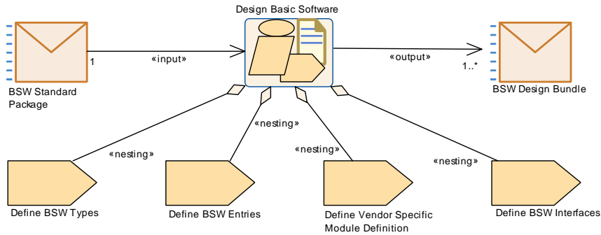
Figure 2.37: Nesting Relationship : Design Basic Software
