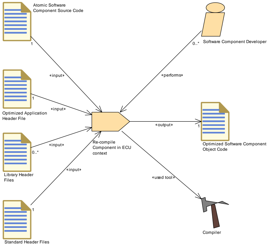
Figure 3.99: Recompile Component in ECU Context
