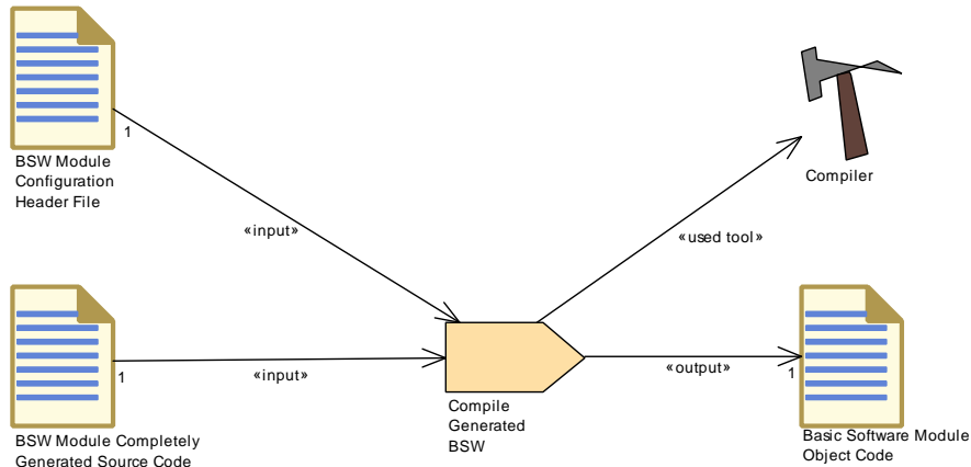
Figure 3.155: Compile Generated BSW
