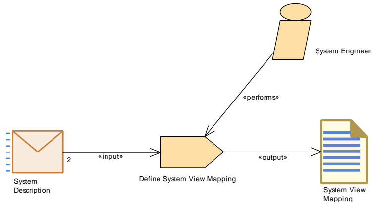
Figure 3.59: Define System View Mapping
