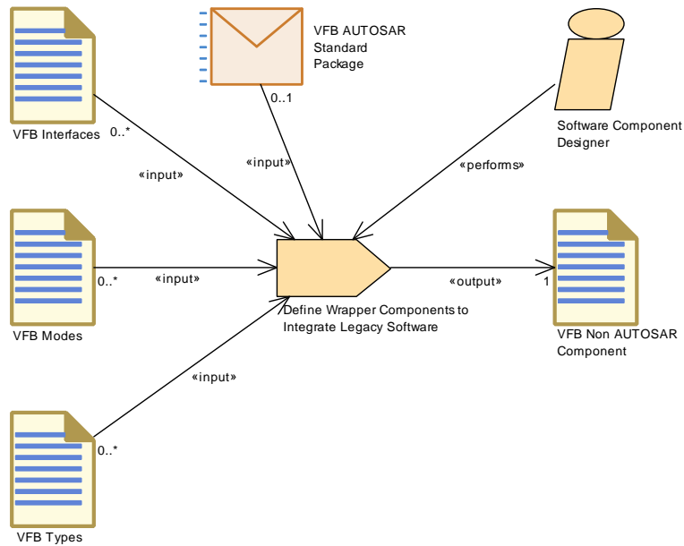
Figure 3.32: Task Define Wrapper Components to Integrate Legacy Software
