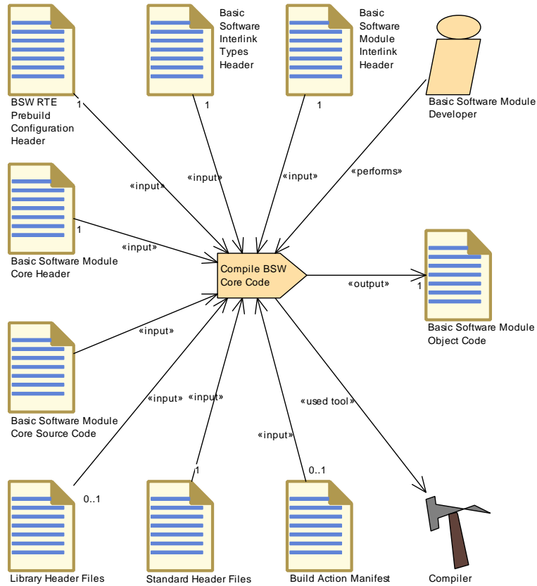
Figure 3.113: Compile BSW Core Code
