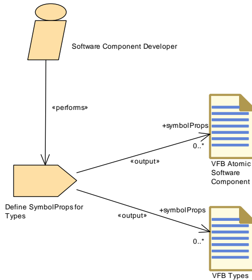
Figure 3.90: Define SymbolProps for Types
