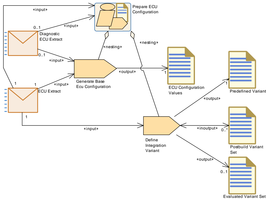
Figure 2.43: Prepare ECU Configuration
