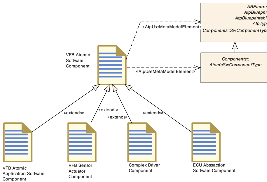
Figure 3.45: The Generic Work Product VFB Atomic Software Component
