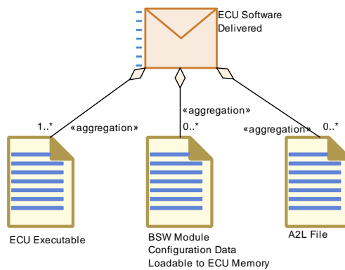
Figure 3.151: ECU Software Delivered
