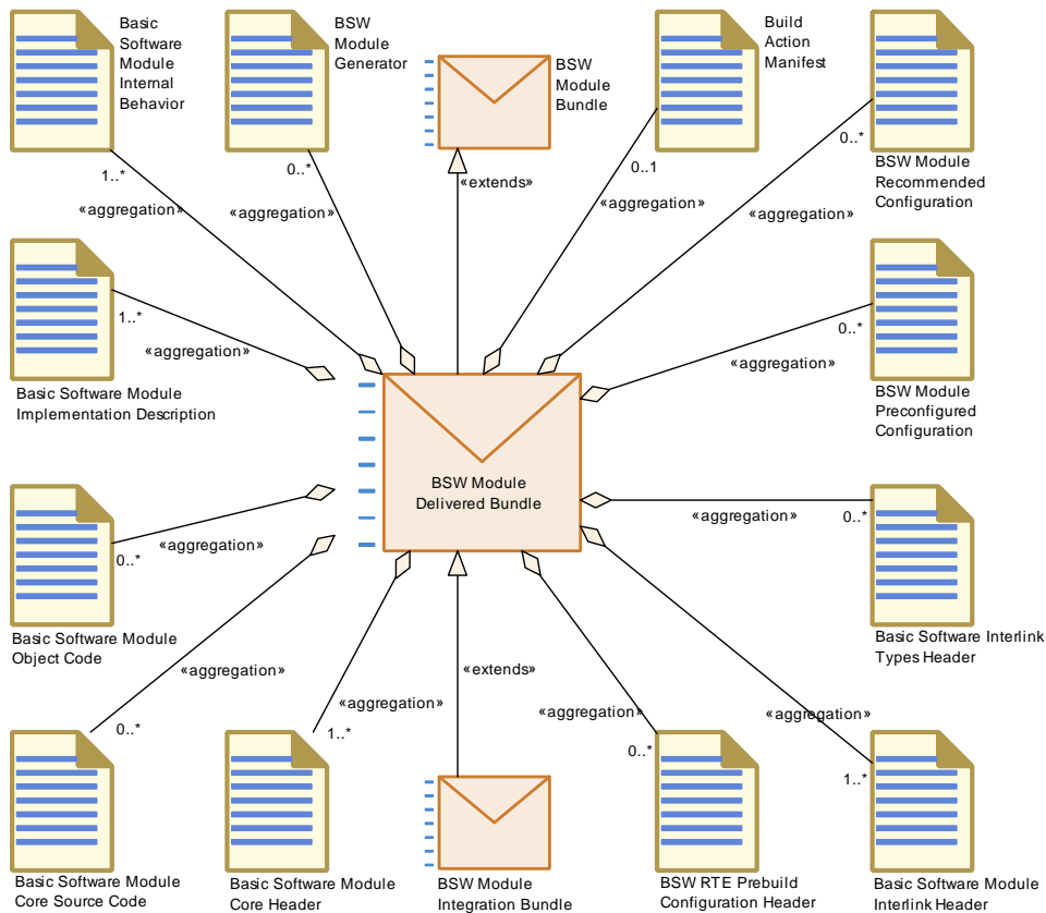
Figure 3.118: BSW Module Delivered Bundle
