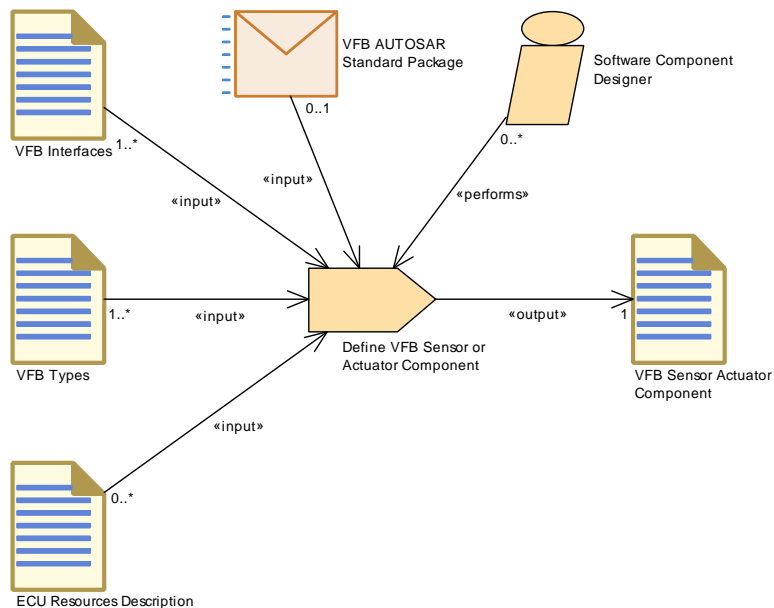
Figure 3.27: Task Define VFB Sensor or Actuator Component
