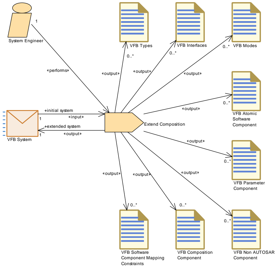
Figure 3.24: Task Extend Composition
