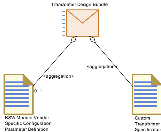
Figure 3.65: Structure of deliverable Transformer Design Bundle
