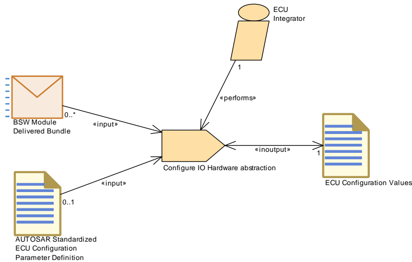
Figure 3.134: Configure IO Hardware Abstraction
