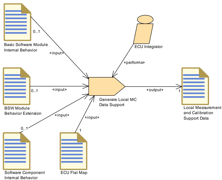
Figure 3.138: Generate Local MC Data Support
