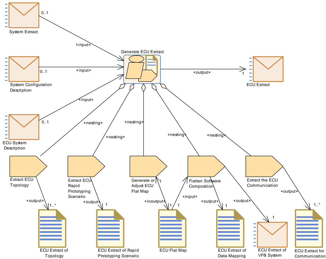
Figure 2.33: Generate the ECU Extract
