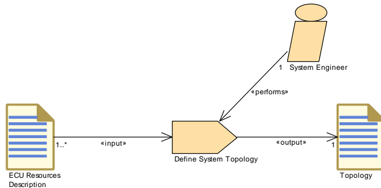
Figure 3.49: Define System Topology
