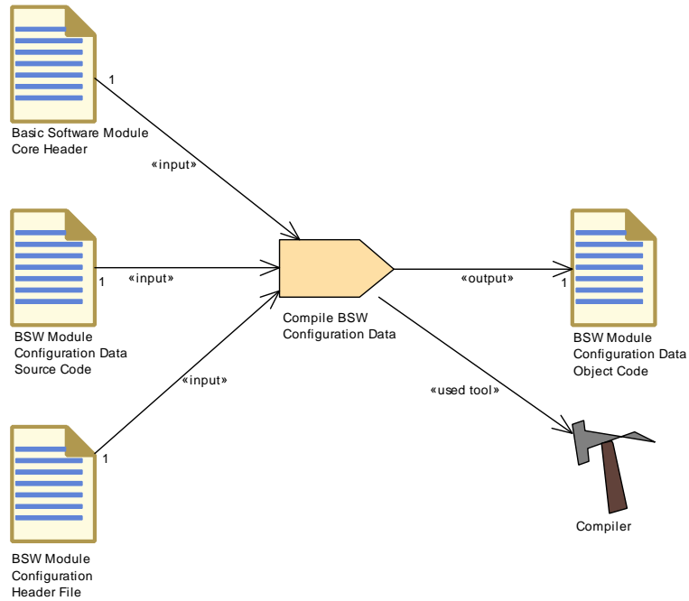
Figure 3.154: Compile BSW Configuration Data
