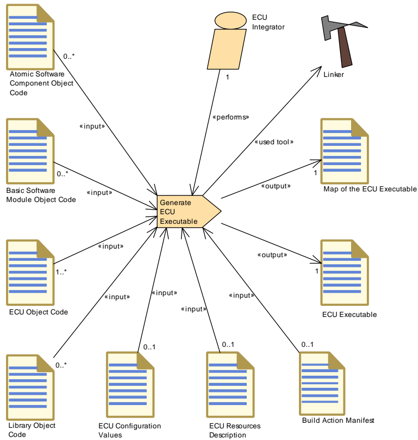
Figure 3.145: Generate ECU Executable
