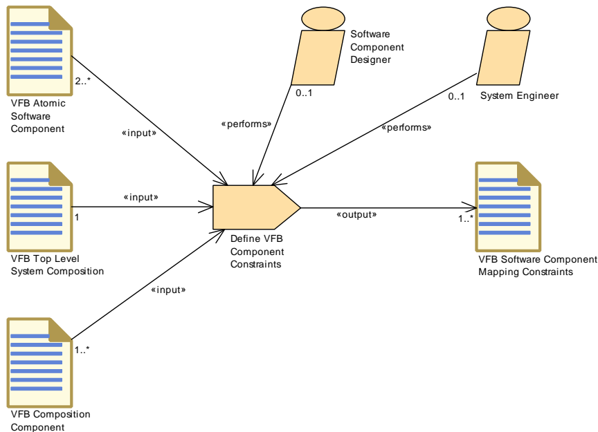
Figure 3.25: Task Define VFB Component Constraints
