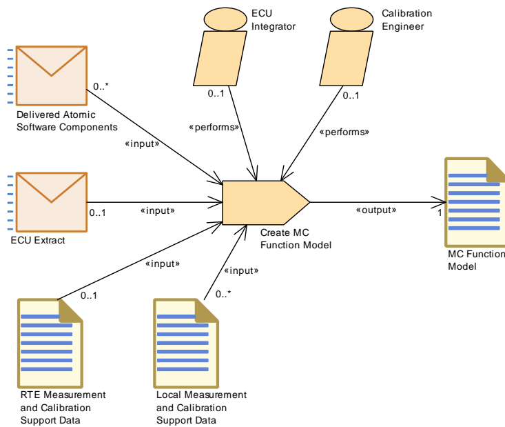
Figure 3.139: Create MC Function Model
