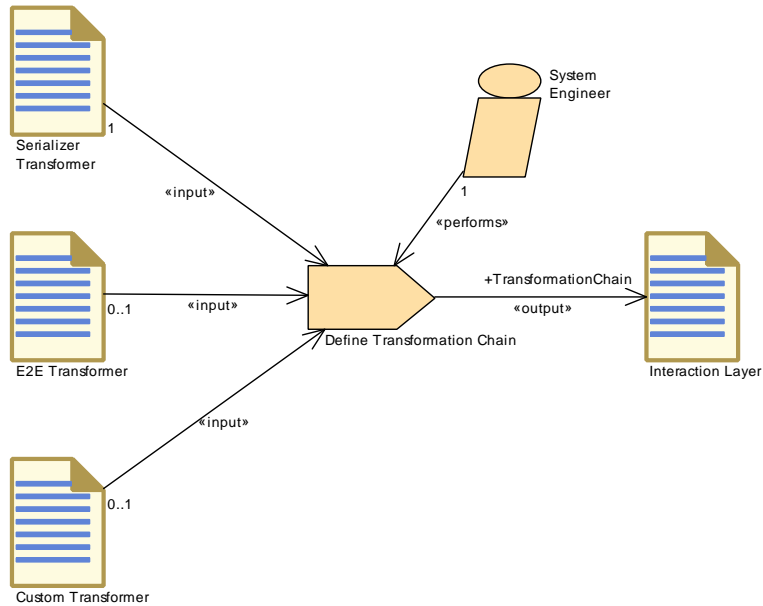
Figure 3.76: Define Transformation Chain
