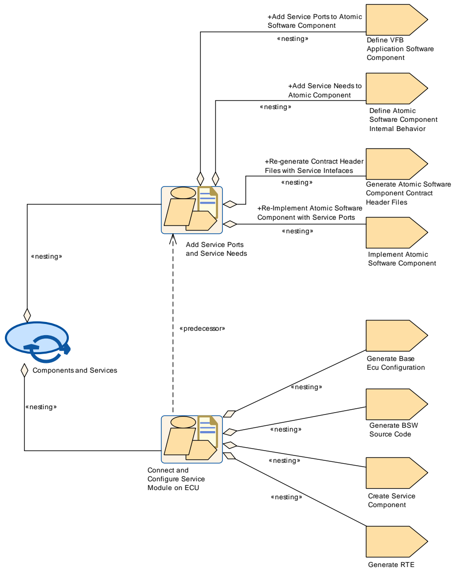
Figure 2.58: Use Case: Components and Services
