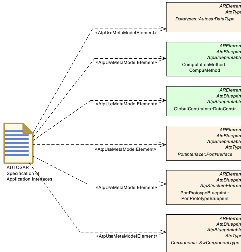
Figure 3.44: The AUTOSAR Specification of Application Interfaces
