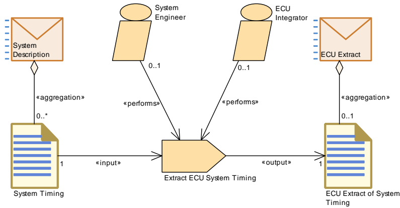
Figure 3.83: Extract the ECU System Timing Model
