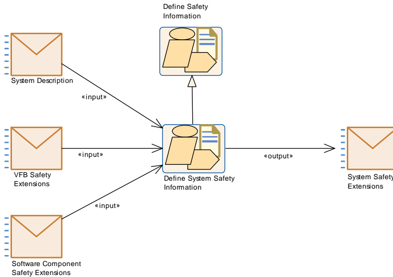
Figure 2.35: Define System Safety Information
