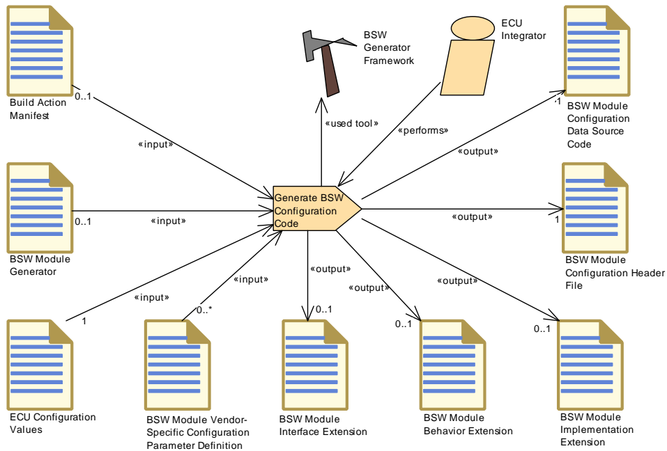
Figure 3.137: Generate BSW Code and model extensions
