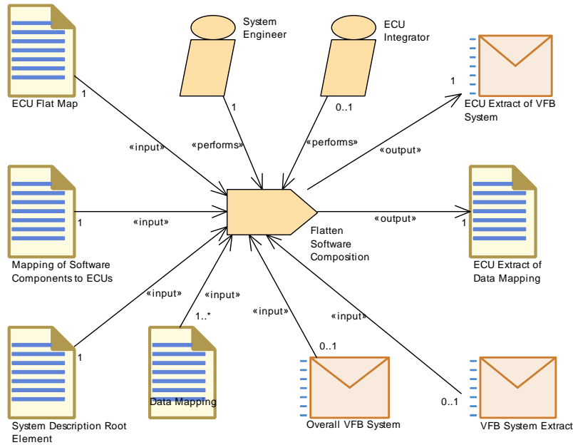
Figure 3.81: Flatten Software Composition
