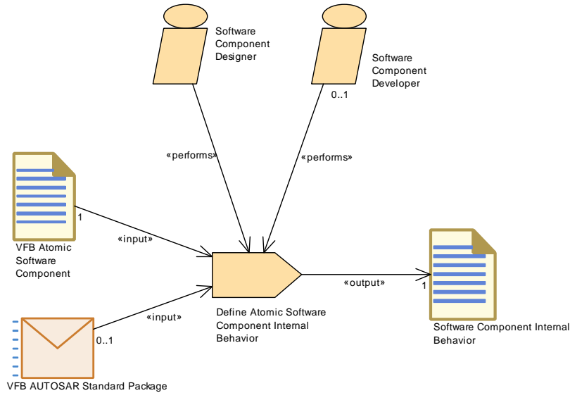
Figure 3.87: Define Software Component Internal Behavior
