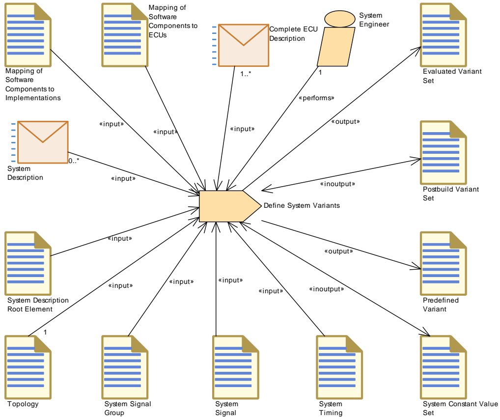
Figure 3.54: Define System Variants
