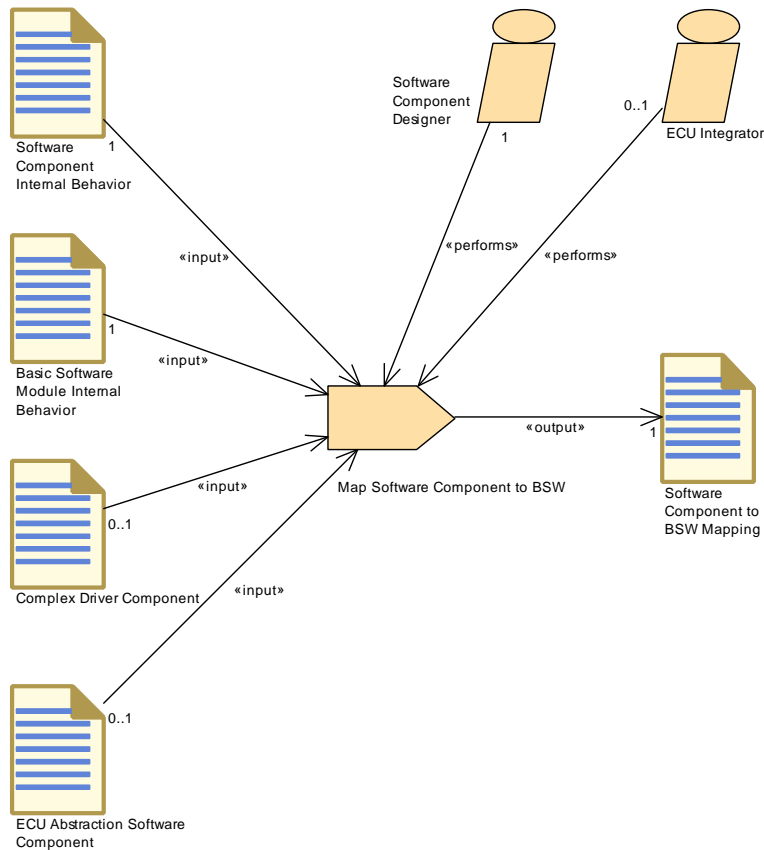
Figure 3.97: Map Software Component to BSW
