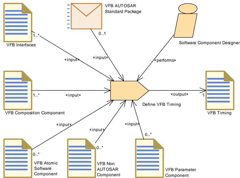
Figure 3.37: Task Define VFB Timing
