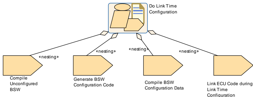
Figure 2.54: Link time configuration
