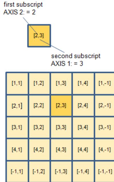
Figure 3.14: Matrix Representation
