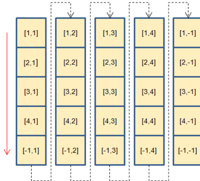
Figure 3.15: Transformation Matrix in column-major order
