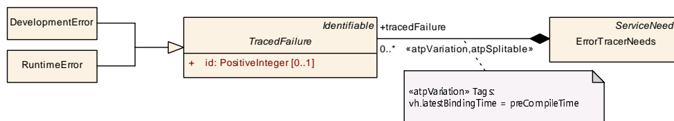
Figure 12.6: Modeling of ErrorTracerNeeds
