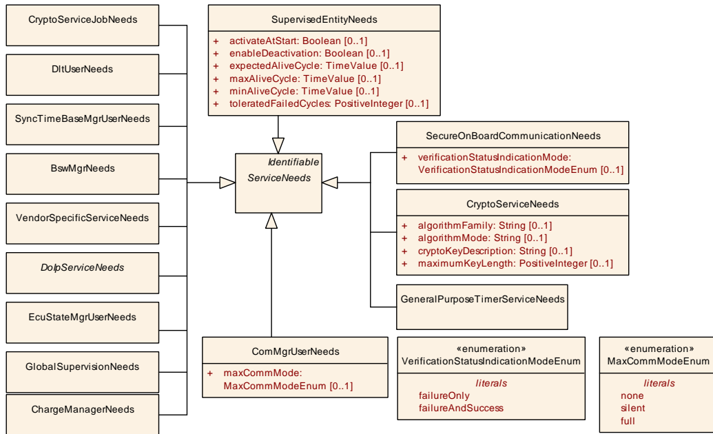
Figure 12.3: Class ServiceNeeds from CommonStructure and some derived classes
