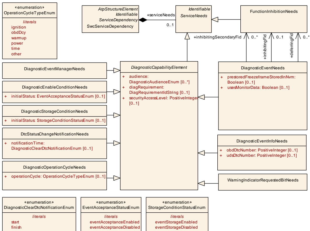
Figure 12.5: Class ServiceNeeds from CommonStructure and derived classes for diagnosis use cases
