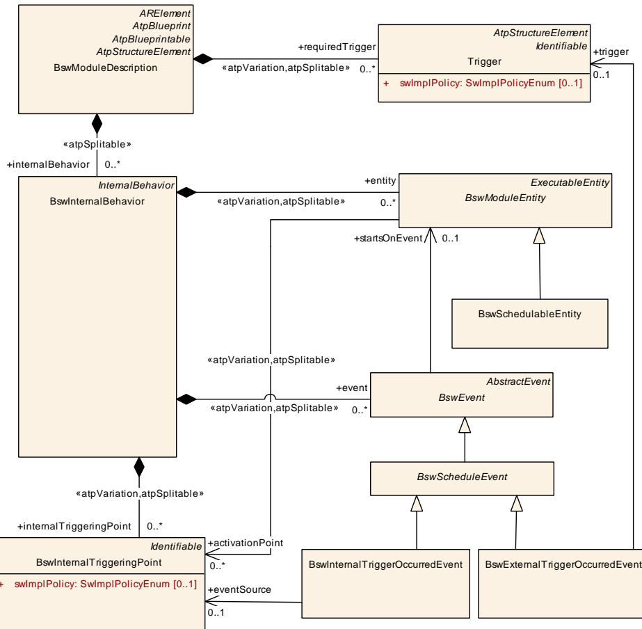
Figure 5.8: Details on BSW Trigger Events
