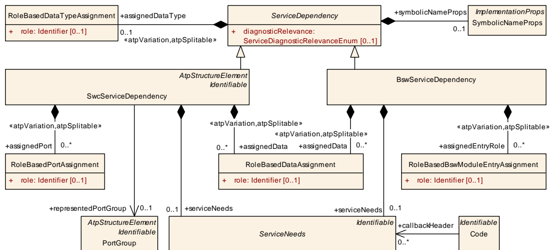
Figure 12.1: Concept of ServiceDependency for BSW and SWC
