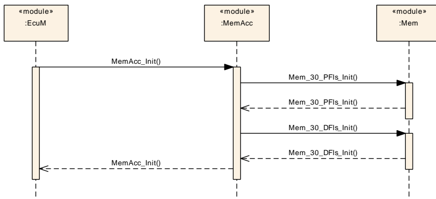
Figure 9.3: Mem Driver Initialization by MemAcc
