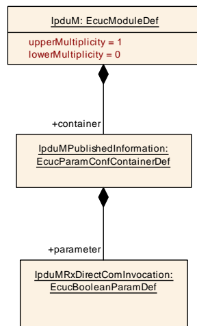
Figure 10.10: IpduMPublishedInformation
