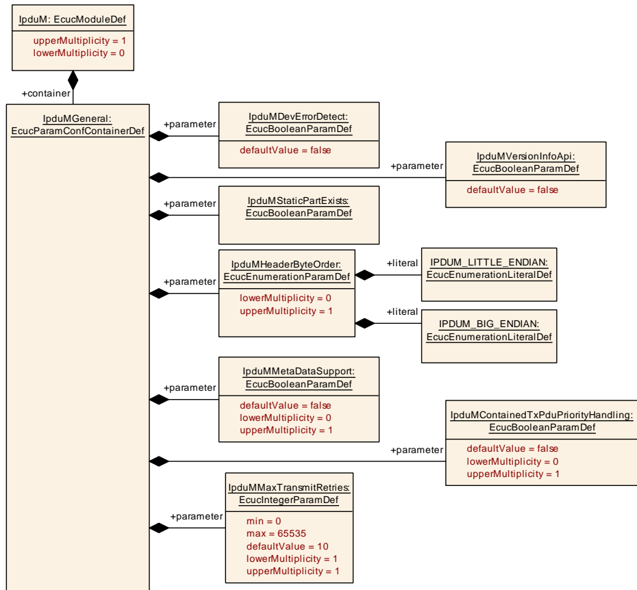
Figure 10.3: IpduMGeneral
