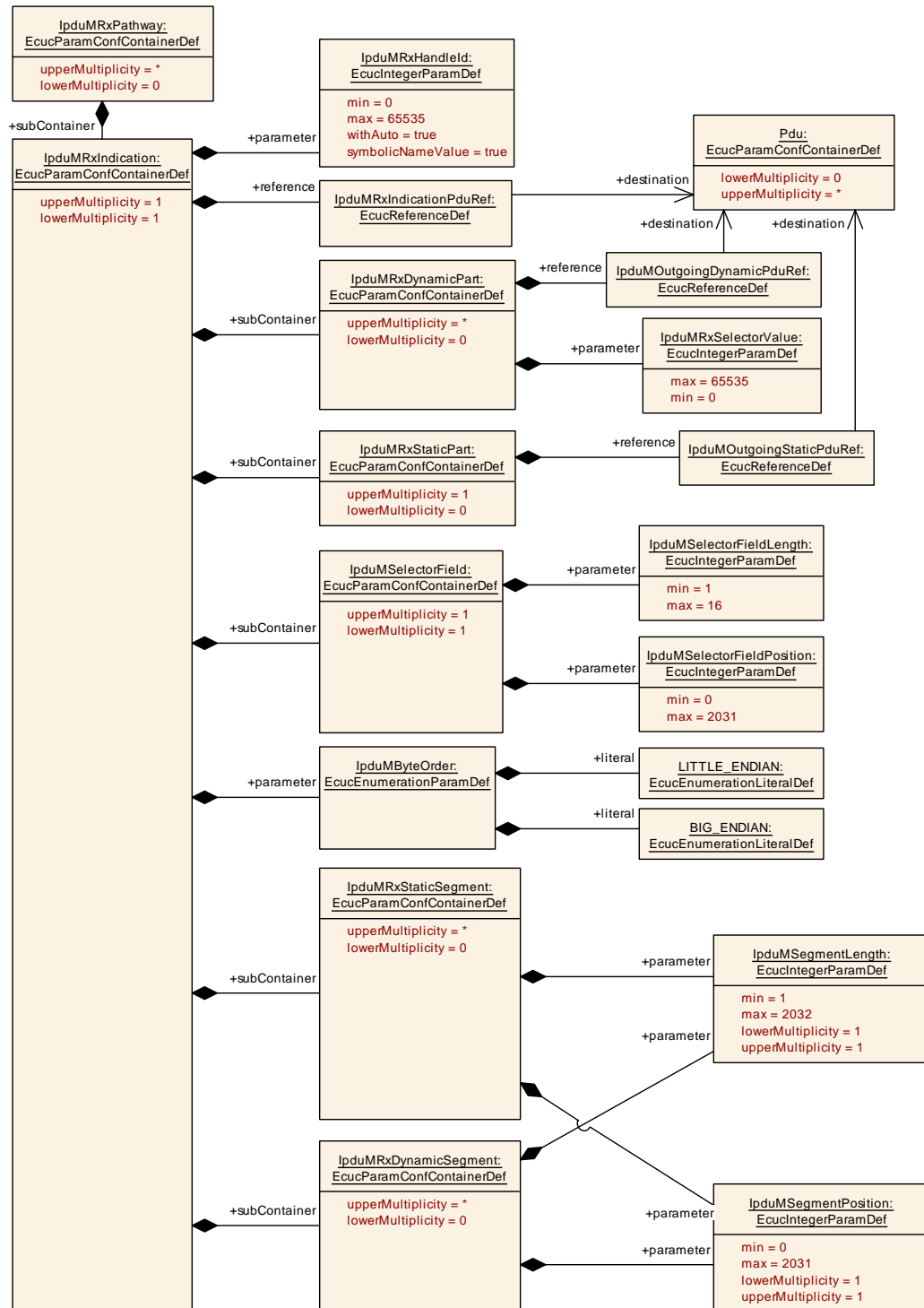
Figure 10.6: IpduMRxPathwayIndication
