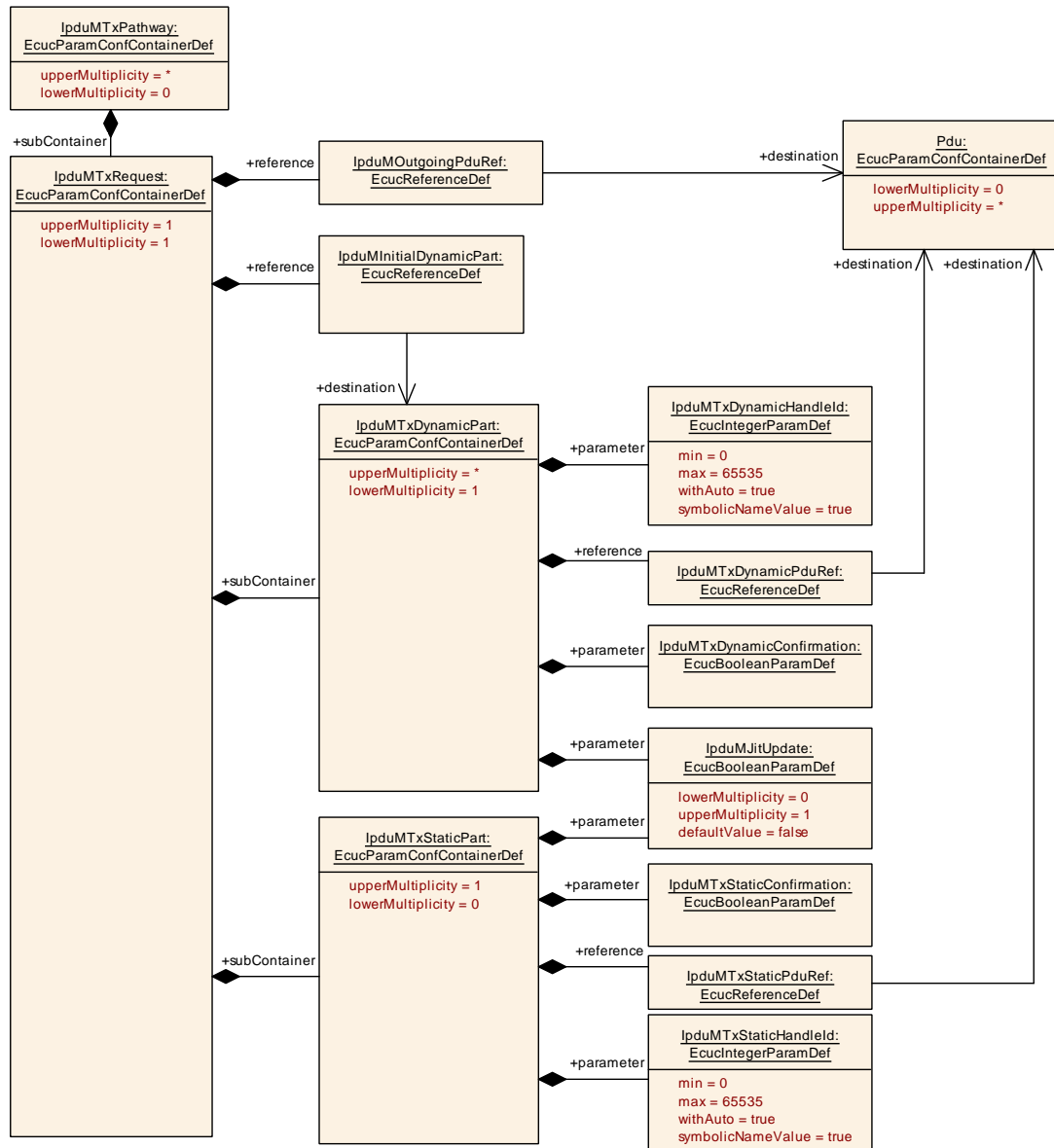
Figure 10.5: IpduMTxPathwayRequest part 2
