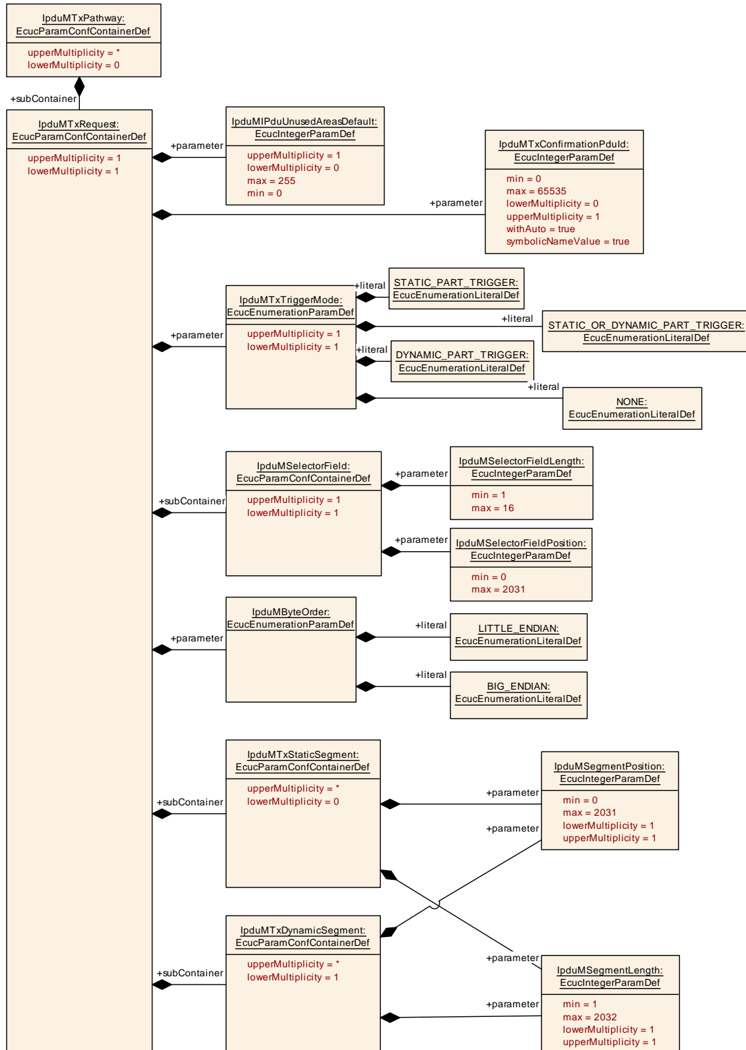
Figure 10.4: IpduMTxPathwayRequest part 1
