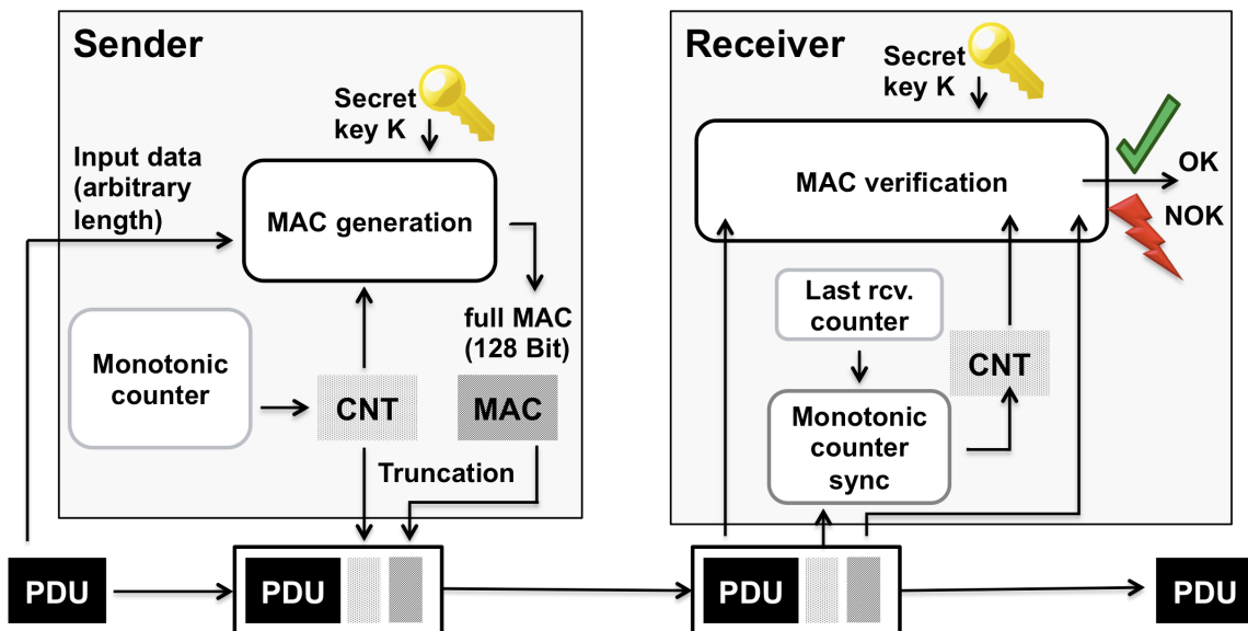
Figure 4.1: Message Authentication and Freshness Verification
