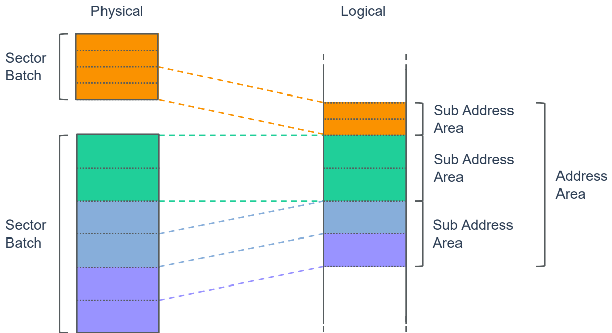
Figure 6.1: Overview of Address Translation/Mapping
