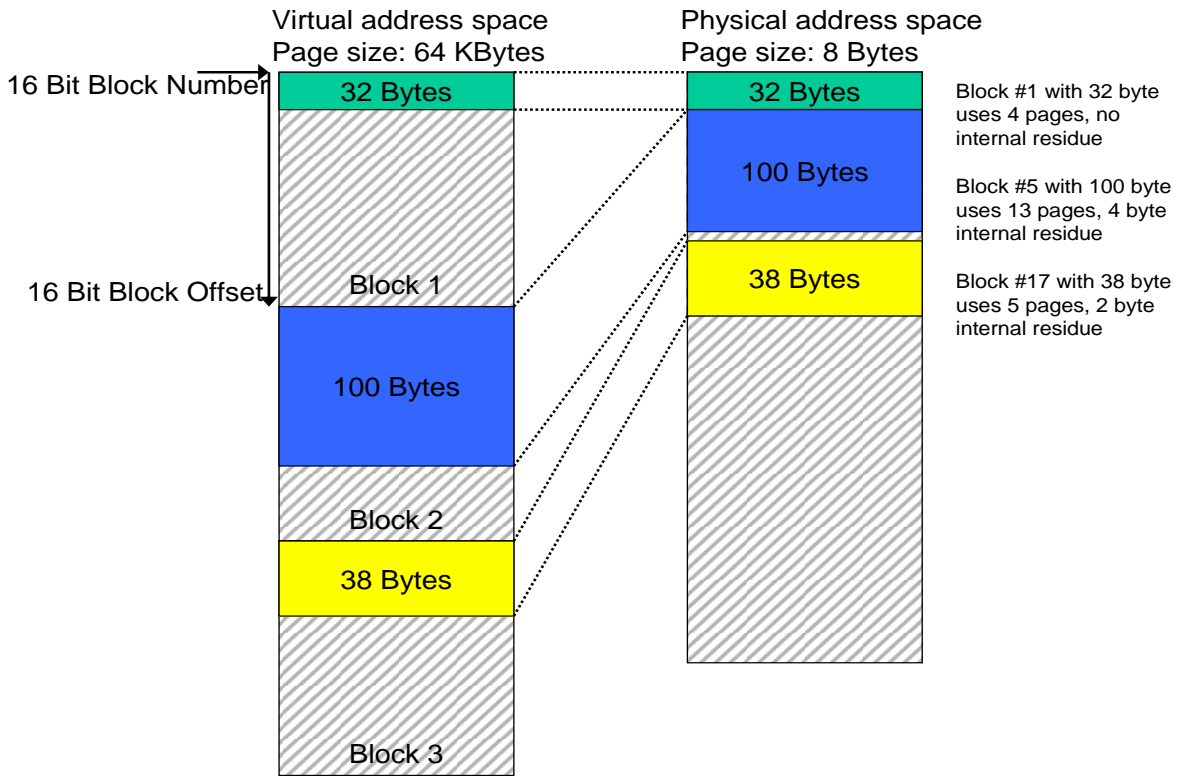
Figure 6.2: Virtual vs. physical address space
