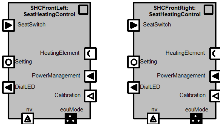
Figure 3.3: Example showing the multiple instantiation of the component "SeatHeating Control" as "SHCFrontLeft" and "SHCFrontRight"
