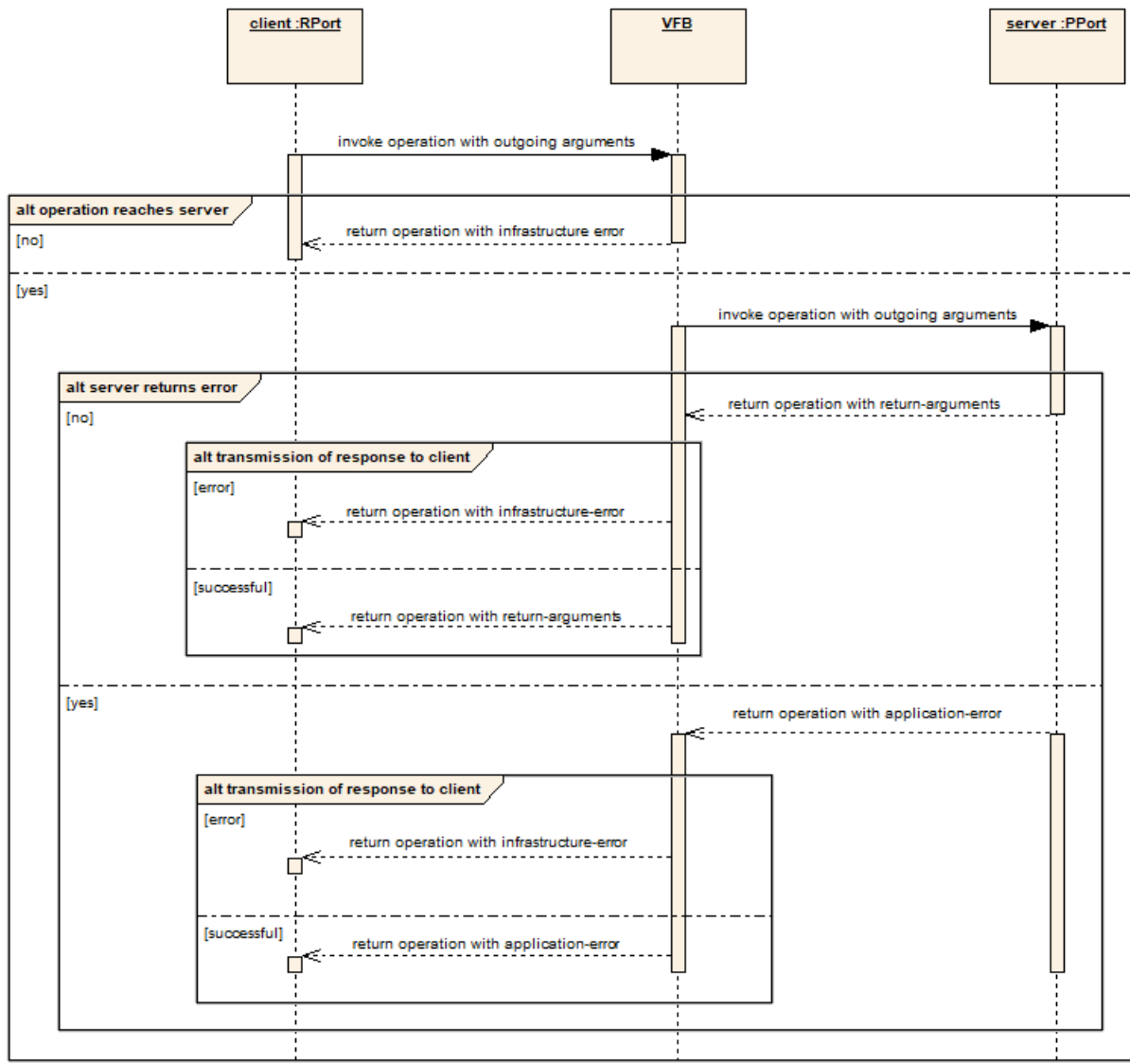
Figure 4.6: Client-server on the VFB (synchronous and asynchronous)
