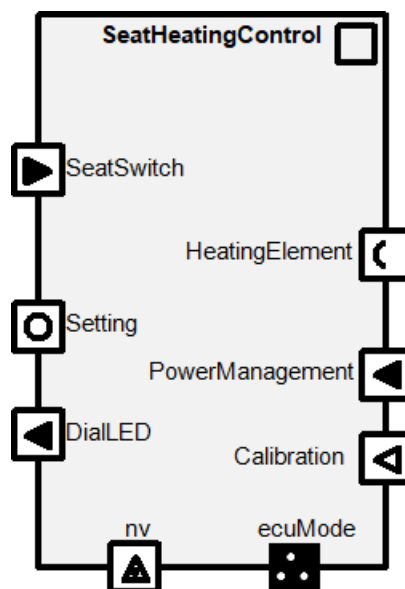
Figure 3.1: Example of the definition of the component-type "SeatHeatingControl" with eight ports
