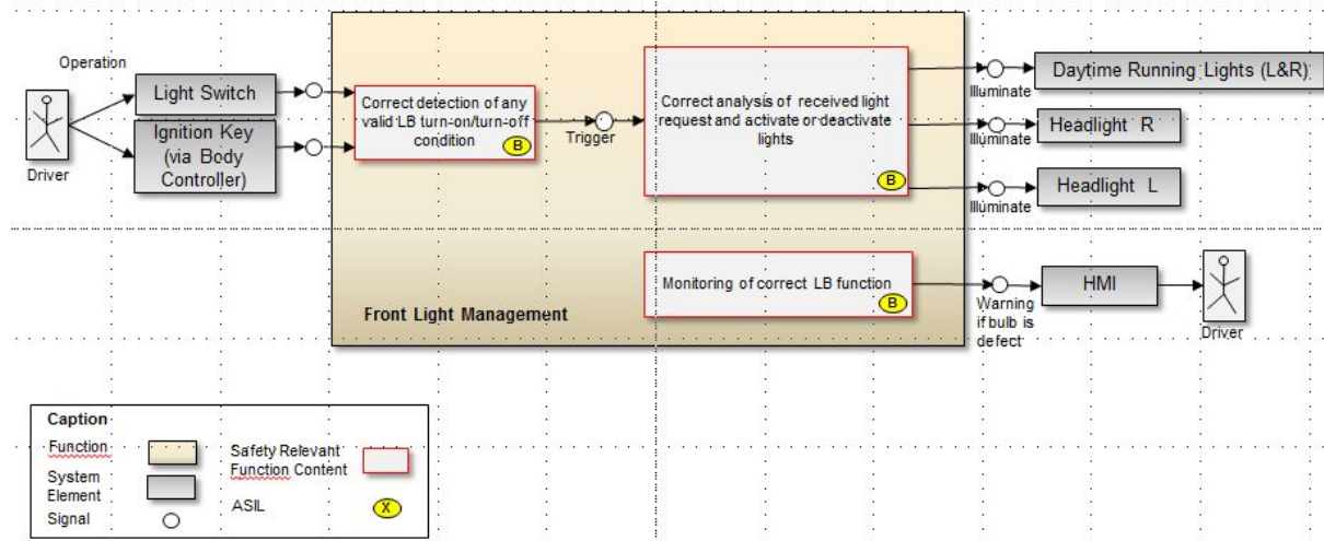
Figure 3.1: Functional Safety Architecture
