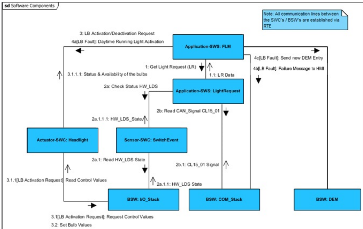
Figure 5.3: SWC Communication-Diagram via RTE
