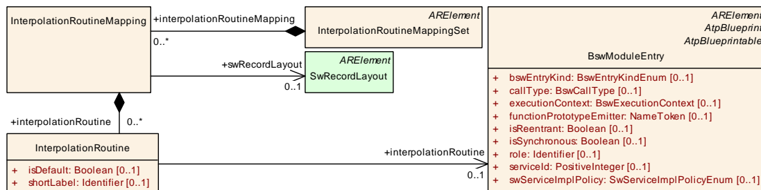
Figure 7.5: Mapping of Record Layouts and Interpolation Routines
