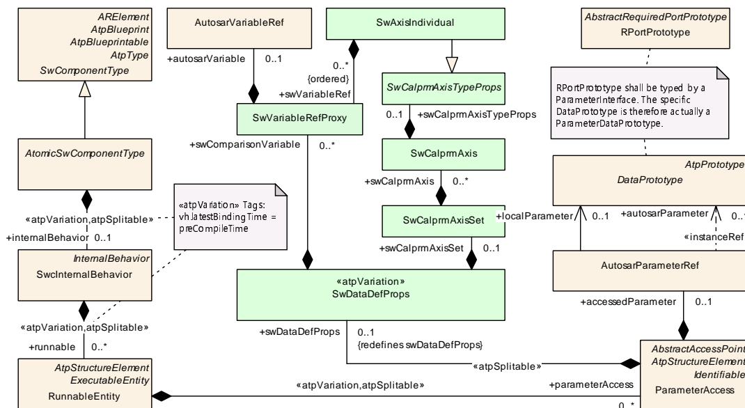
Figure 7.8: Runnable Access to a Calibration Port
