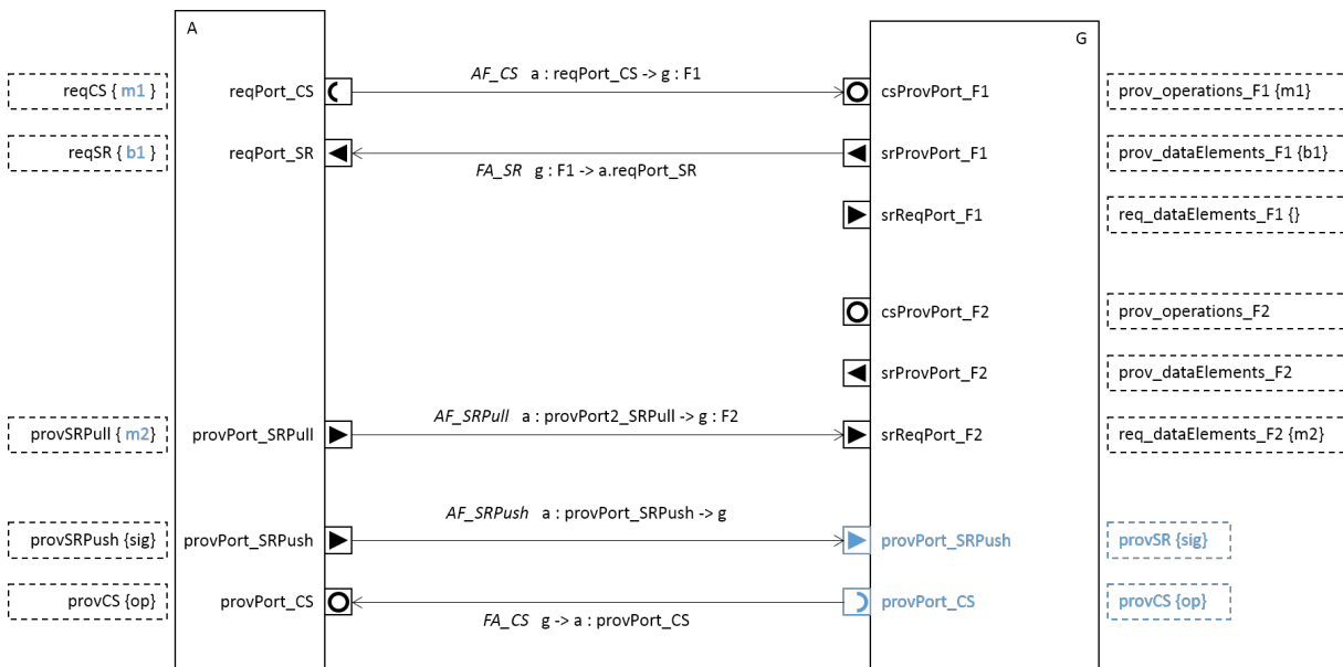
Figure 3.1: Translation of Franca links to AUTOSAR
