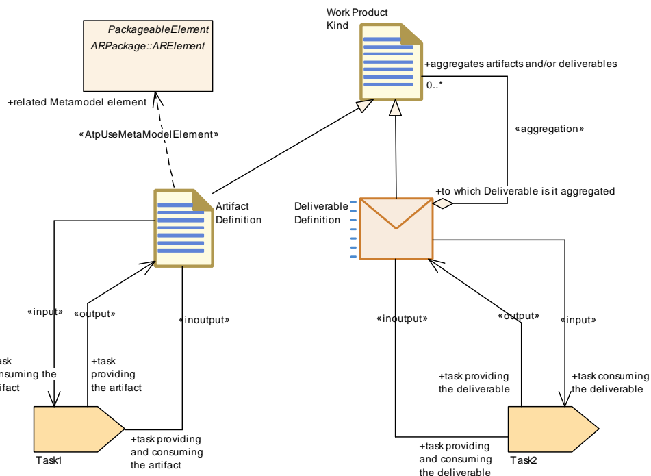
Figure 1.3: Work Product Definition Overview
