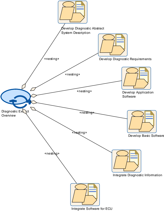
Figure 2.66: Diagnostic Extract Overview
