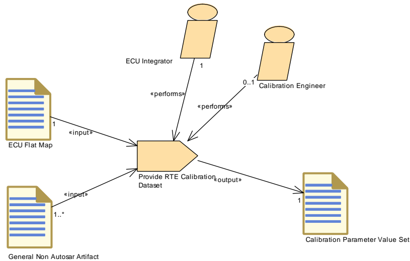
Figure 3.121: Provide RTE Calibration Dataset
