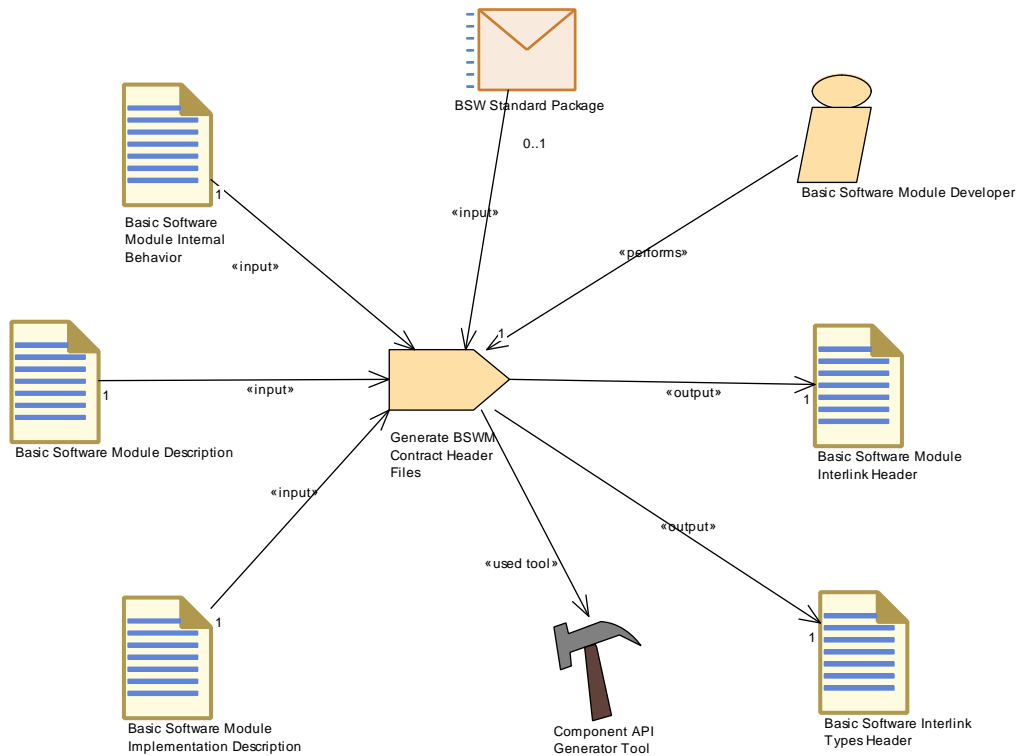
Figure 3.111: Generate BSW Contract Header Files
