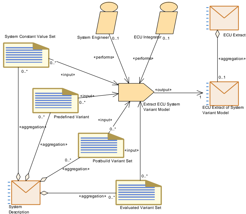
Figure 3.86: Extract the ECU System Variant Model
