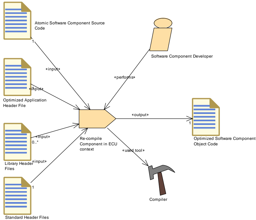
Figure 3.101: Recompile Component in ECU Context
