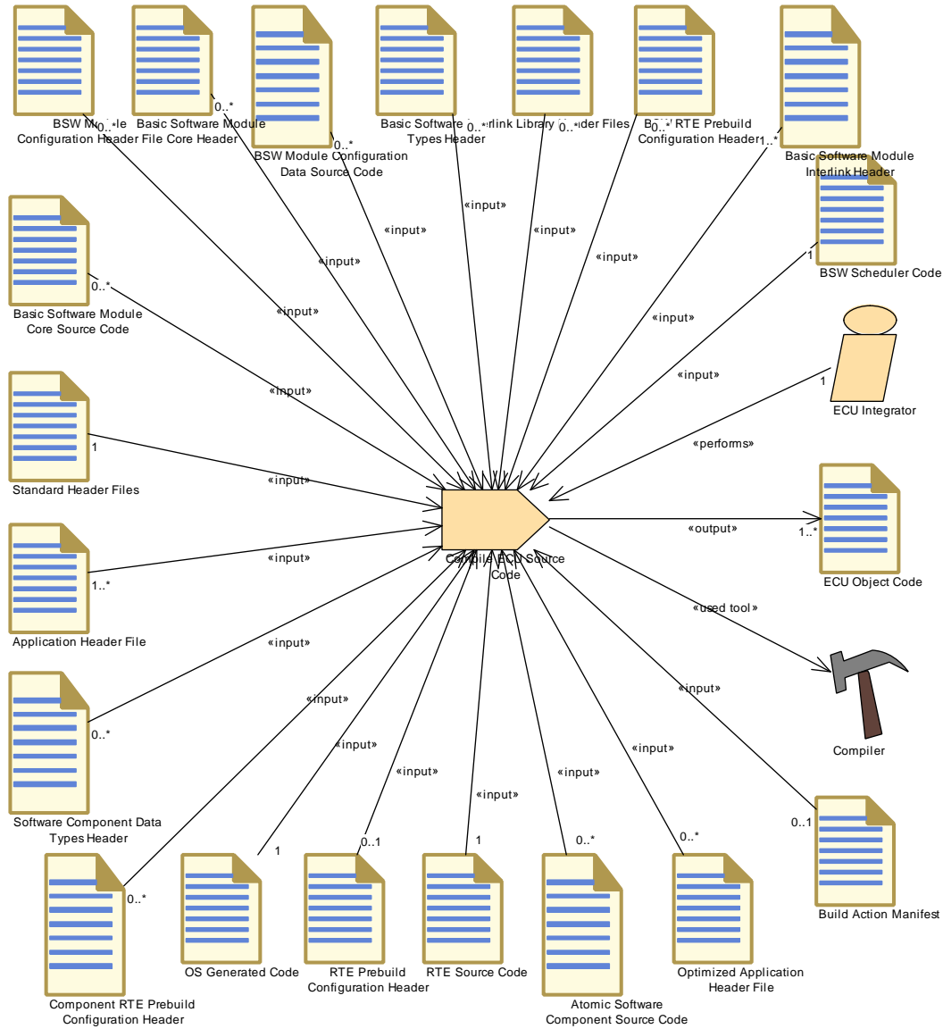
Figure 3.146: Compile ECU Source Code
