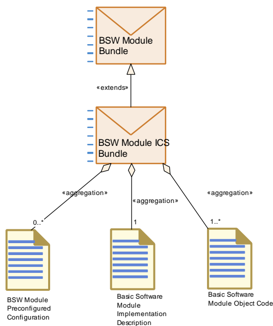
Figure 3.119: BSW Module ICS Bundle
