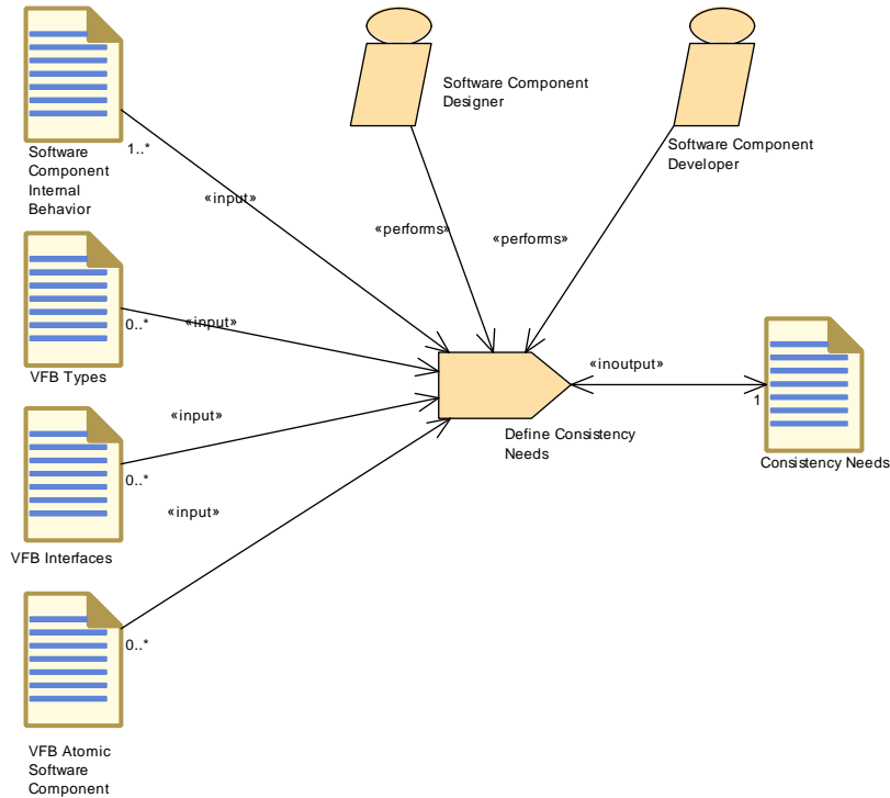
Figure 3.102: Define Consistency Needs
