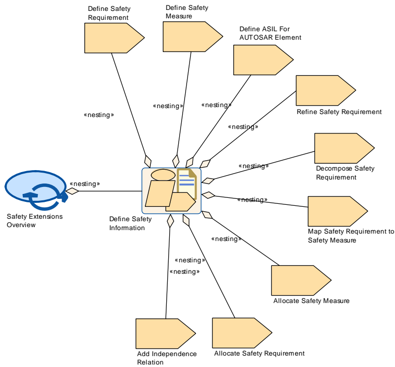
Figure 2.69: Safety Extensions Overview
