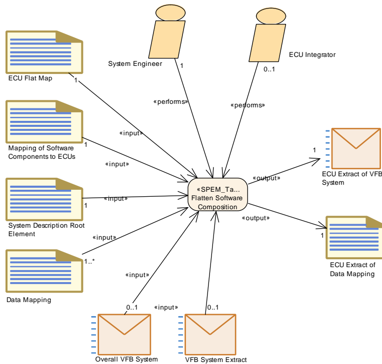
Figure 3.83: Flatten Software Composition
