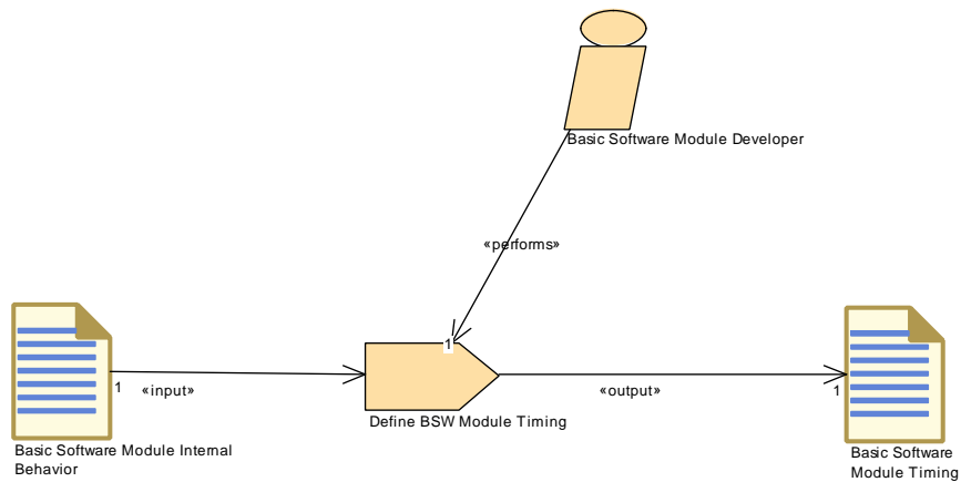
Figure 3.110: Define BSW Module Timing
