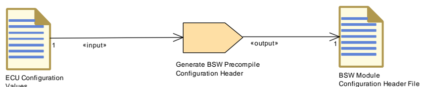
Figure 3.158: Generate BSW Precompile Configuration Header
