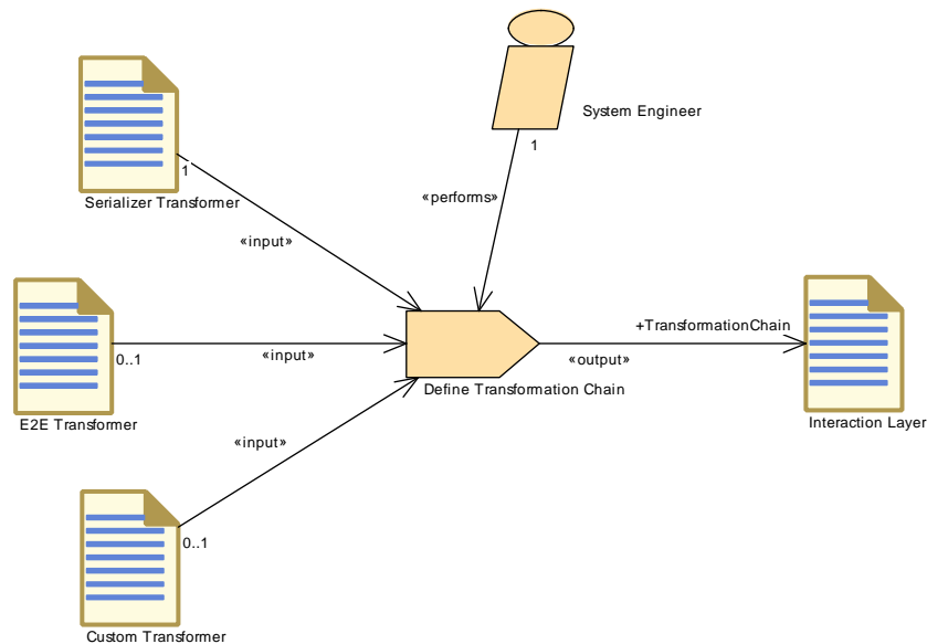
Figure 3.78: Define Transformation Chain
