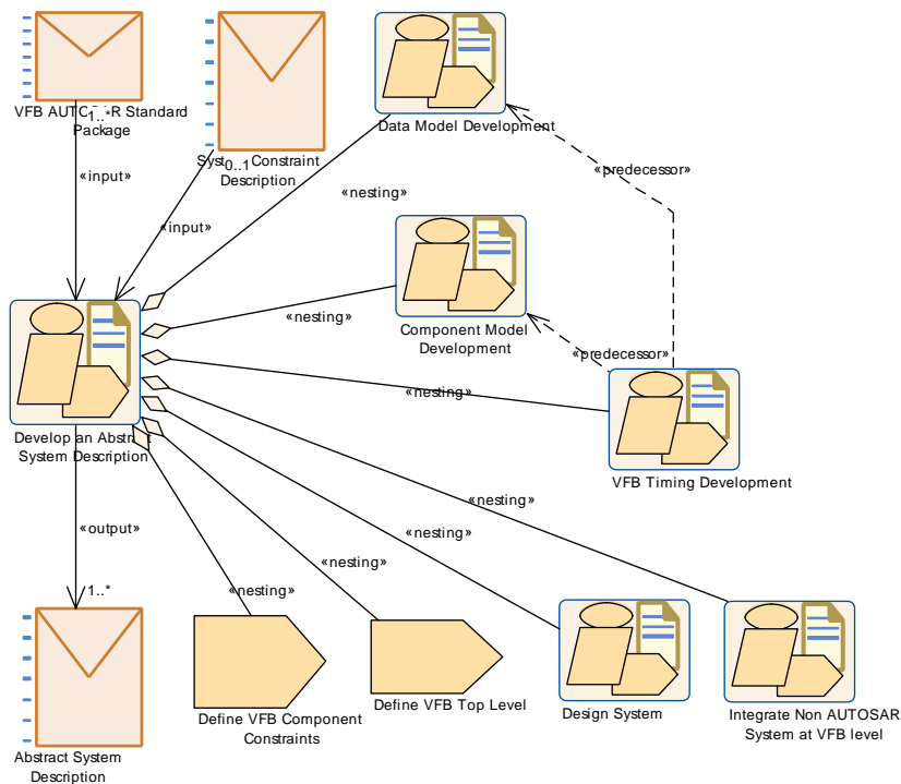
Figure 2.10: Develop an Abstract System Description
