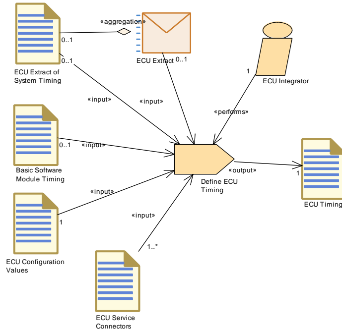
Figure 3.125: Define ECU Timing
