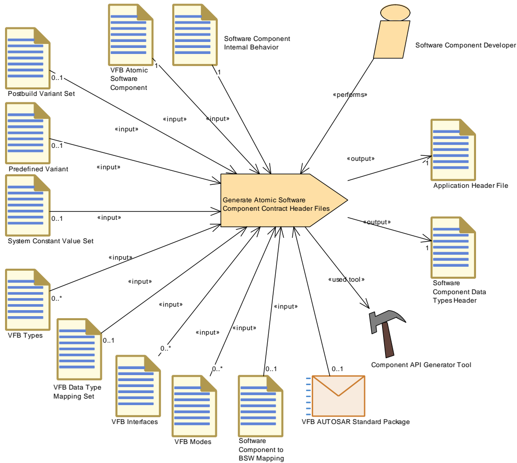
Figure 3.94: Generate Atomic Software Component Contract Header Files
