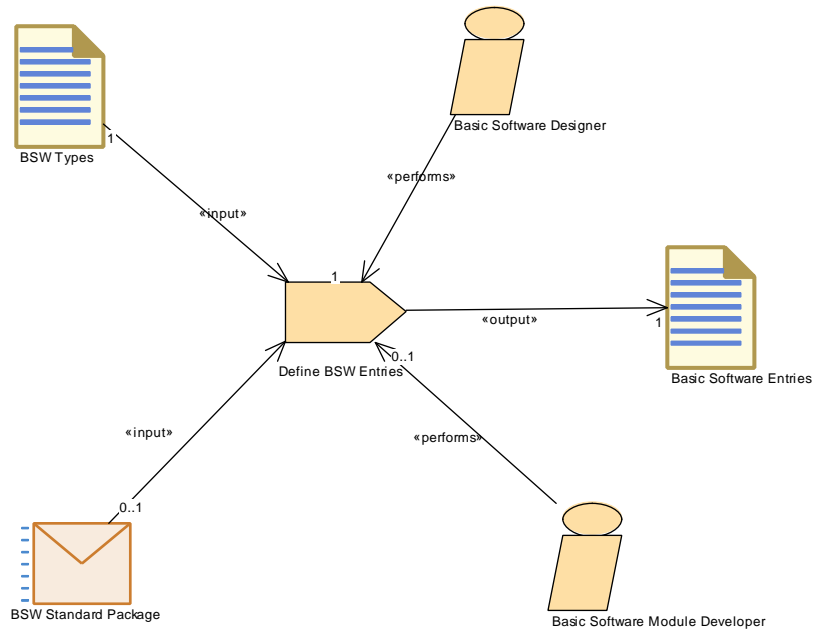
Figure 3.106: Define BSW Entries
