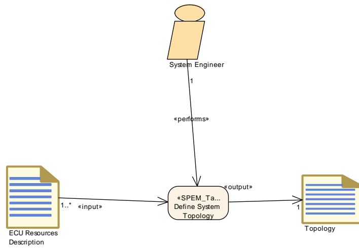
Figure 3.51: Define System Topology
