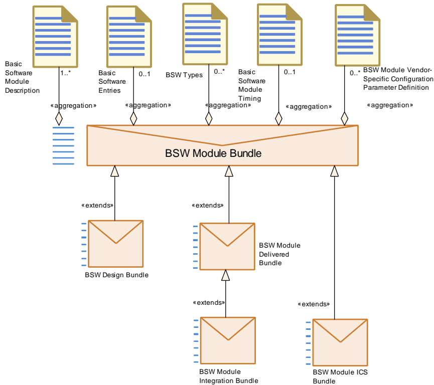
Figure 3.118: BSW Module Bundle
