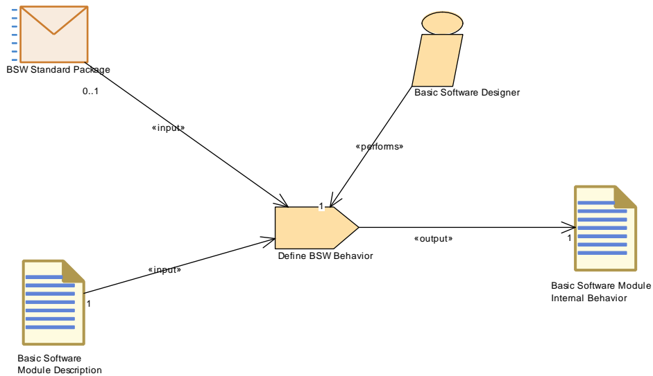
Figure 3.109: Define BSW Behavior
