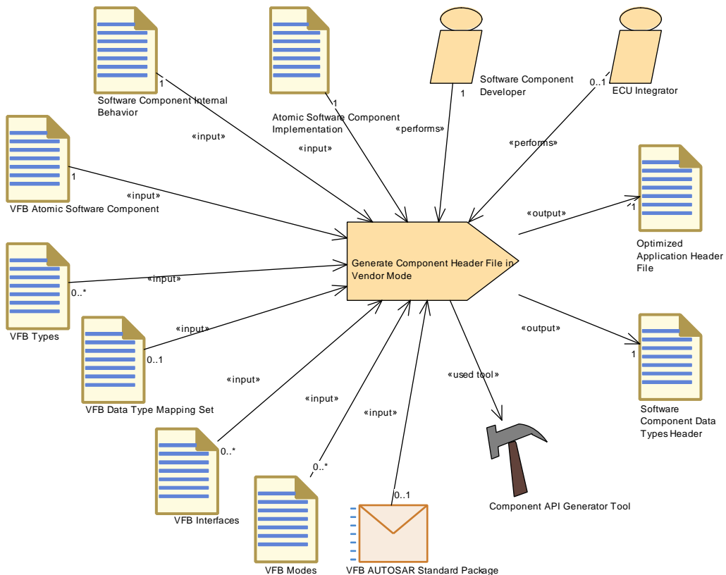
Figure 3.95: Generate Component Header File in Vendor Mode
