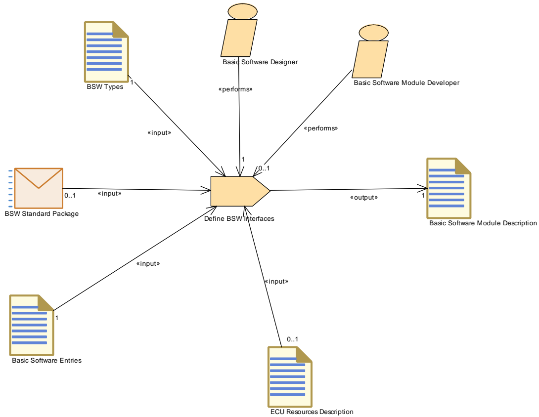
Figure 3.107: Define BSW Interfaces
