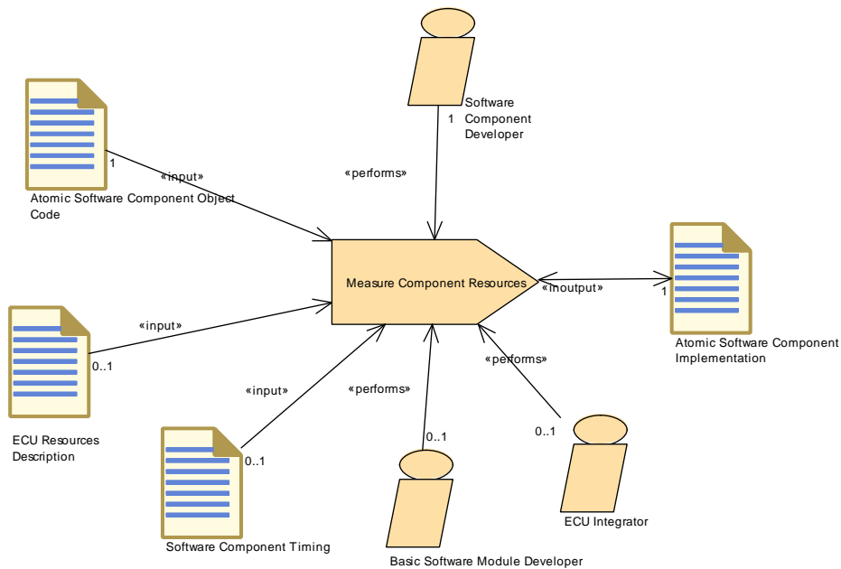
Figure 3.100: Measure Component Resources
