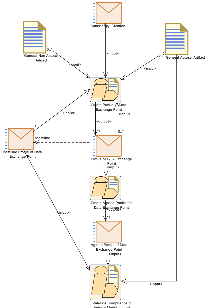
Figure 2.71: Data Exchange Point Workflow
