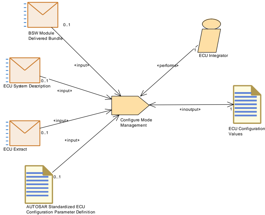
Figure 3.130: Configure Mode Management
