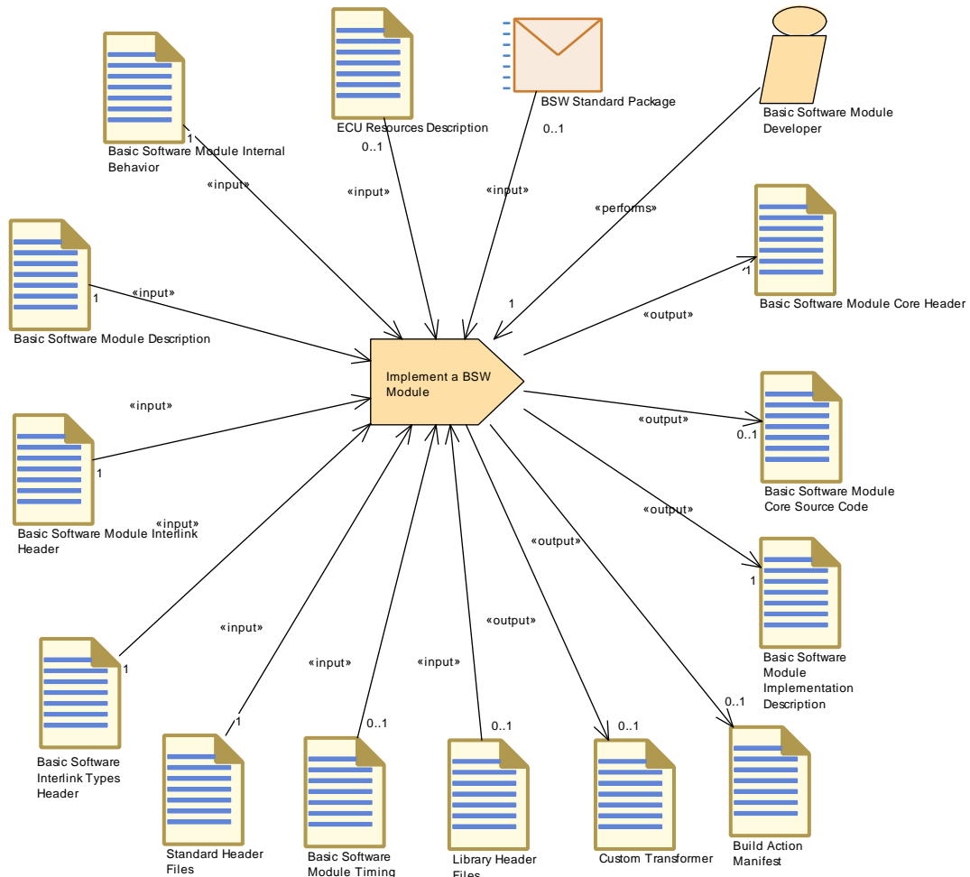
Figure 3.112: Implement a BSW Module
