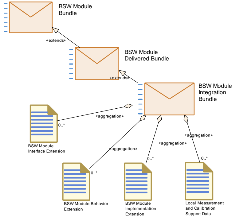
Figure 3.152: BSW Module Integration Bundle
