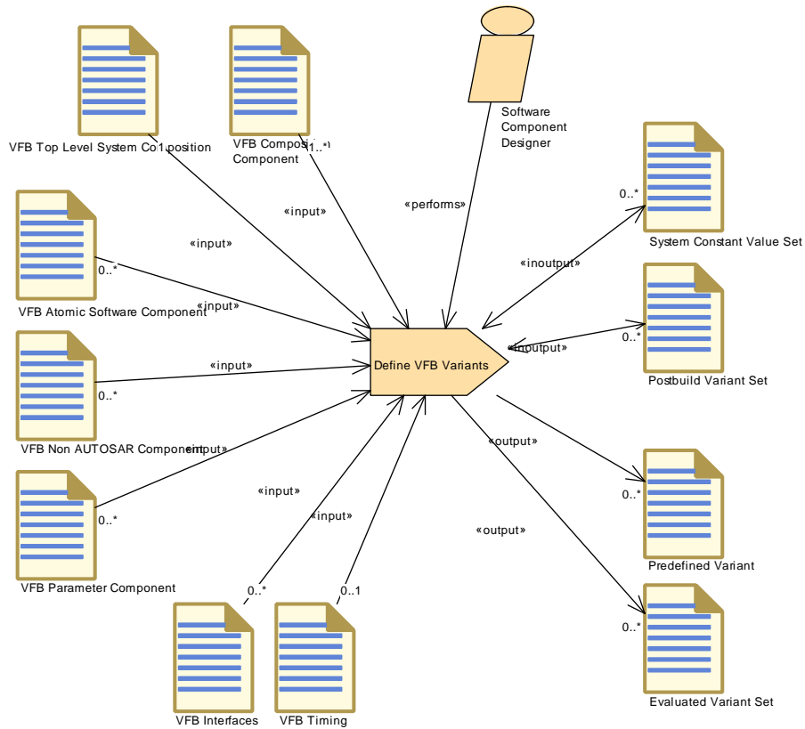
Figure 3.40: Task Define VFB Variants
