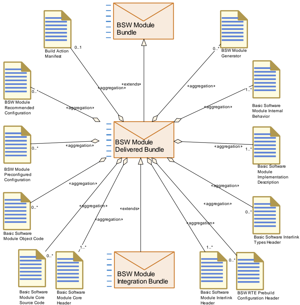
Figure 3.120: BSW Module Delivered Bundle
