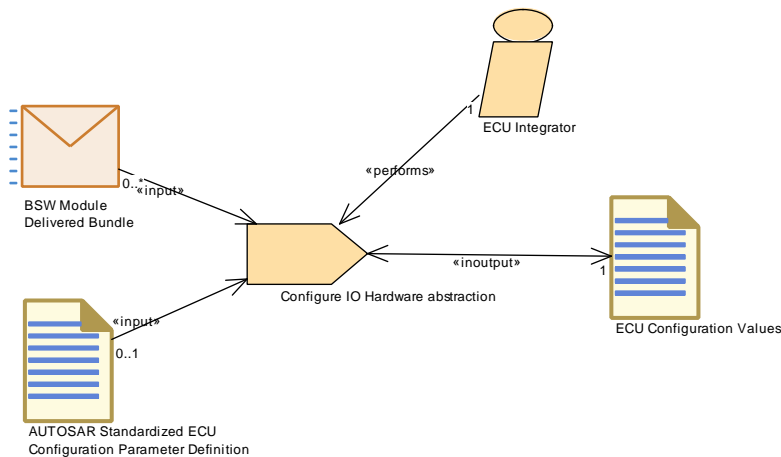
Figure 3.136: Configure IO Hardware Abstraction
