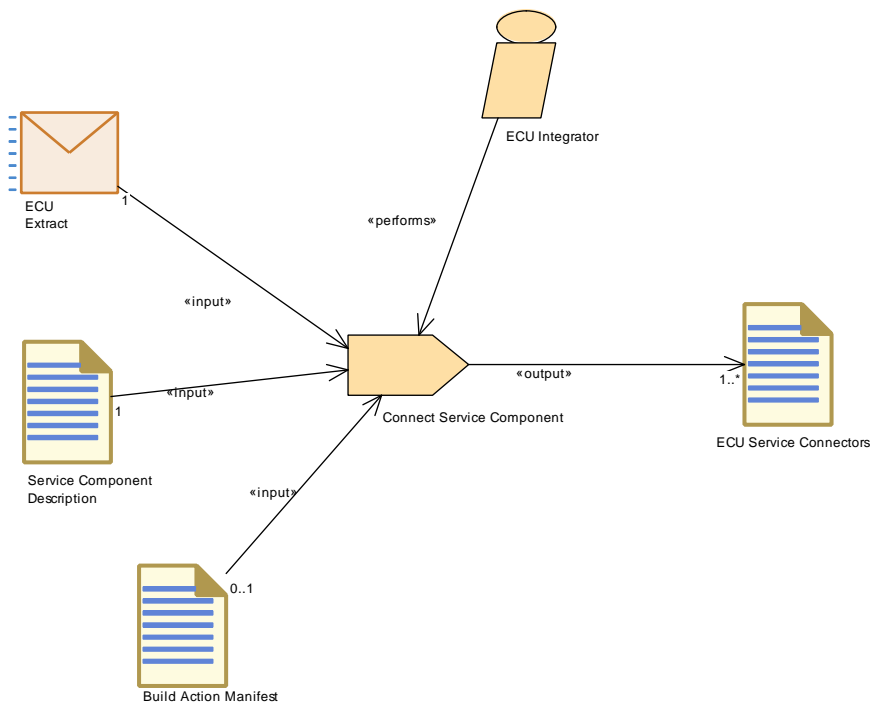
Figure 3.134: Connect Service Component
