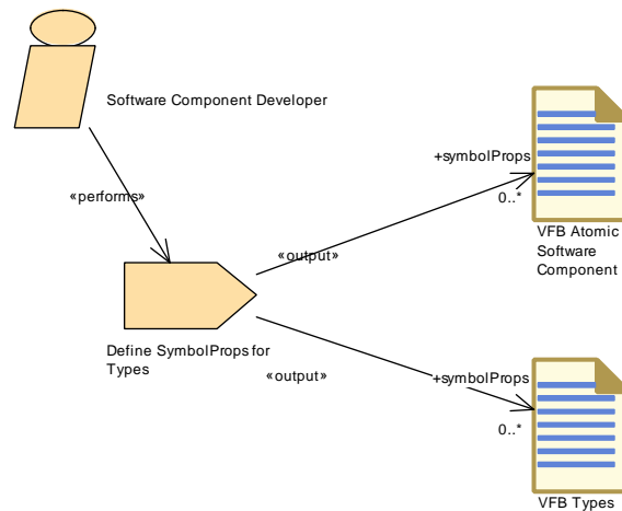
Figure 3.92: Define SymbolProps for Types
