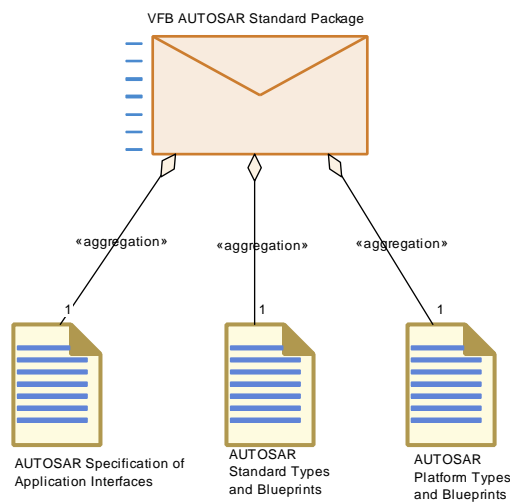
Figure 3.45: Structure of Deliverable VFB AUTOSAR Standard Package
