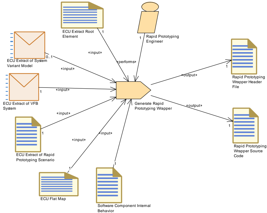
Figure 3.103: Generate Rapid Prototyping Wrapper
