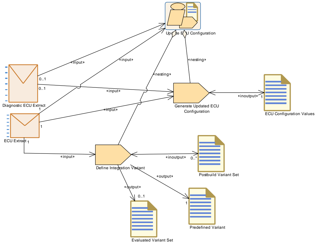
Figure 2.45: Update ECU Configuration
