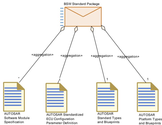
Figure 3.117: BSW Standard Package
