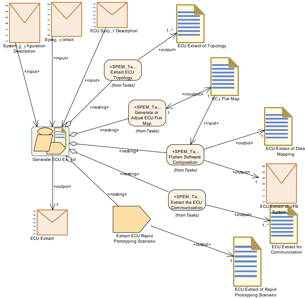
Figure 2.33: Generate the ECU Extract
