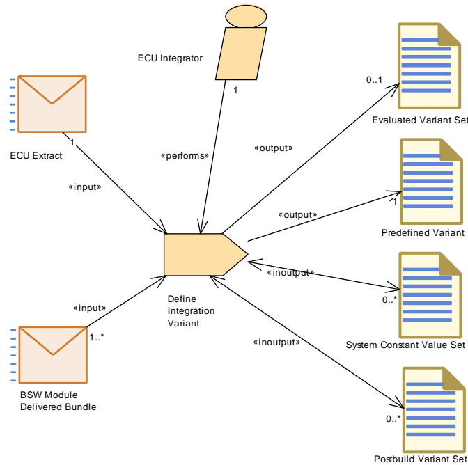
Figure 3.122: Define Integration Variant
