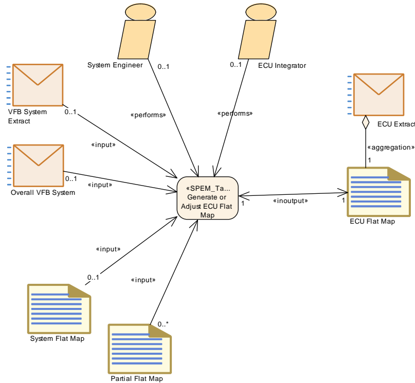
Figure 3.82: Generate or Adjust ECU Flat Map
