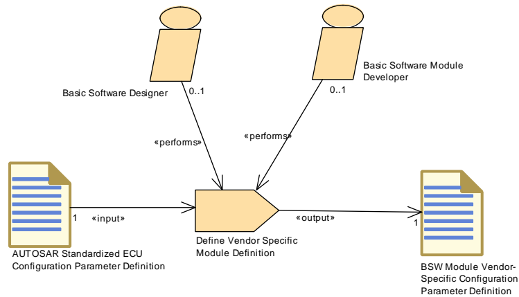
Figure 3.108: Define Vendor Specific Module Definition
