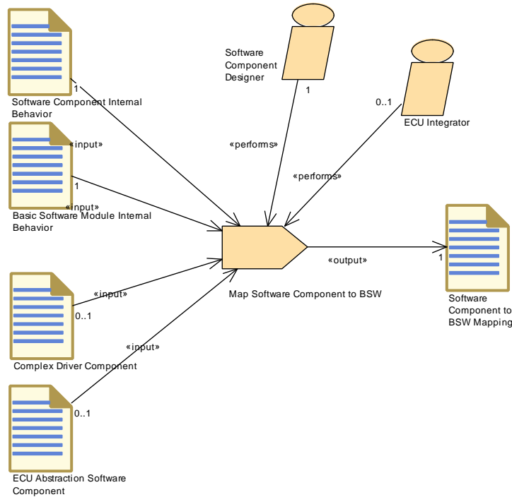
Figure 3.99: Map Software Component to BSW
