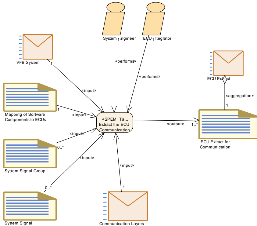
Figure 3.84: Extract the ECU Communication
