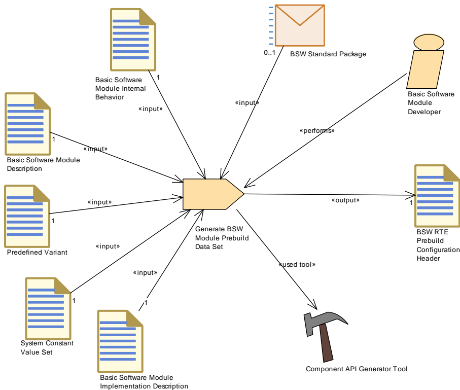
Figure 3.116: Generate BSW Module Prebuild Dataset
