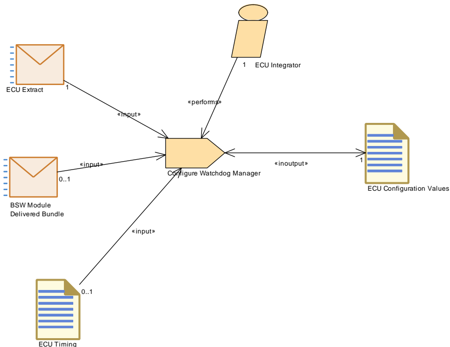
Figure 3.129: Configure Watchdog Manager
