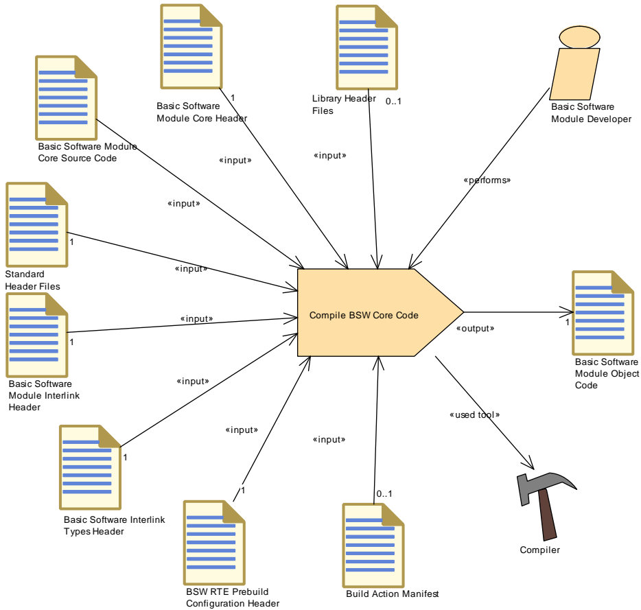
Figure 3.115: Compile BSW Core Code
