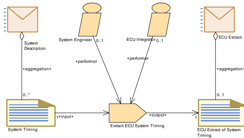
Figure 3.85: Extract the ECU System Timing Model
