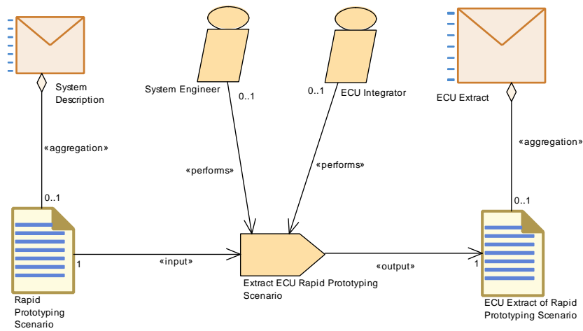
Figure 3.87: Extract ECU Rapid Prototyping Scenario
