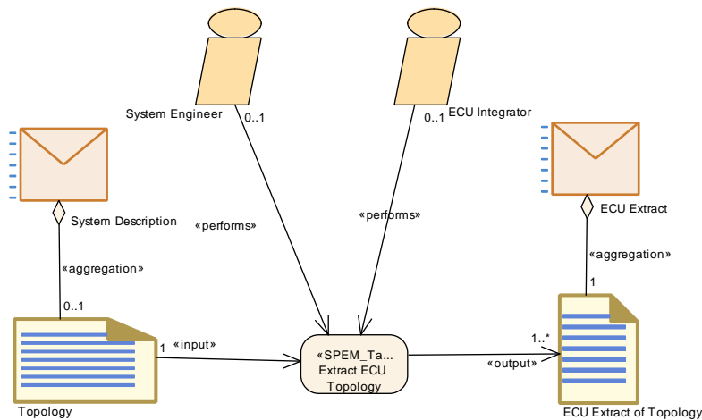
Figure 3.81: Extract ECU Topology
