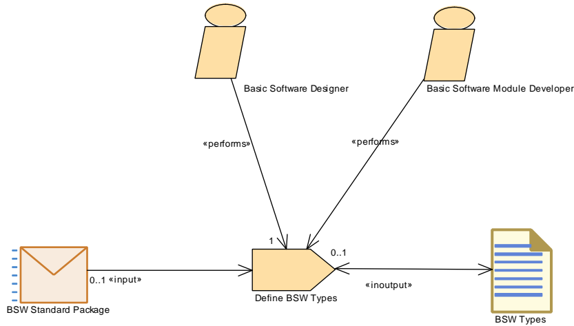
Figure 3.105: Define BSW Types
