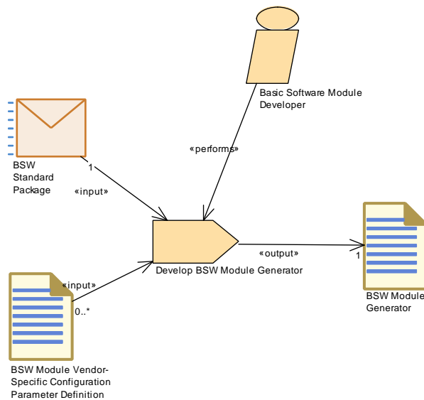
Figure 3.113: Develop BSW Module Generator
