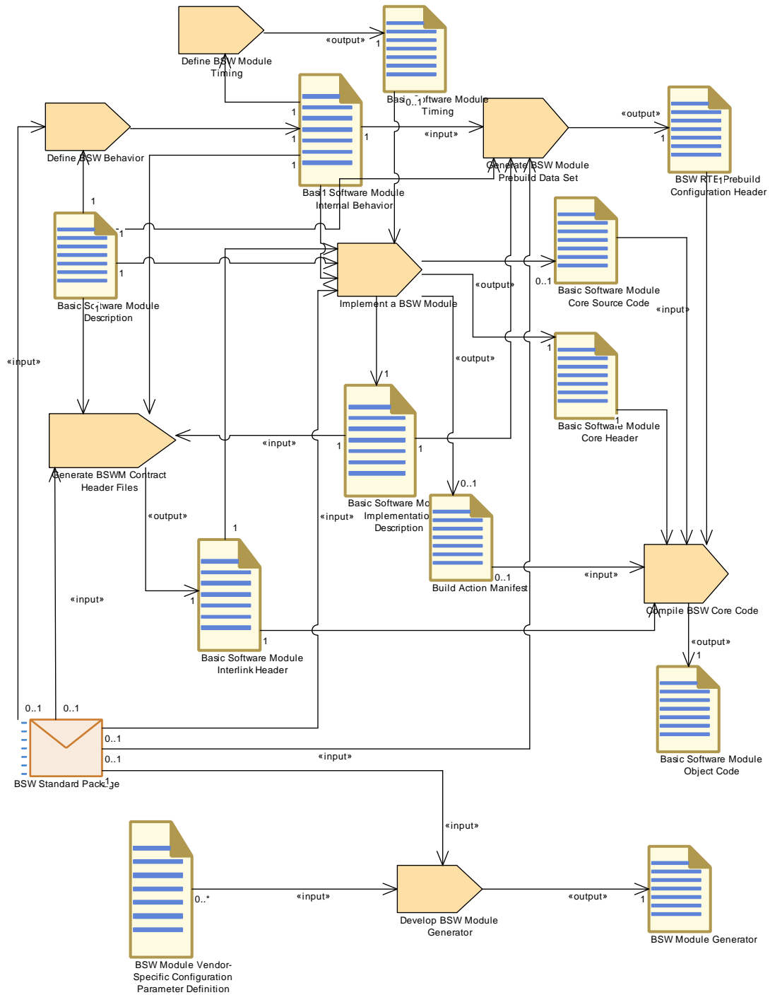
Figure 2.40: Develop Basic Software Module
