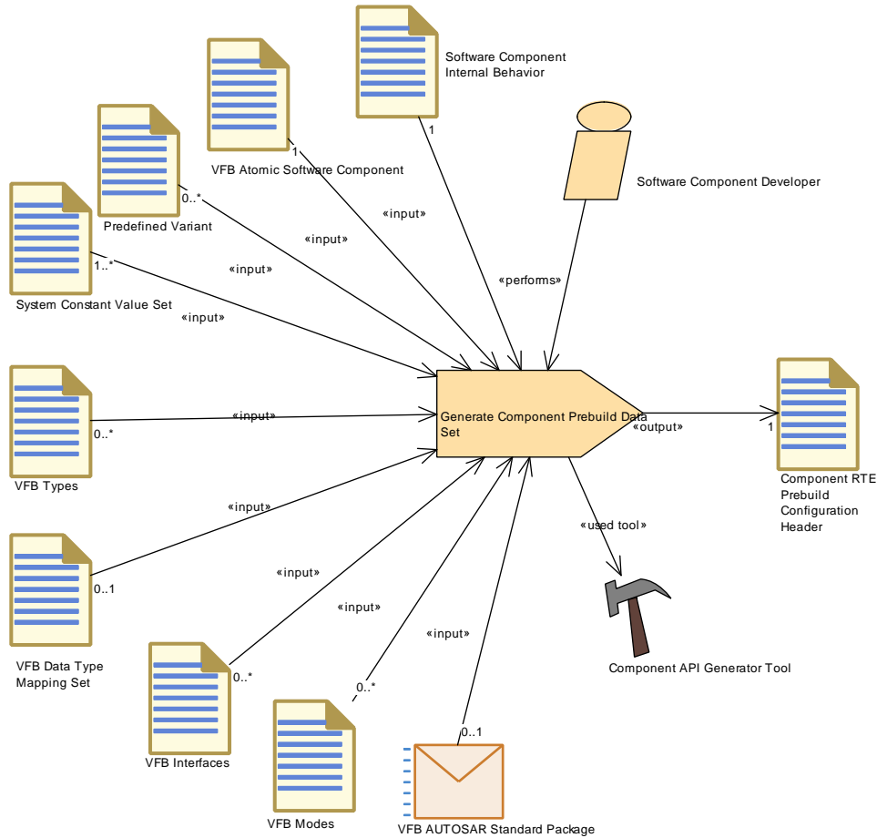
Figure 3.96: Generate Component Prebuild Data Set
