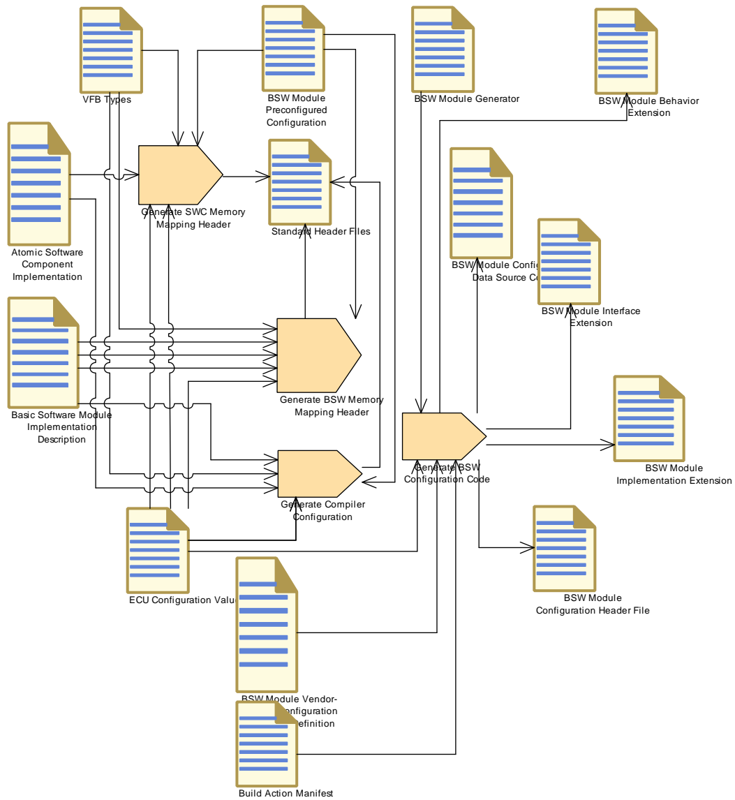
Figure 2.48: Generate BSW and RTE (Part 1)
