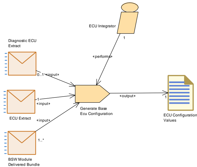
Figure 3.123: Generate Base ECU Configuration
