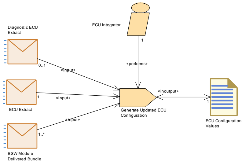
Figure 3.124: Generate Updated ECU Configuration
