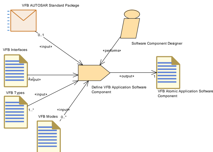
Figure 3.28: Task Define VFB Application Software Component
