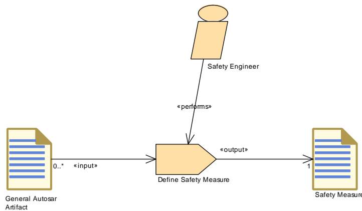
Figure 3.14: Define Safety Measure
