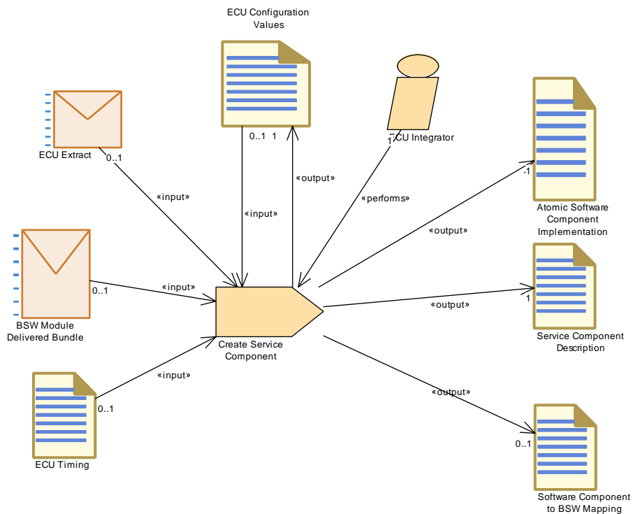
Figure 3.133: Create Service Component
