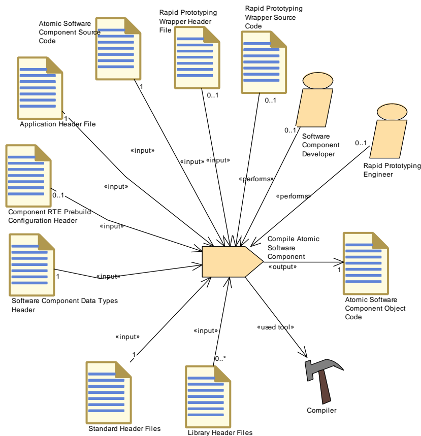
Figure 3.98: Compile Atomic Software Component
