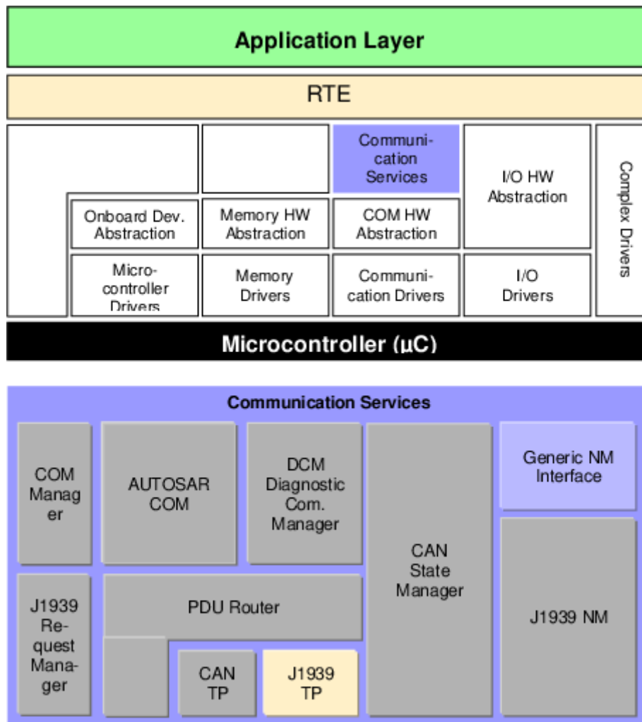
Figure 5.1: Position of the J1939Tp in the AUTOSAR architecture
