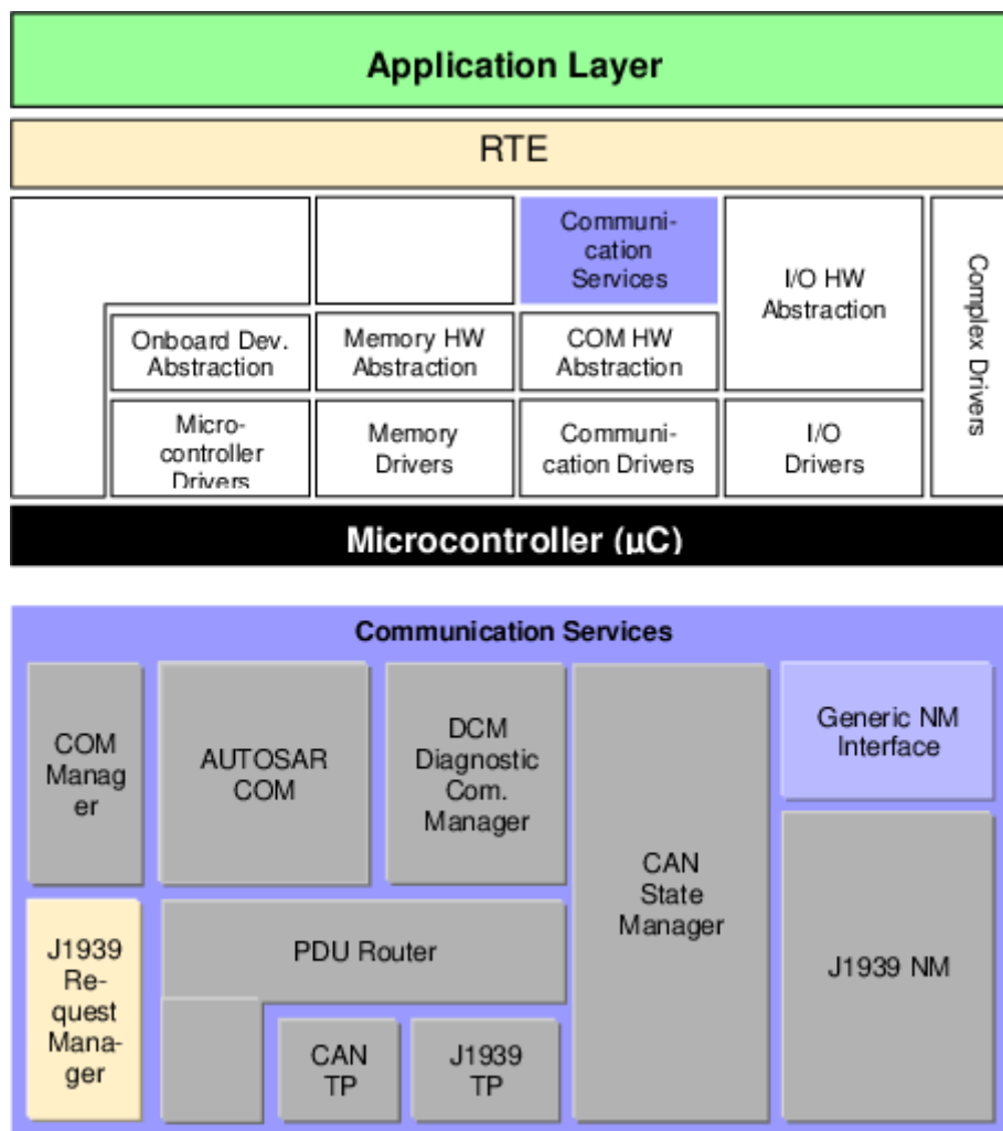
Figure 6.1: Position of the J1939Rm in the AUTOSAR architecture
