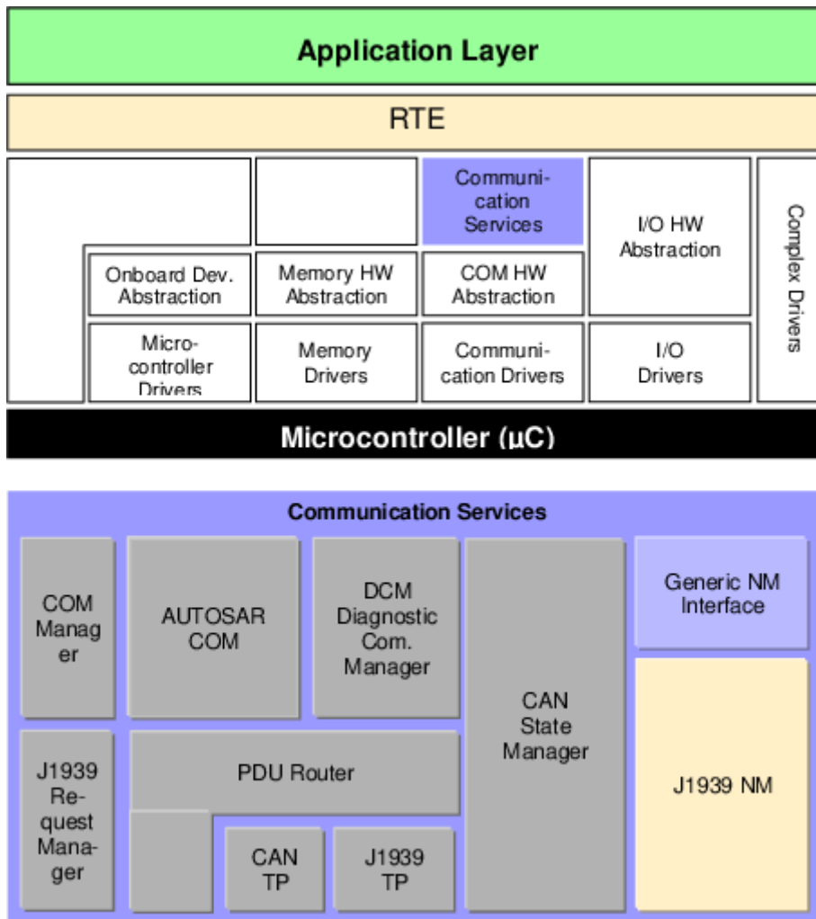
Figure 7.1: Position of the J1939Nm in the AUTOSAR architecture
