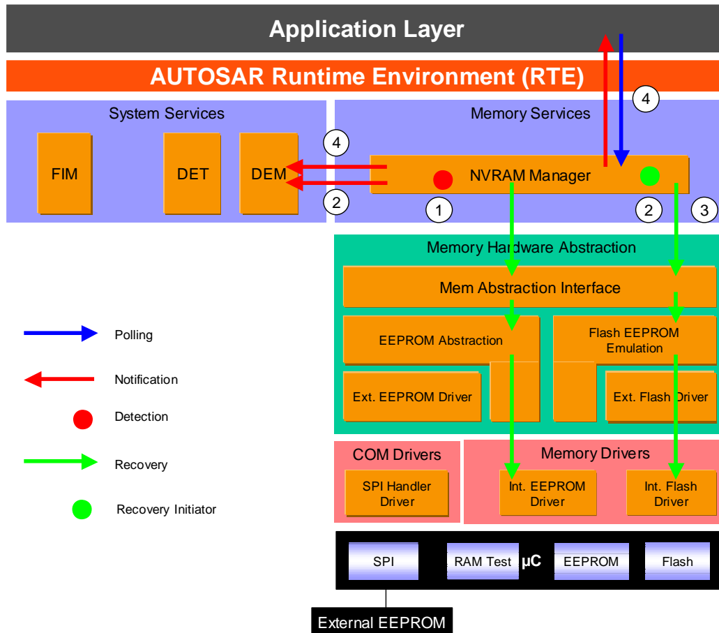
Figure 28: Information path for the Static Block check error
