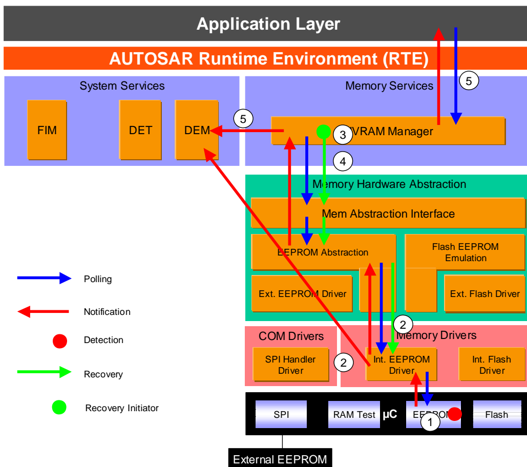
Figure 21: Information path for the EEPROM erase job error (for internal EEPROM)
