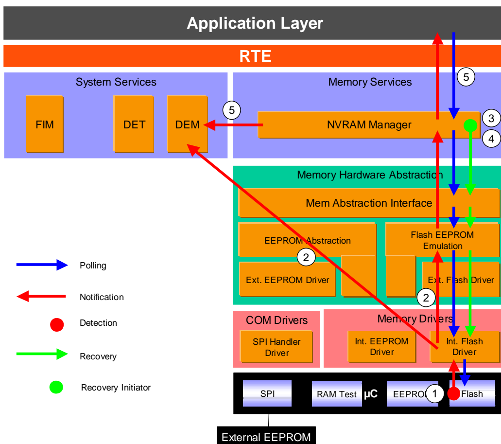
Figure 17: Information path for the flash read job error (internal flash)
