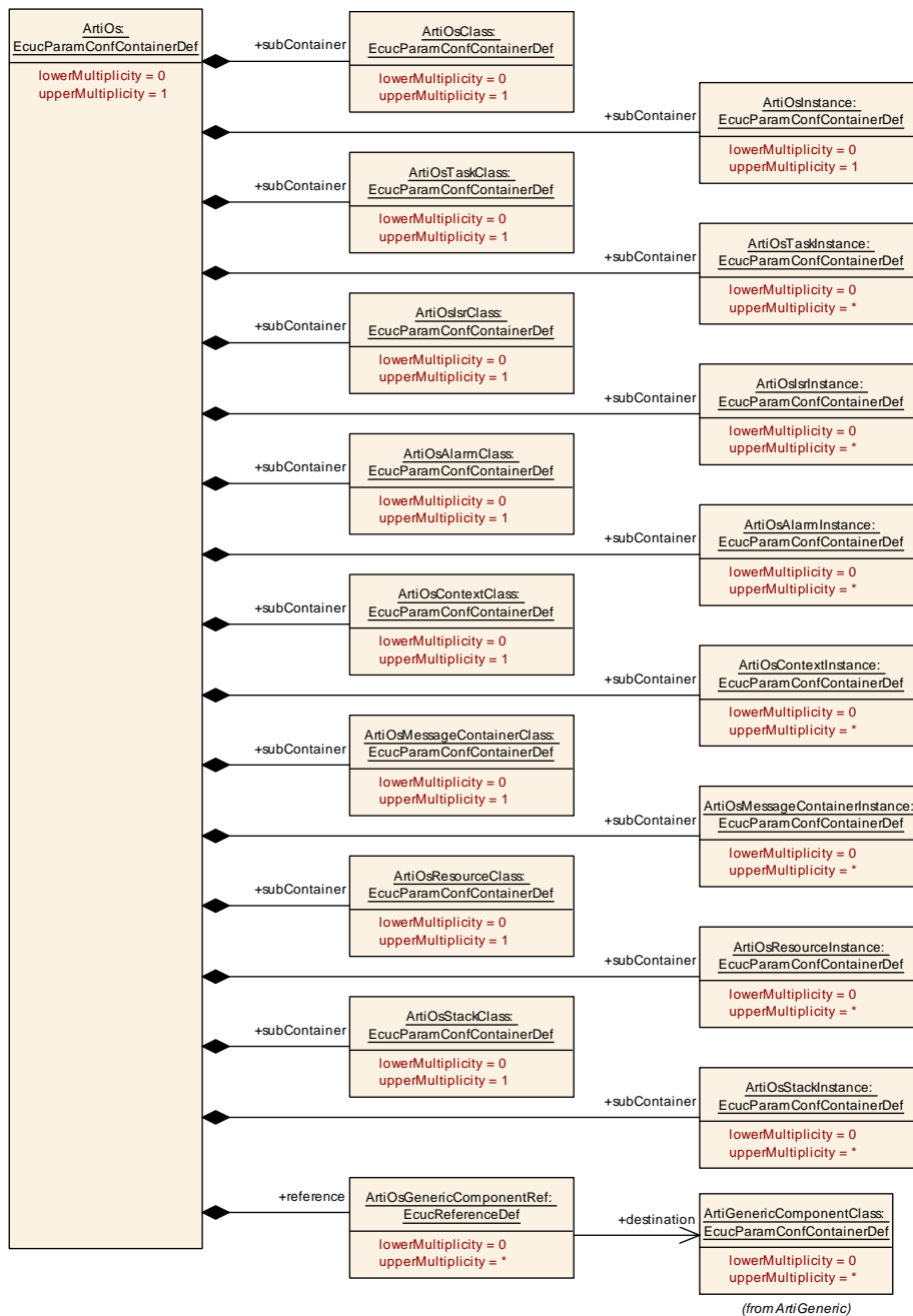
Figure 3.4: ArtiOs Ecuc Module Definition Class Diagram
