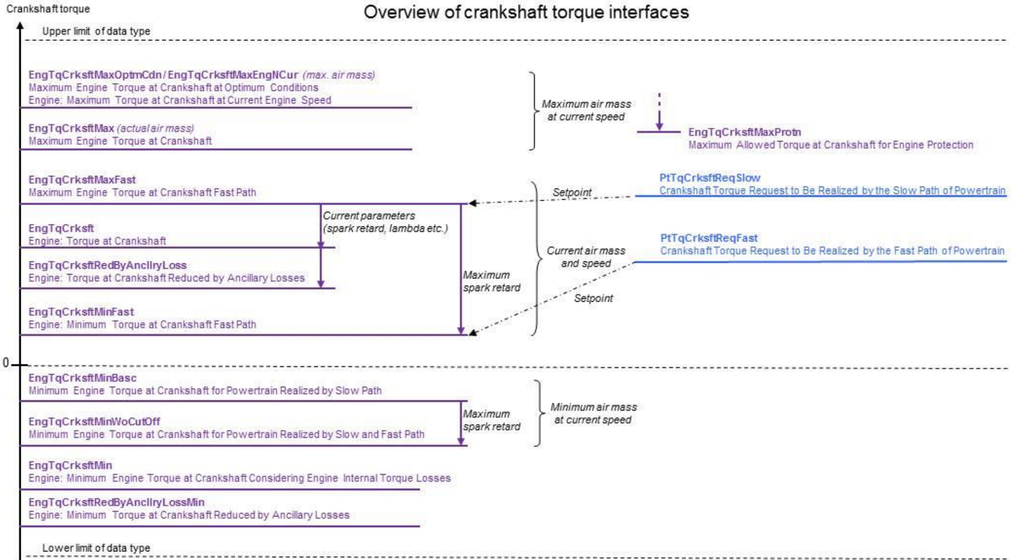
Overview of crankshaft torque interfaces
